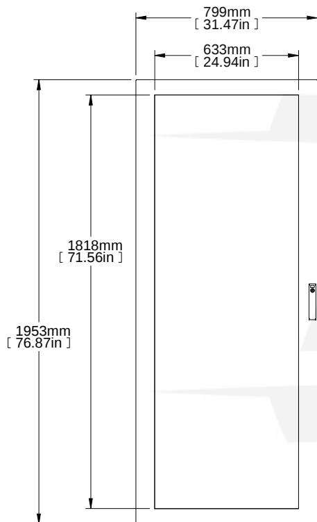
FRONT VIEW
