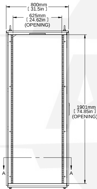
L.S. VIEW
