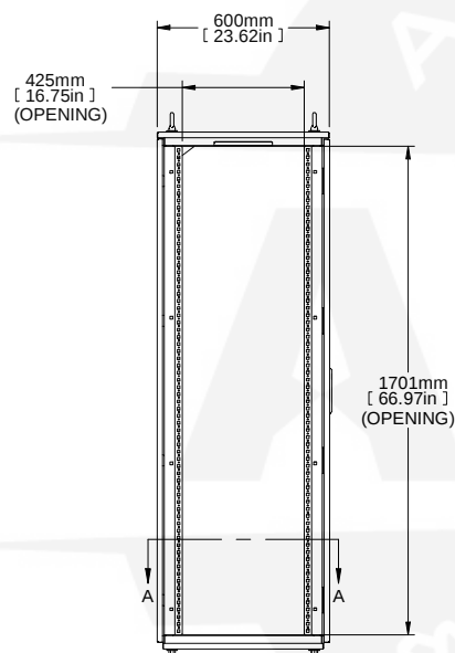
L.S. VIEW
