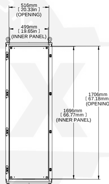
FRONT VIEW DOOR REMOVED
