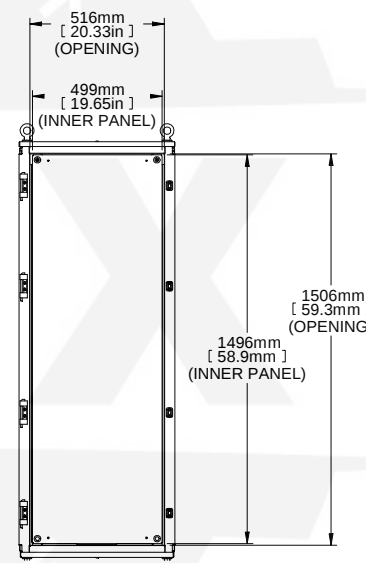
FRONT VIEW DOOR REMOVED
