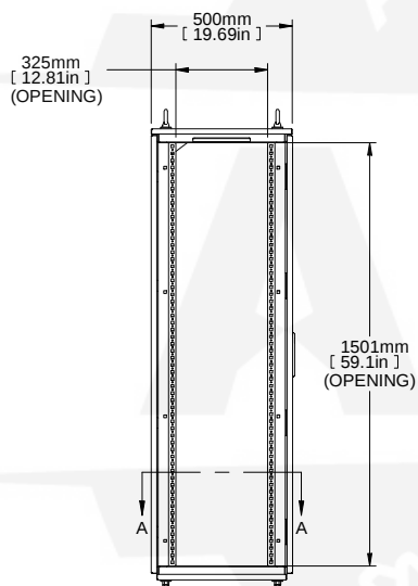
L.S. VIEW
