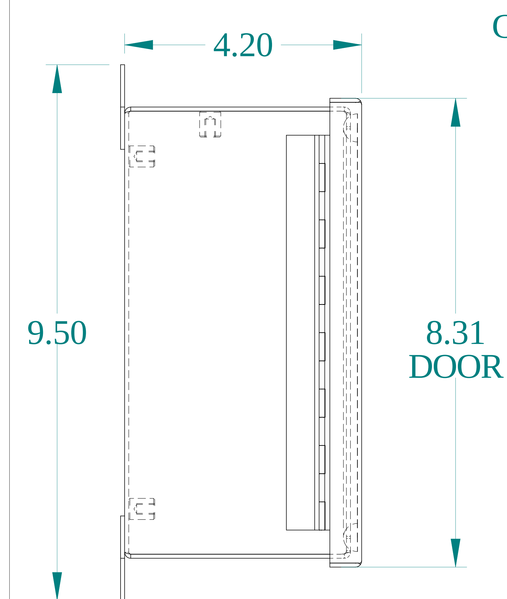
SIDE VIEW
