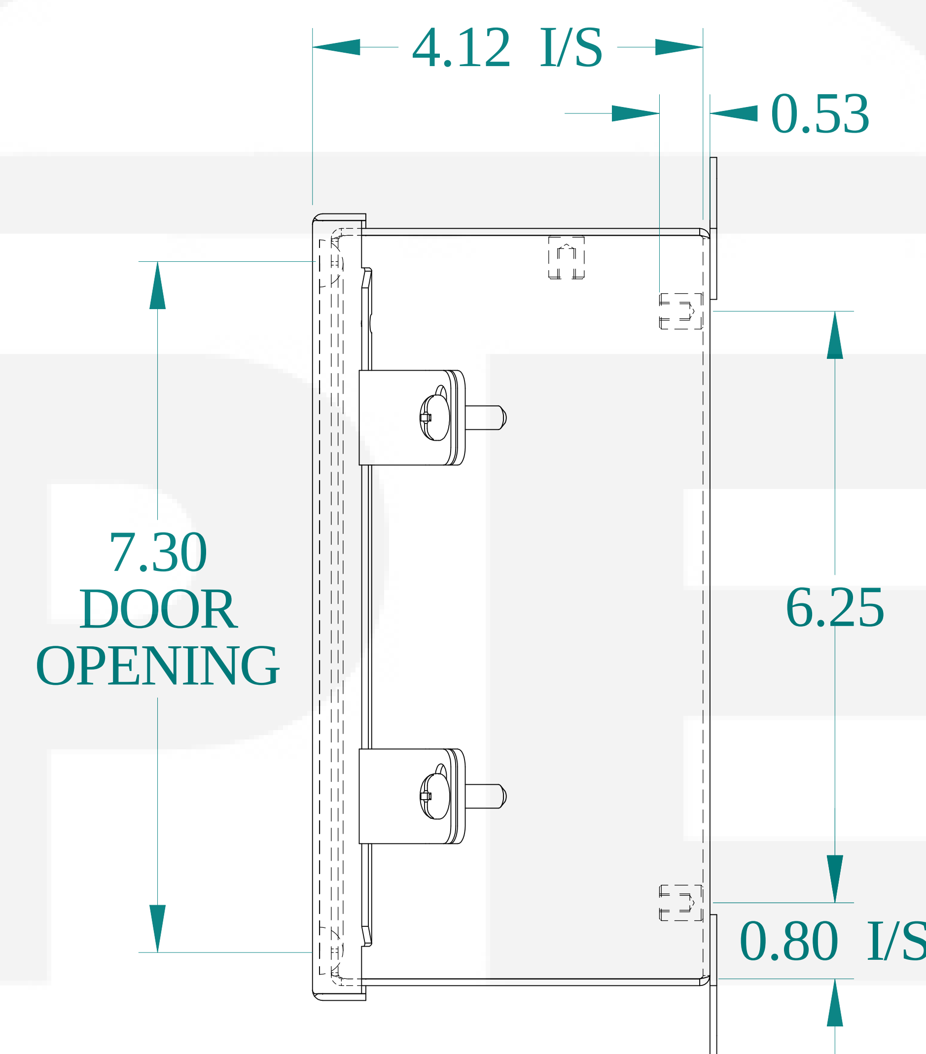
SIDE VIEW
