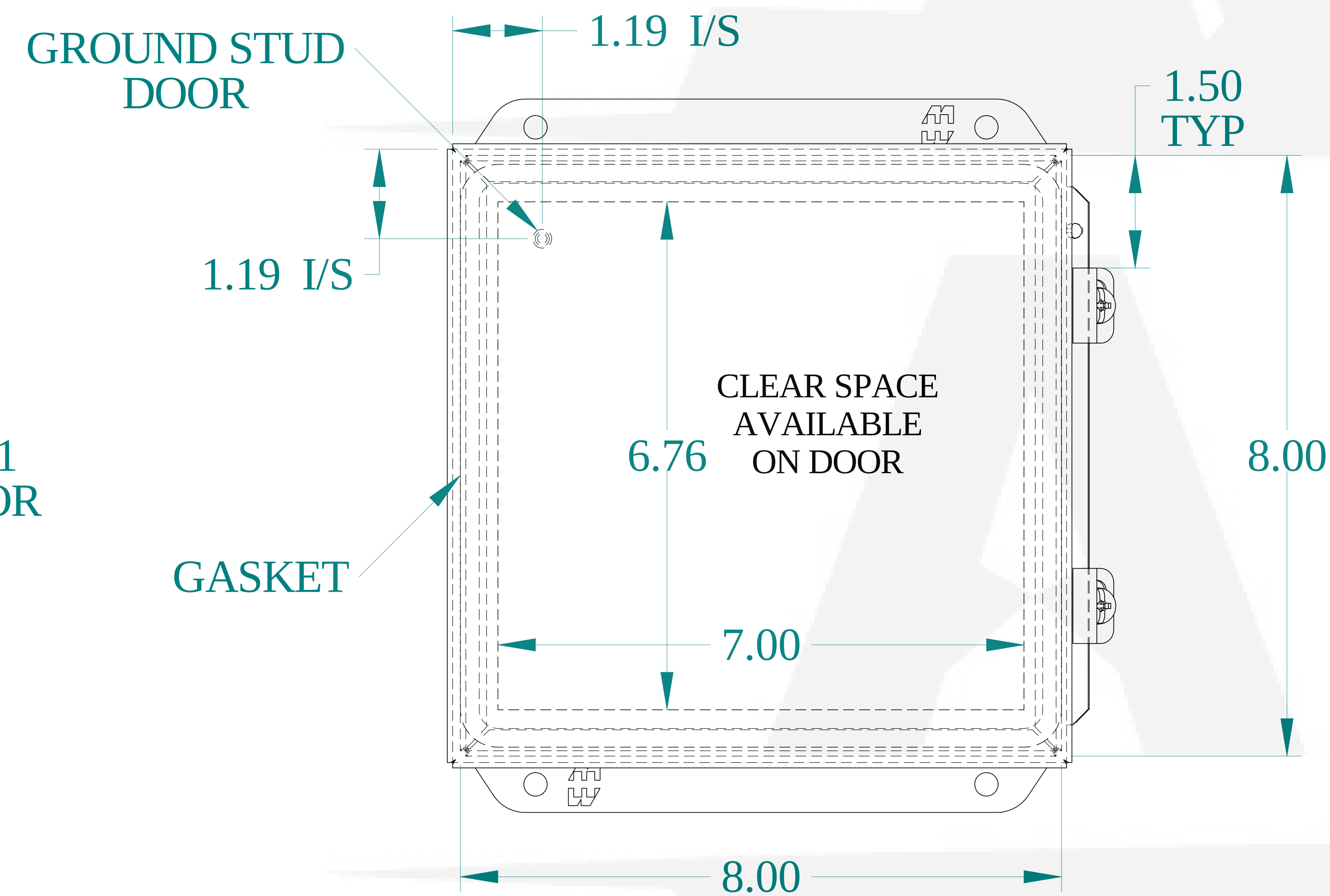
FRONT VIEW
