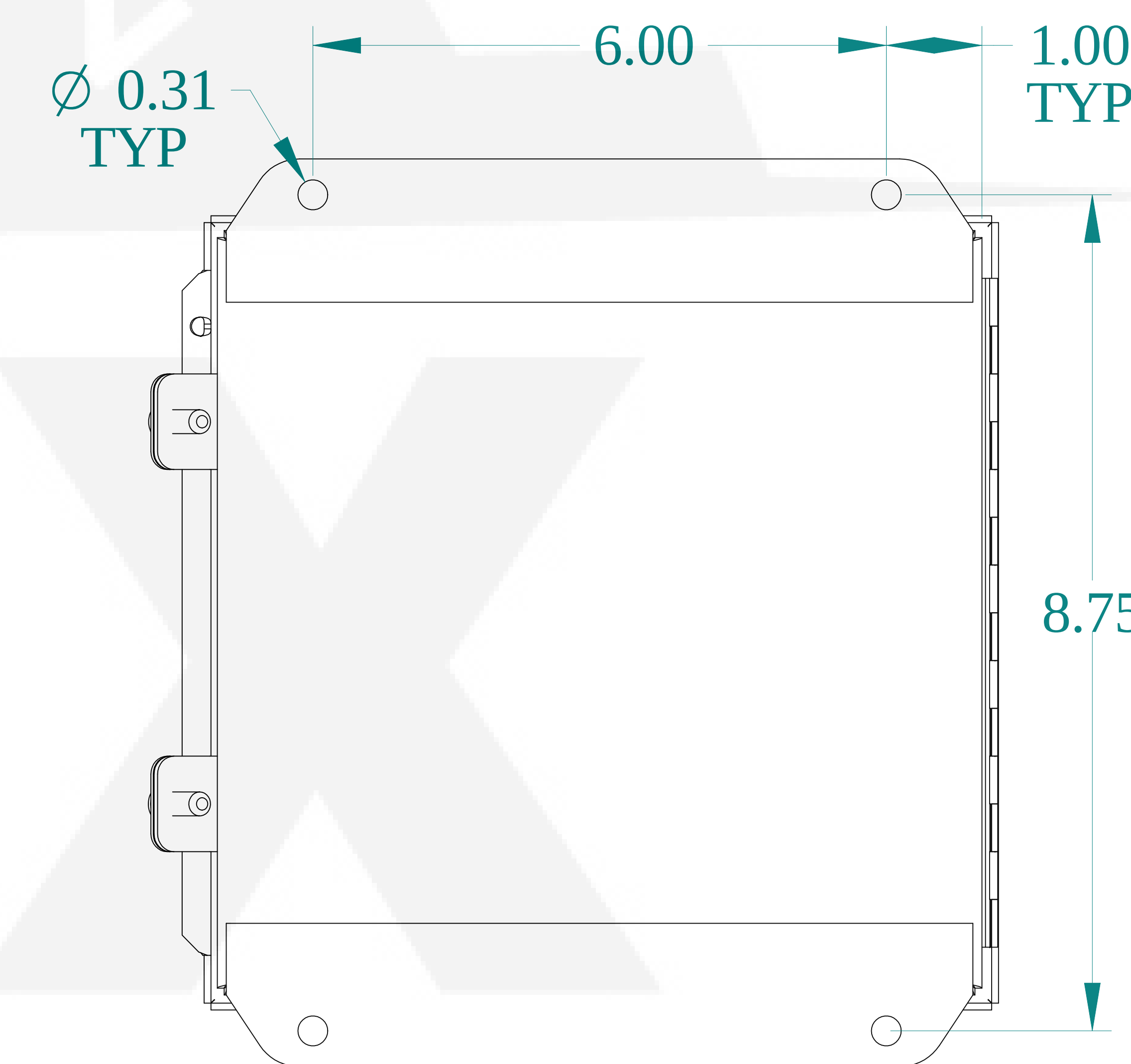
BACK VIEW
