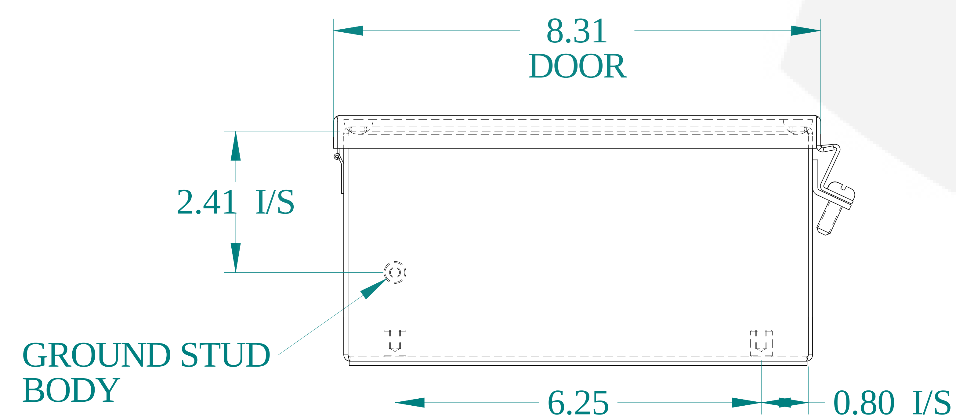
BOTTOM VIEW
