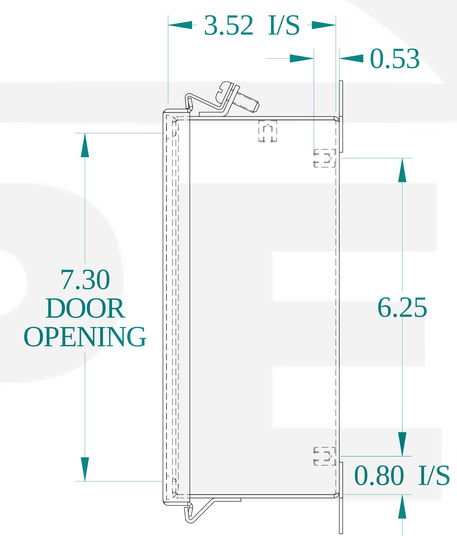
SIDE VIEW
