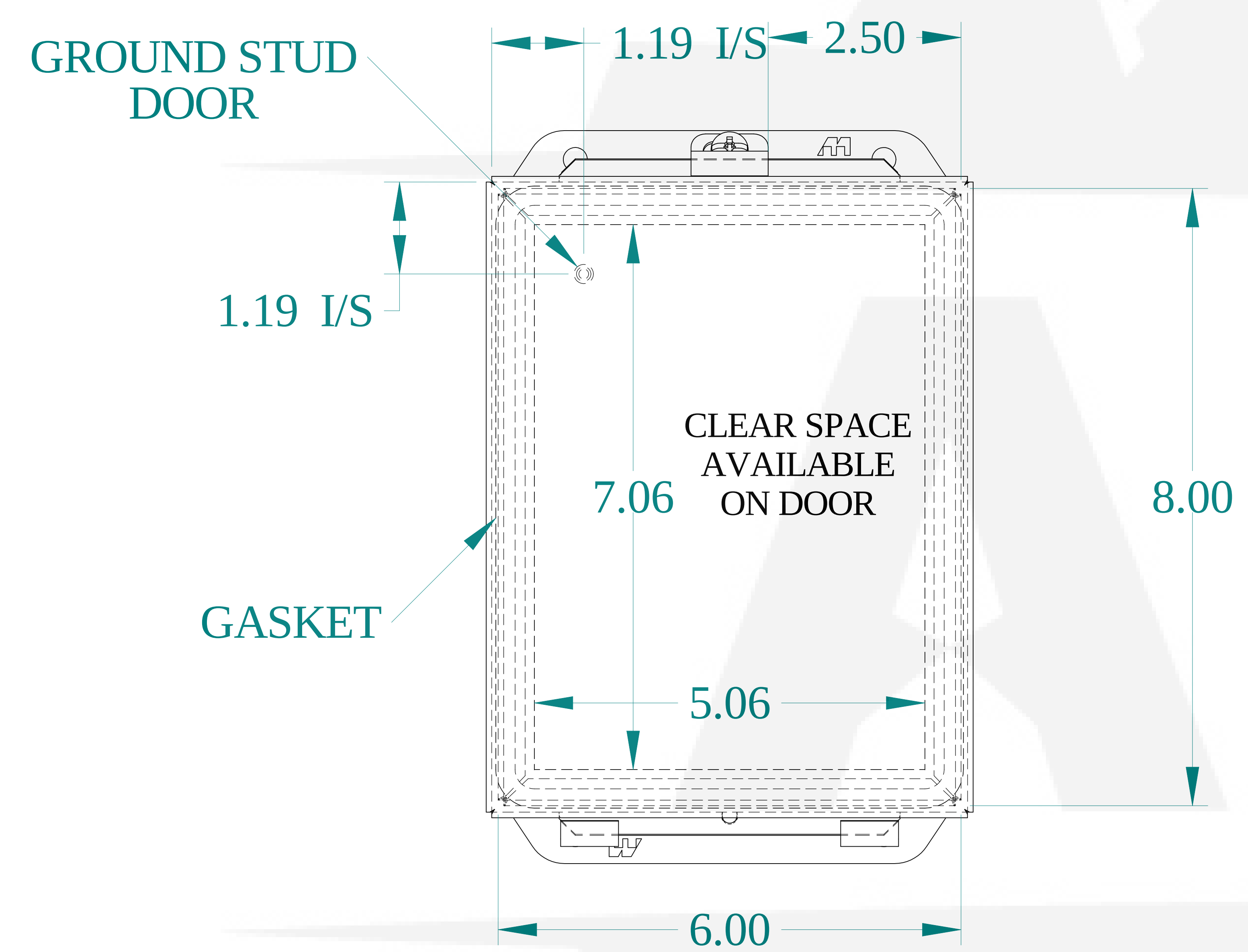
FRONT VIEW
