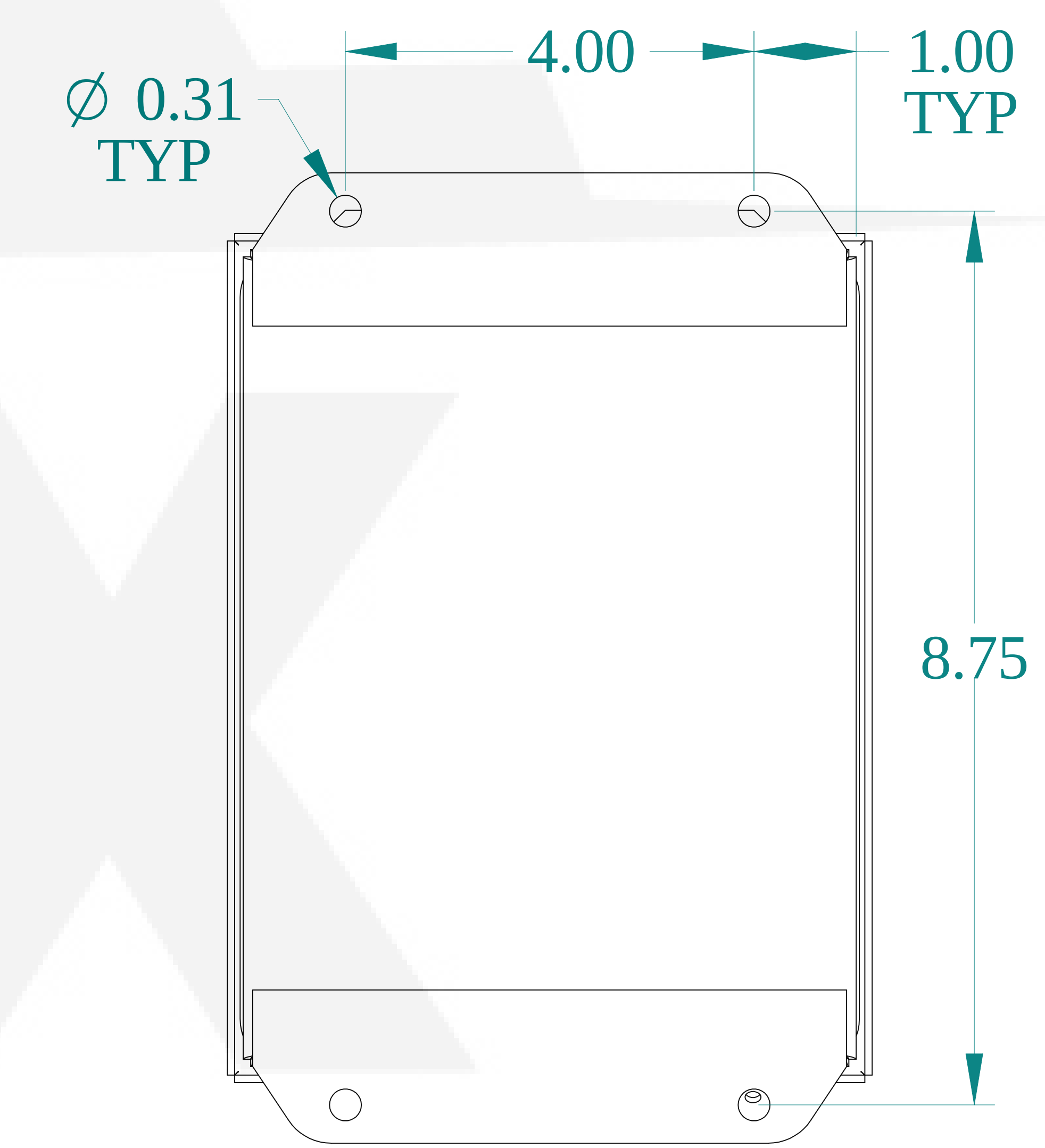
BACK VIEW
