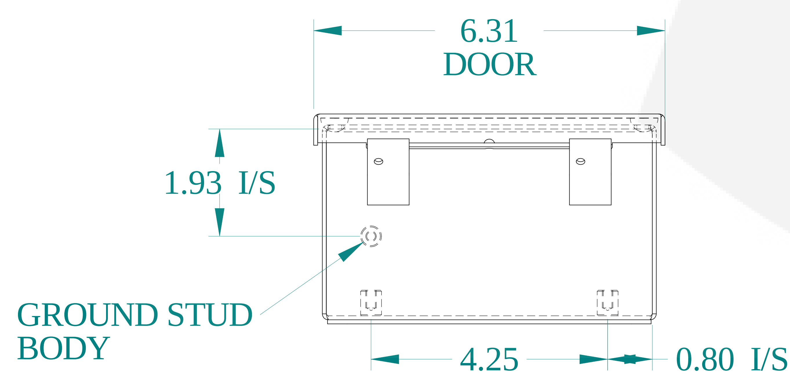
BOTTOM VIEW
