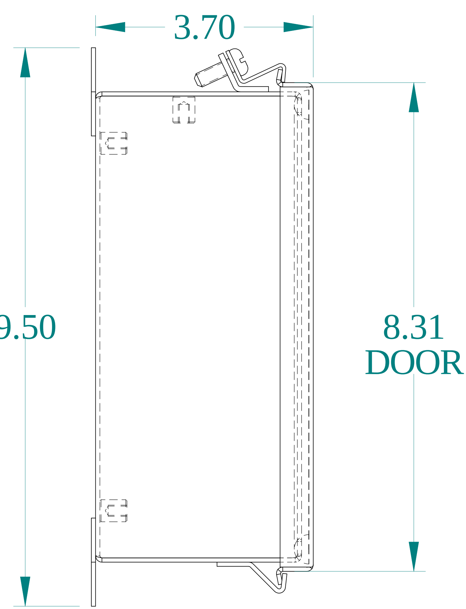
SIDE VIEW
