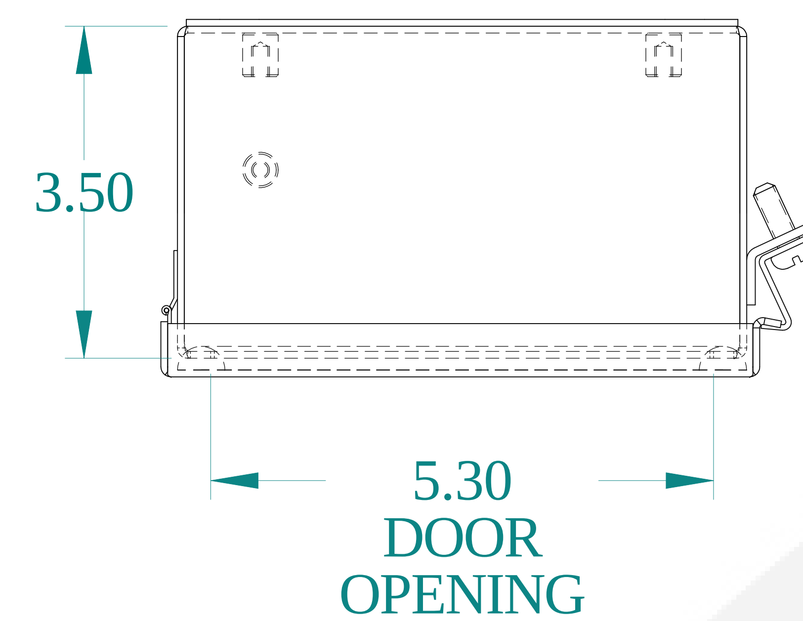
TOP VIEW
