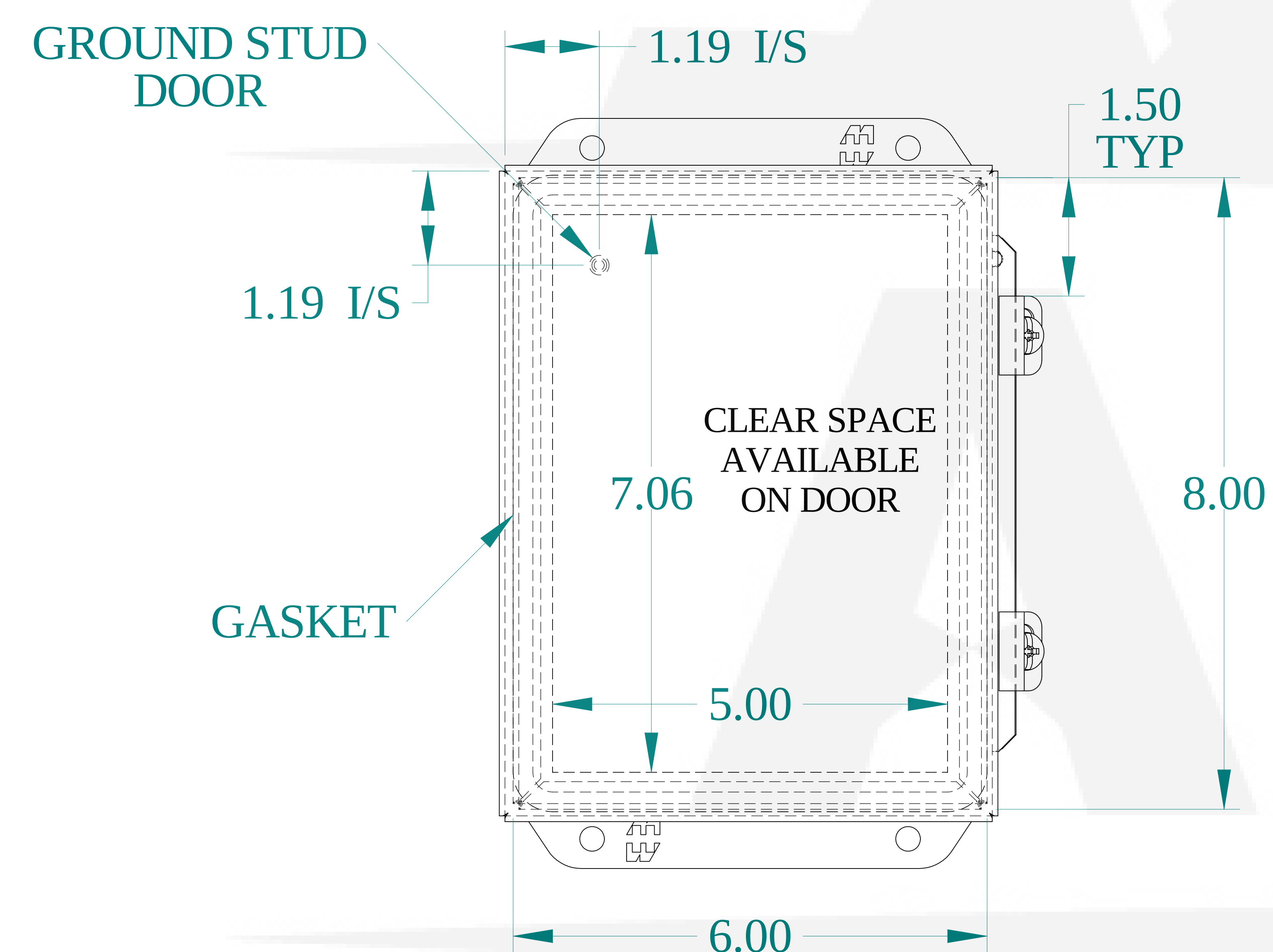
FRONT VIEW
