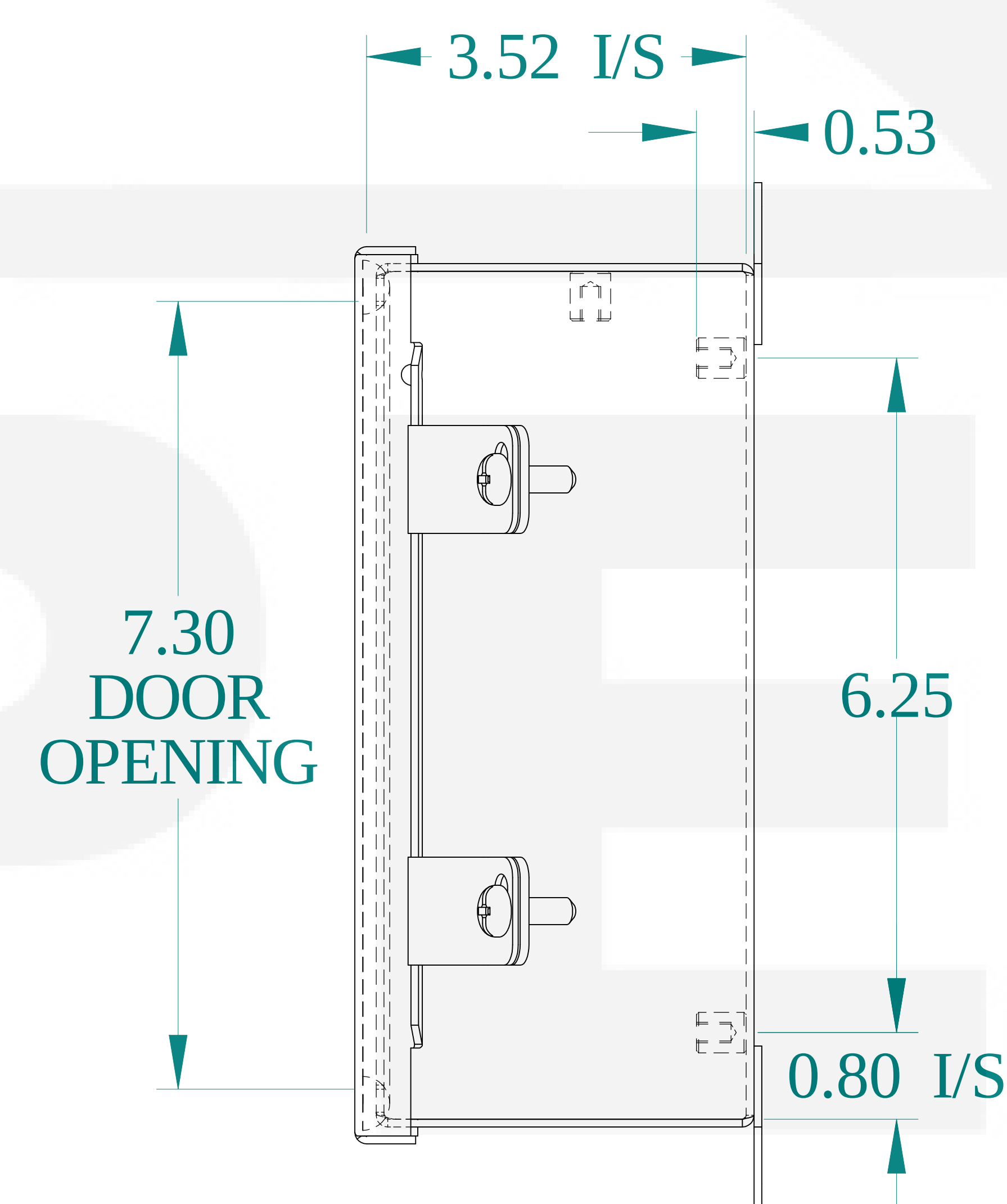
SIDE VIEW
