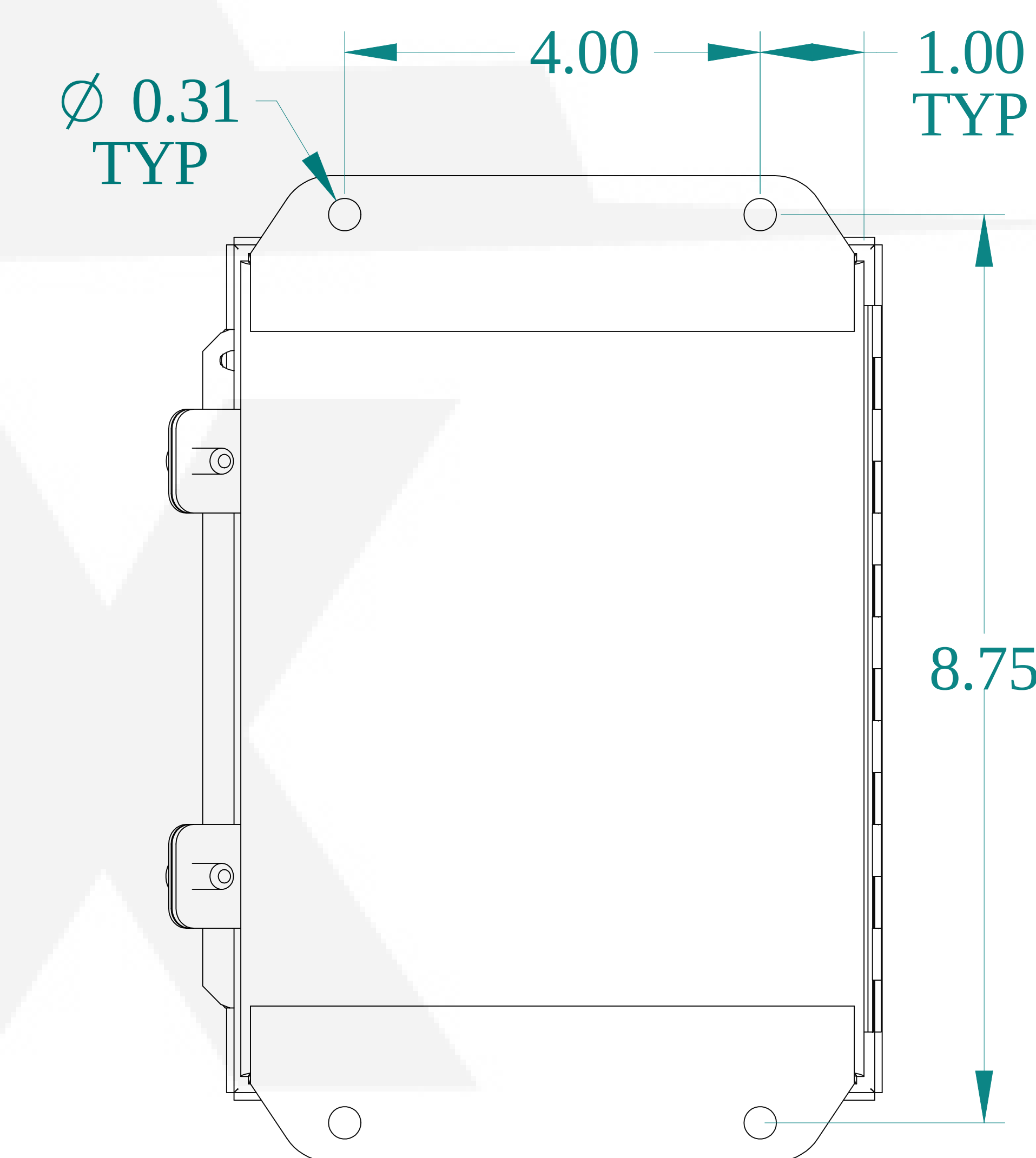
BACK VIEW
