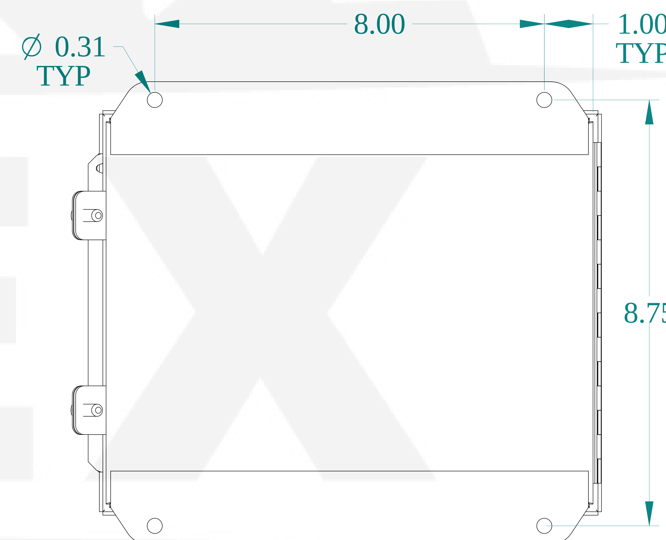
BACK VIEW
