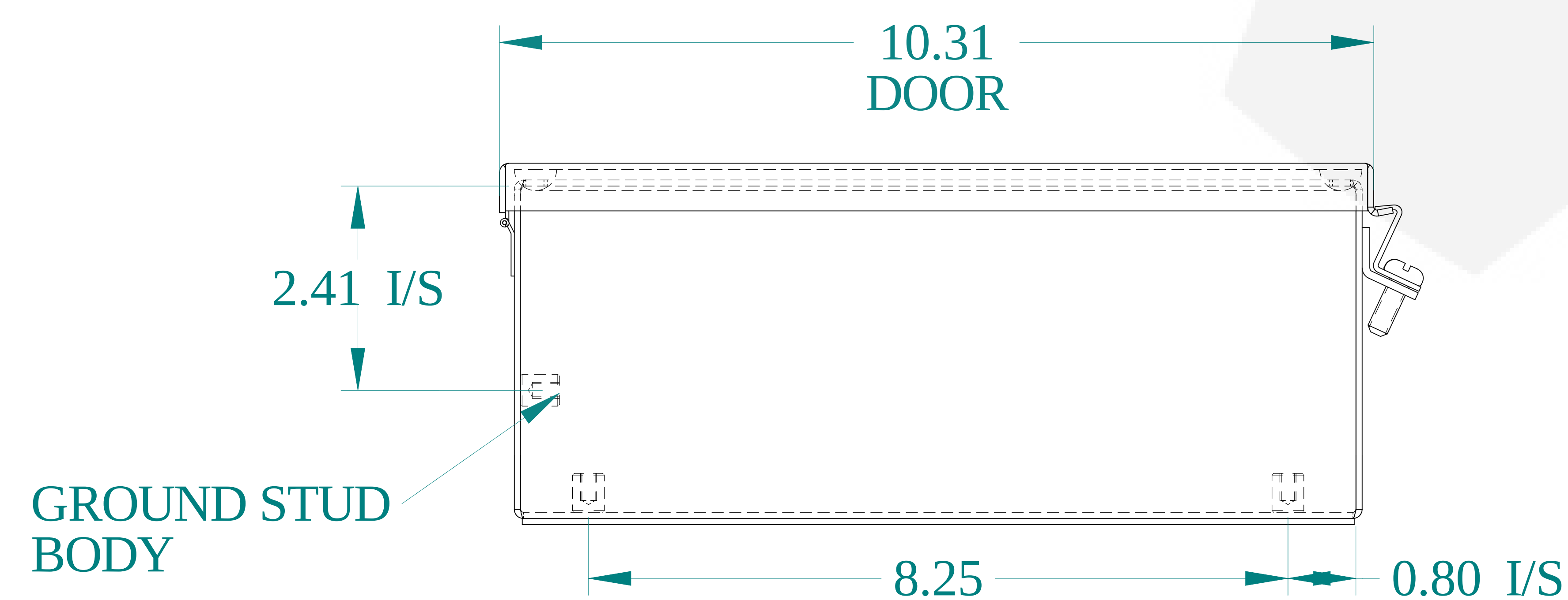
BOTTOM VIEW
