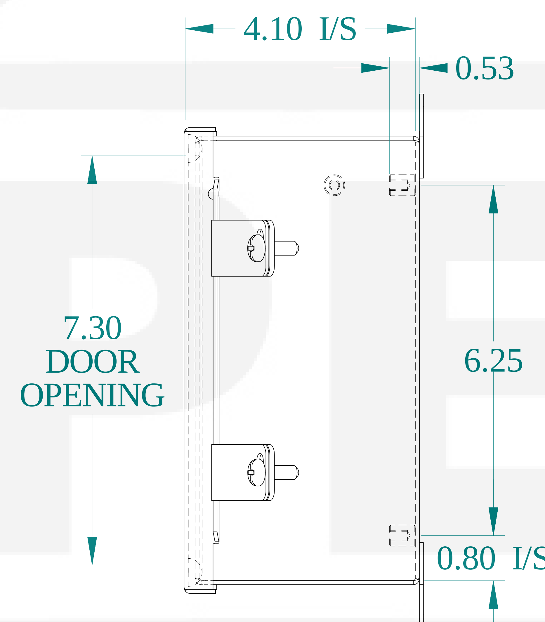
SIDE VIEW
