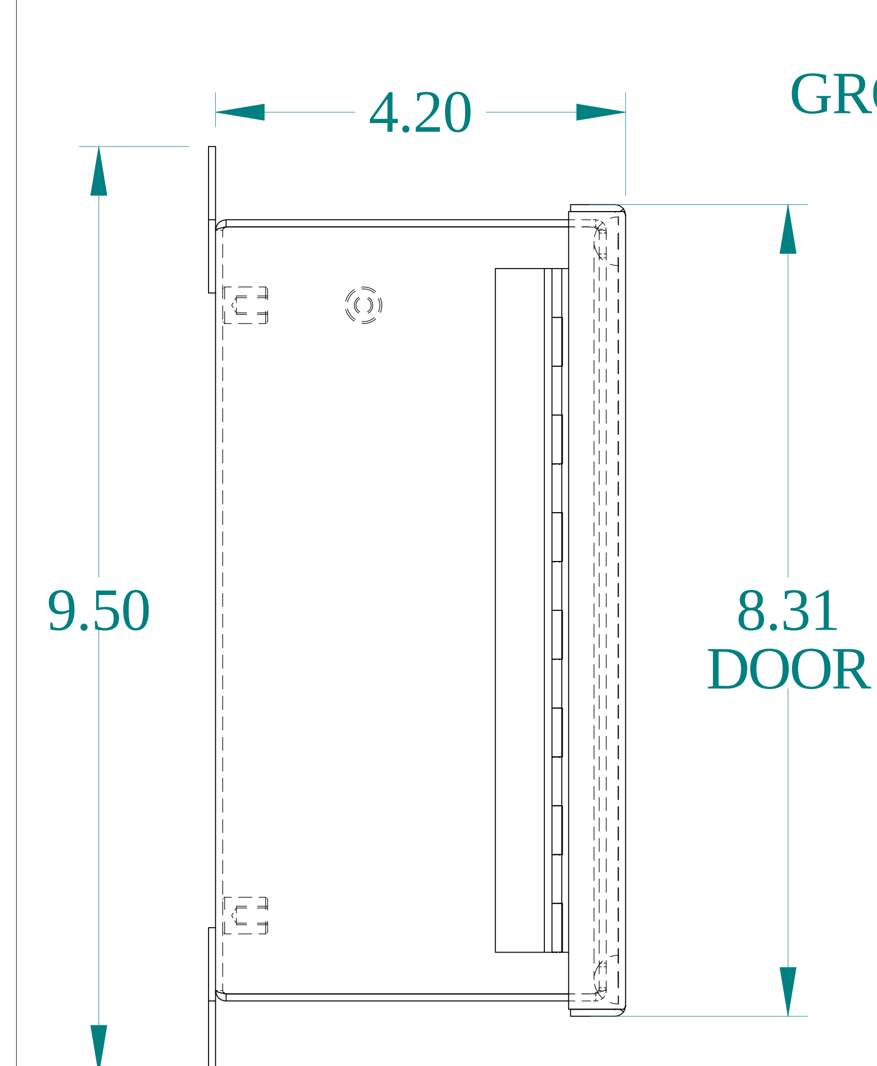
SIDE VIEW
