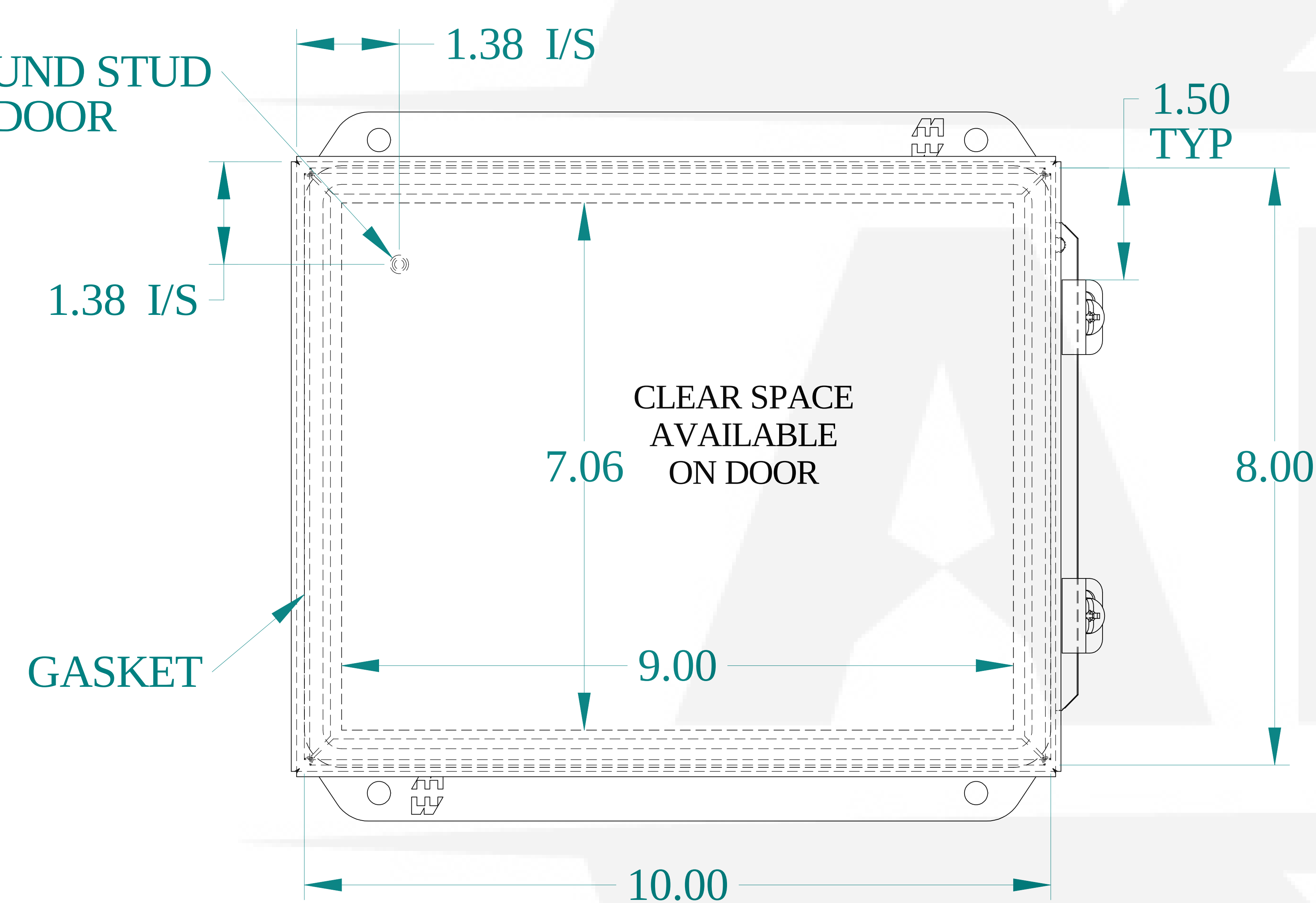
FRONT VIEW
