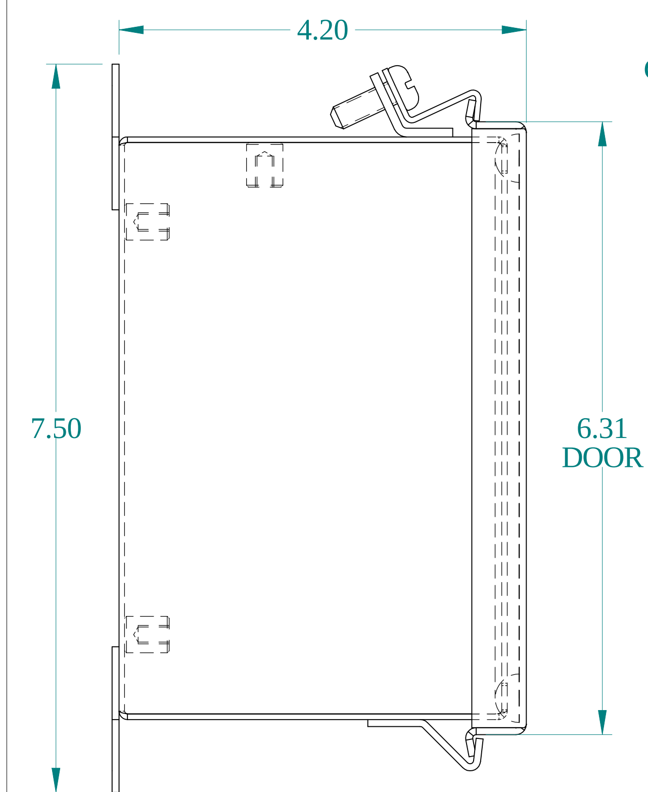
SIDE VIEW
