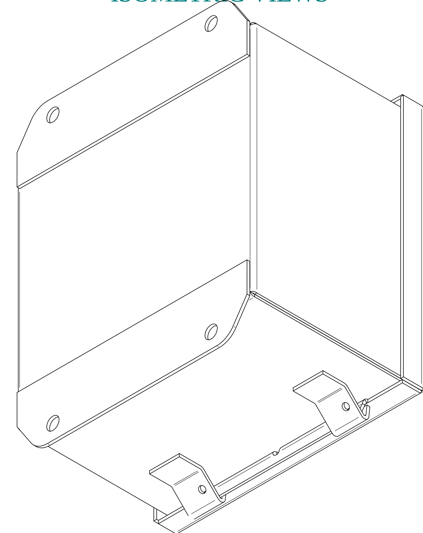
ISOMETRIC VIEWS
