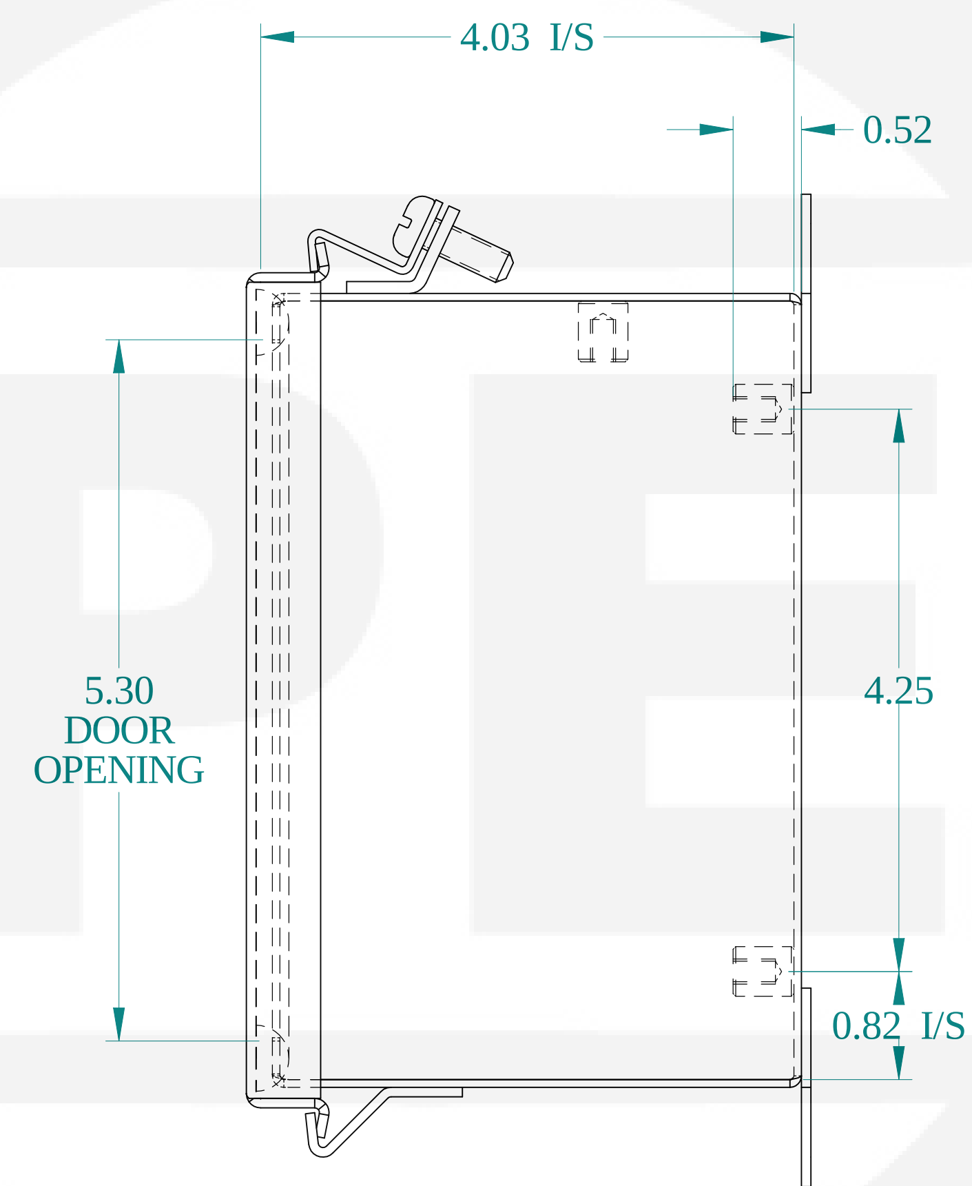
SIDE VIEW
