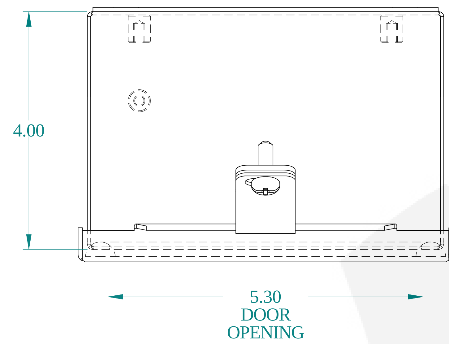
TOP VIEW
