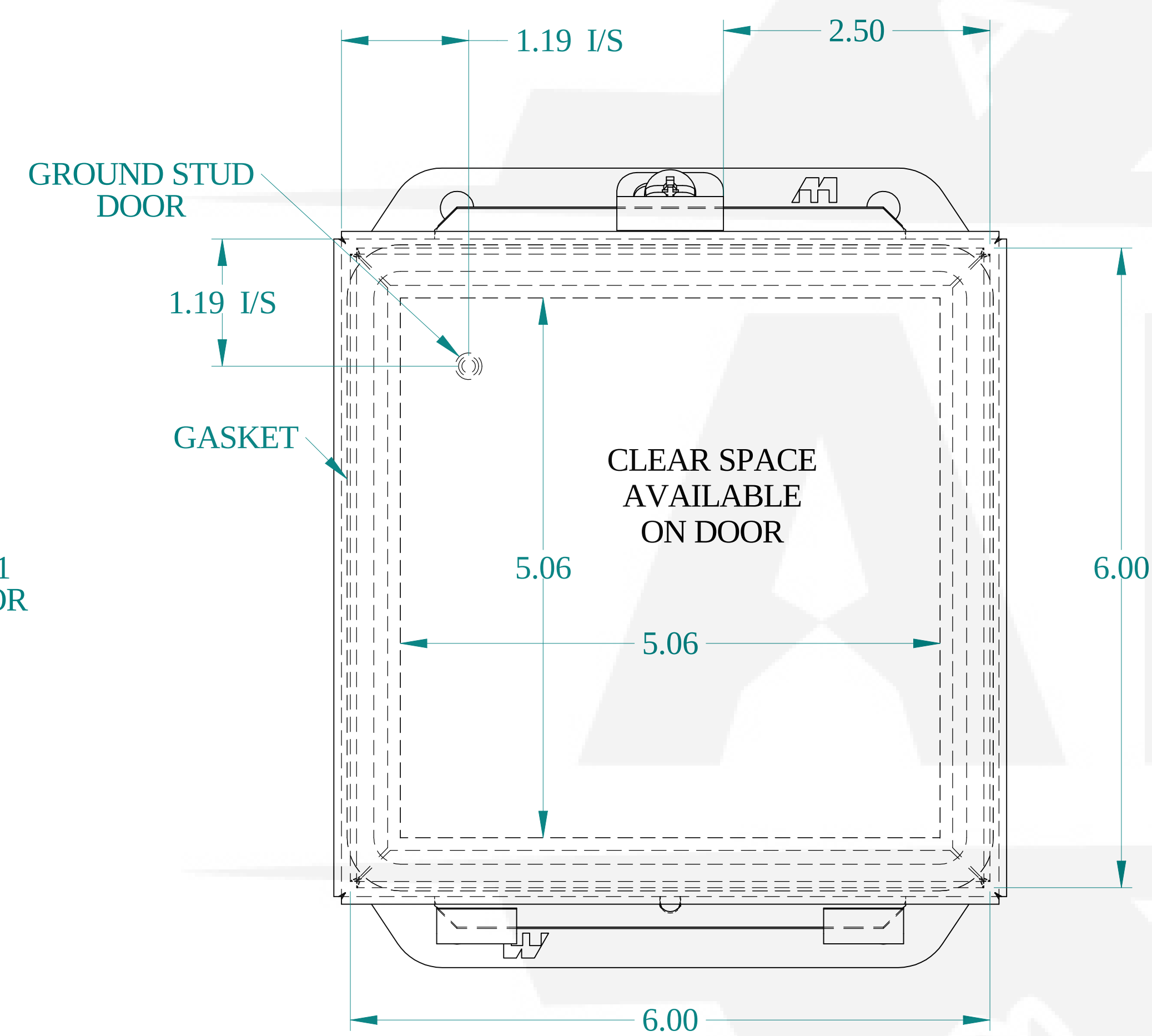
FRONT VIEW
