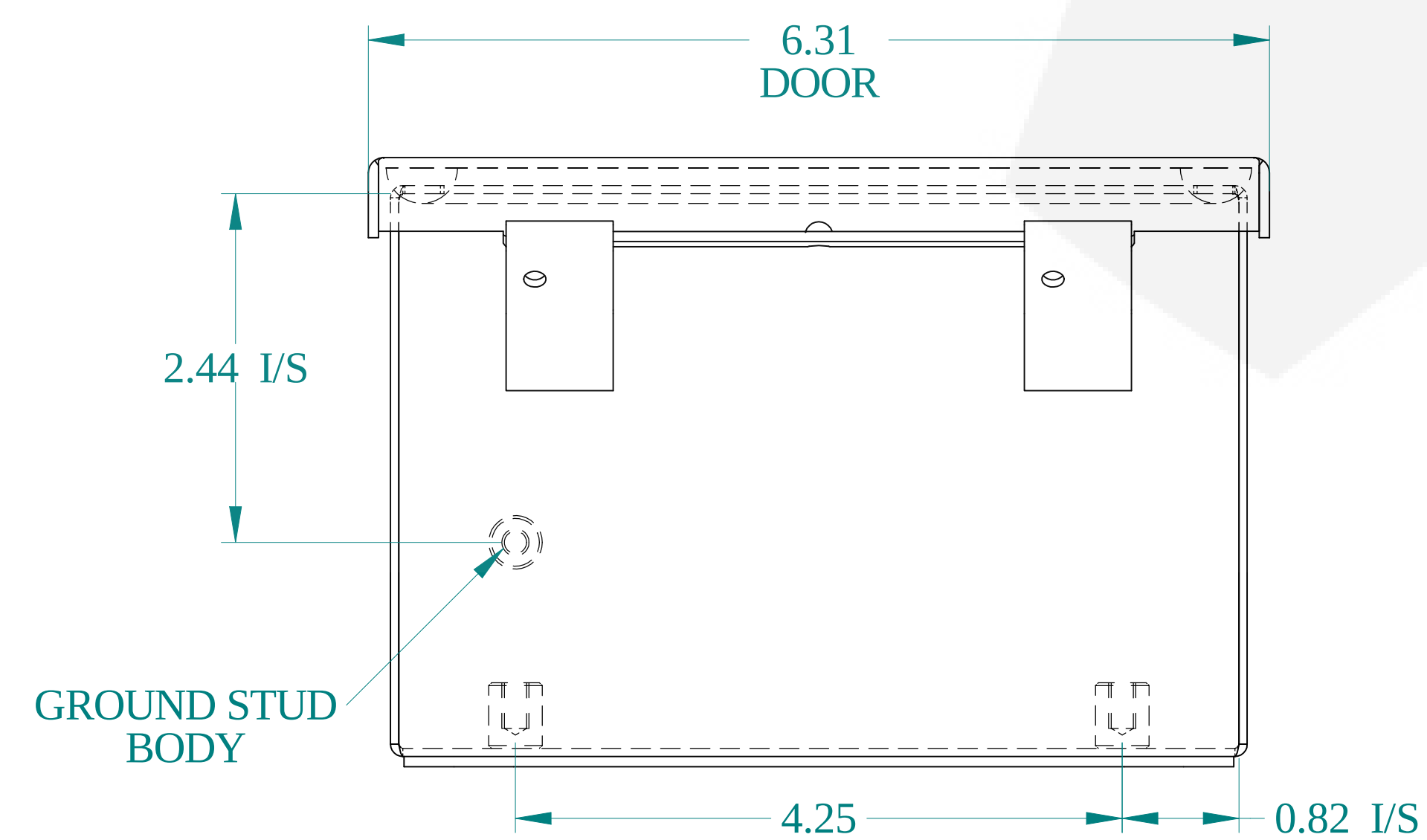
BOTTOM VIEW
