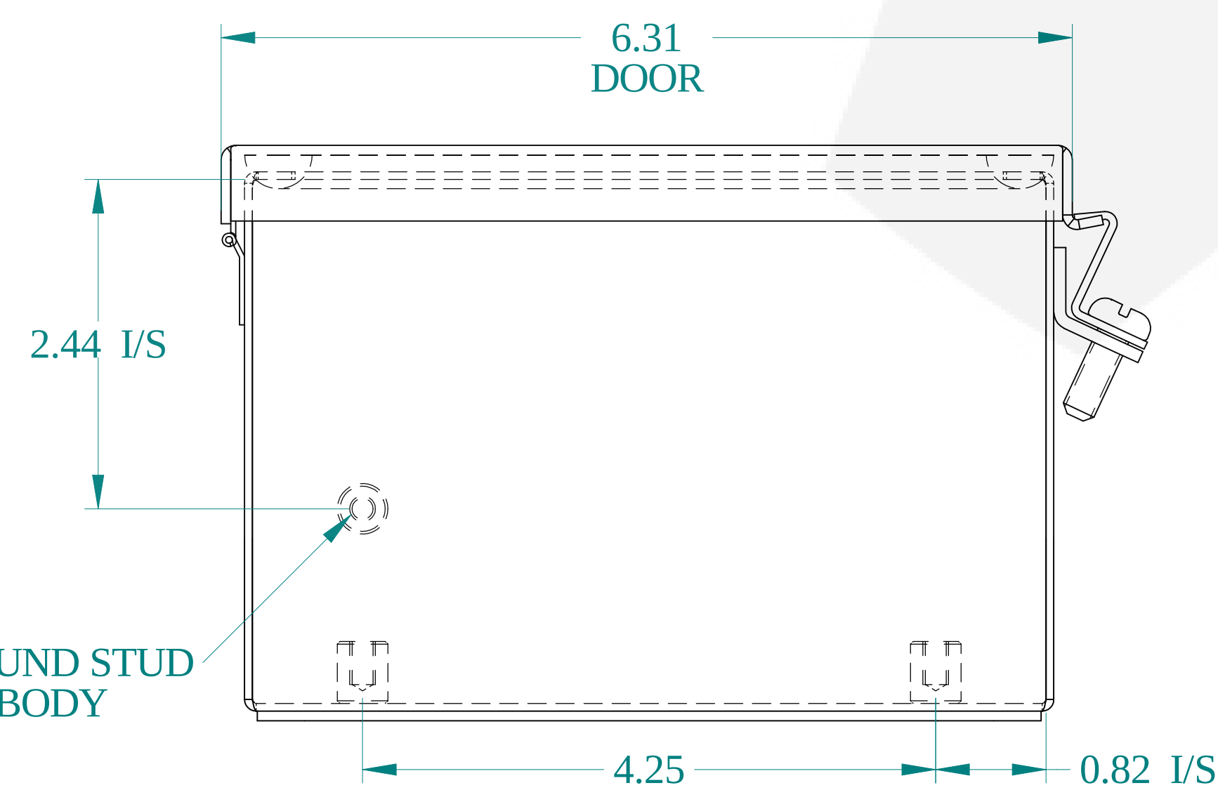
BOTTOM VIEW
