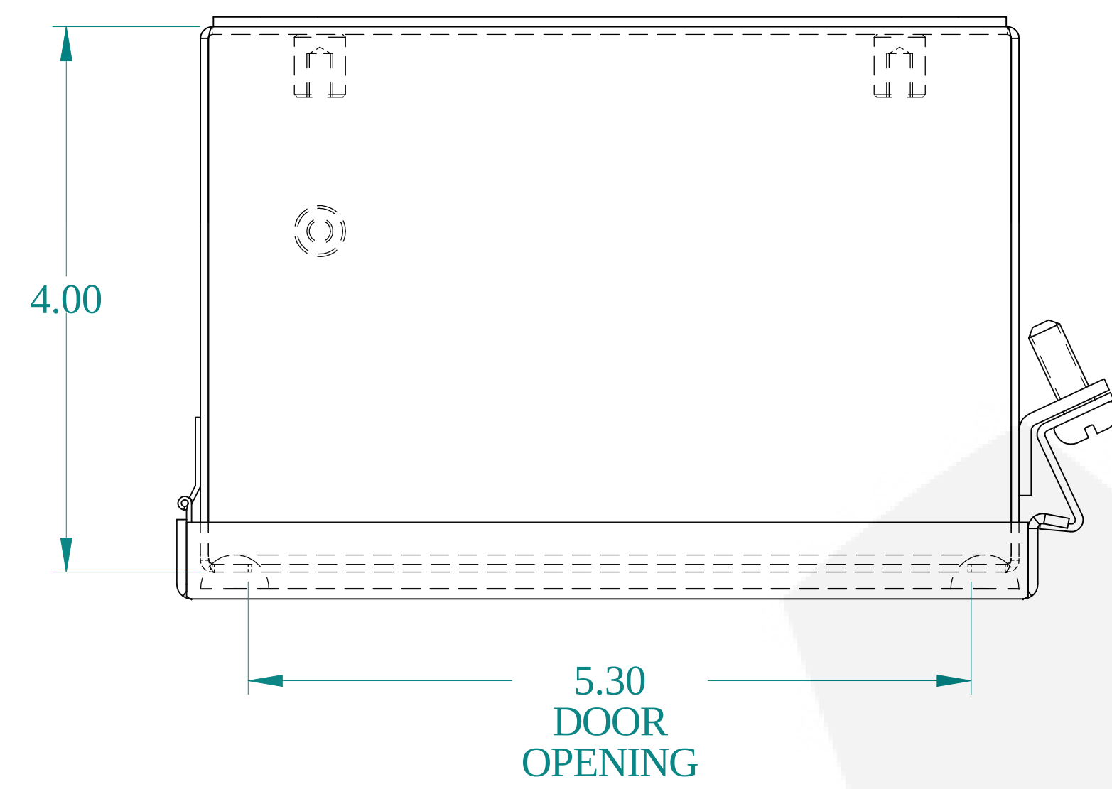
TOP VIEW
