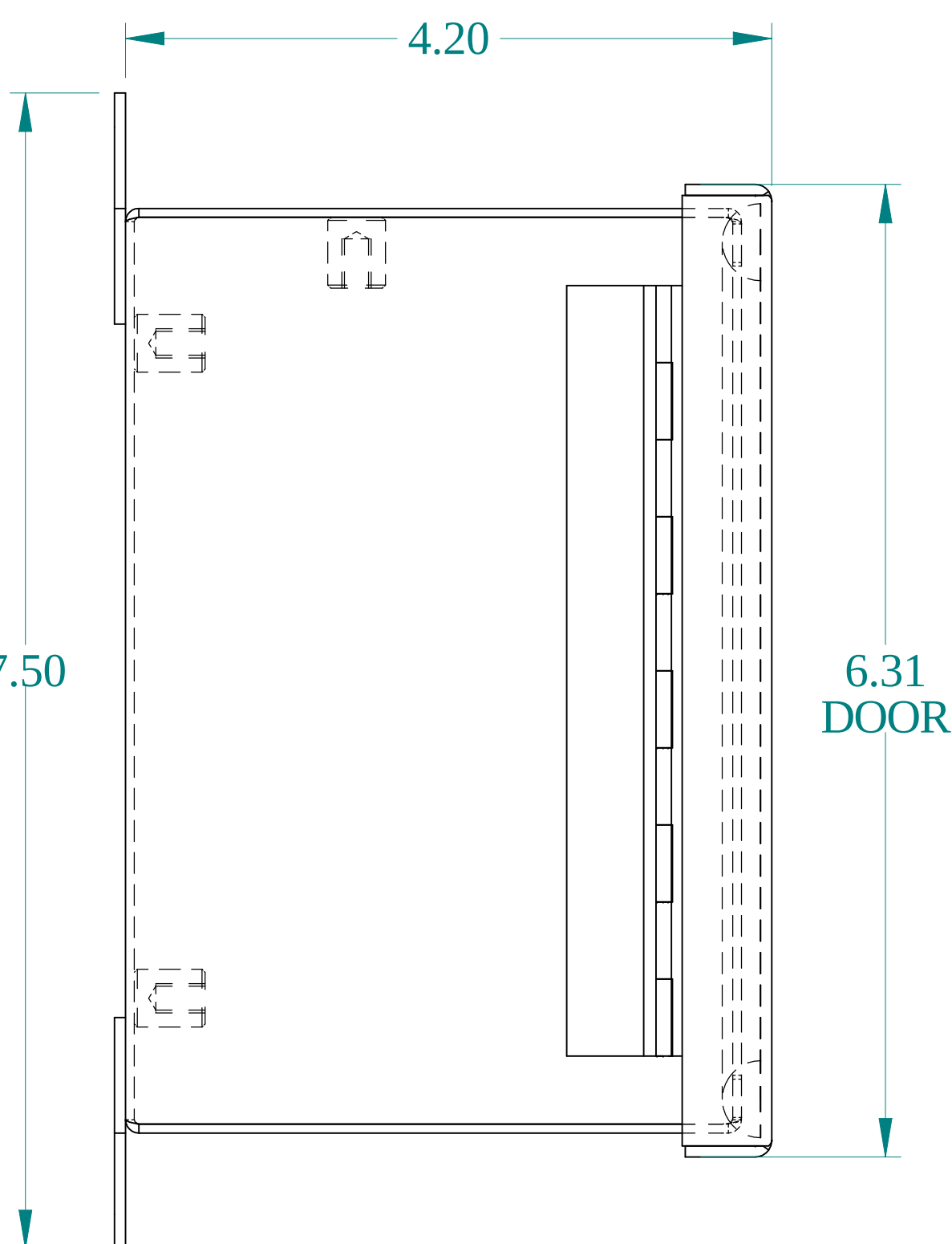
SIDE VIEW
