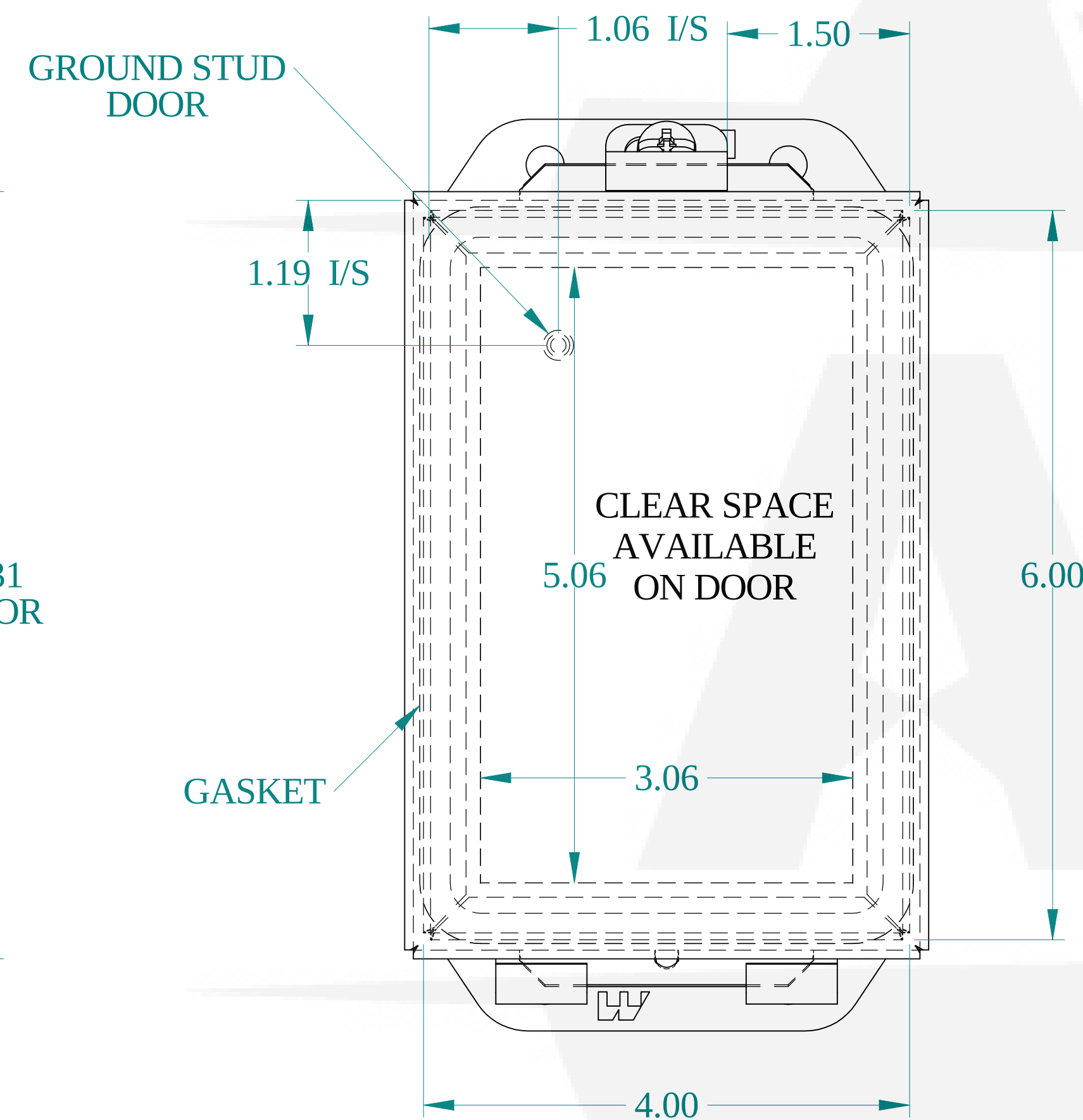
FRONT VIEW
