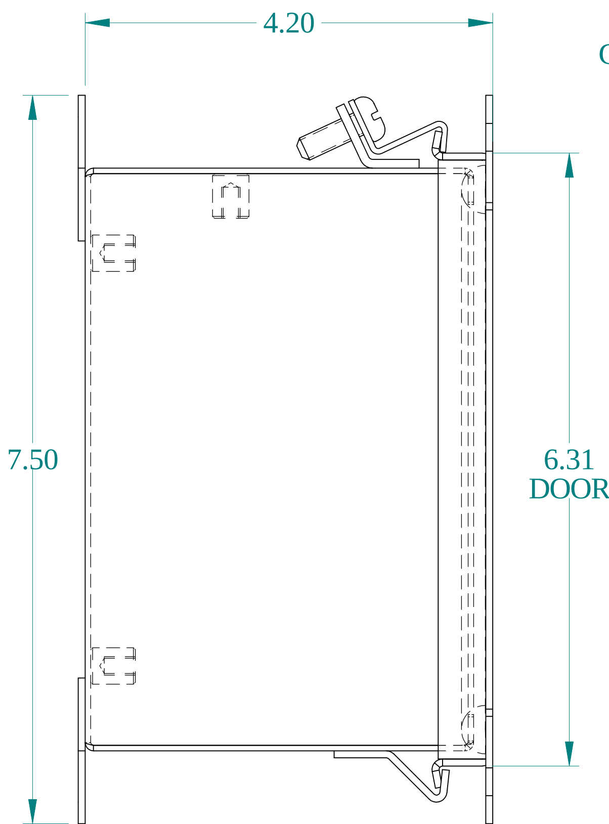
SIDE VIEW
