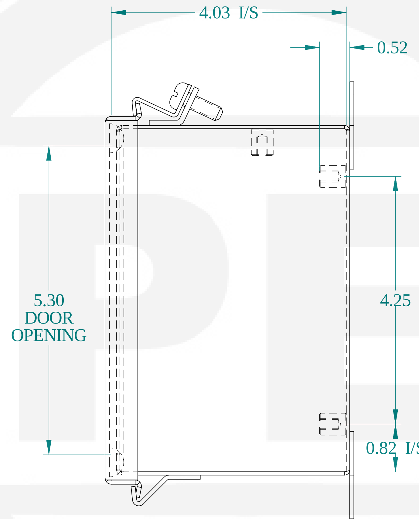
SIDE VIEW
