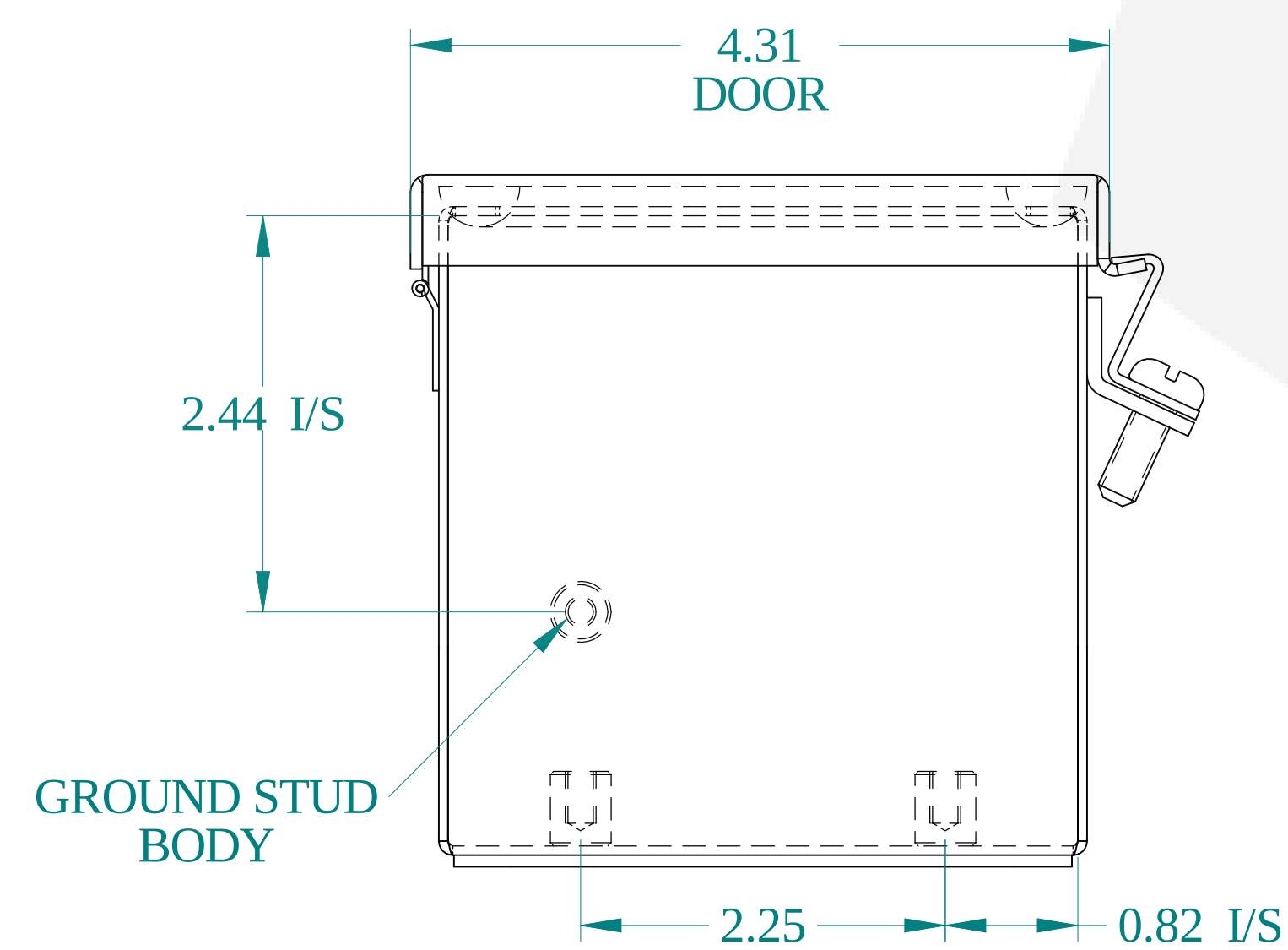
BOTTOM VIEW
