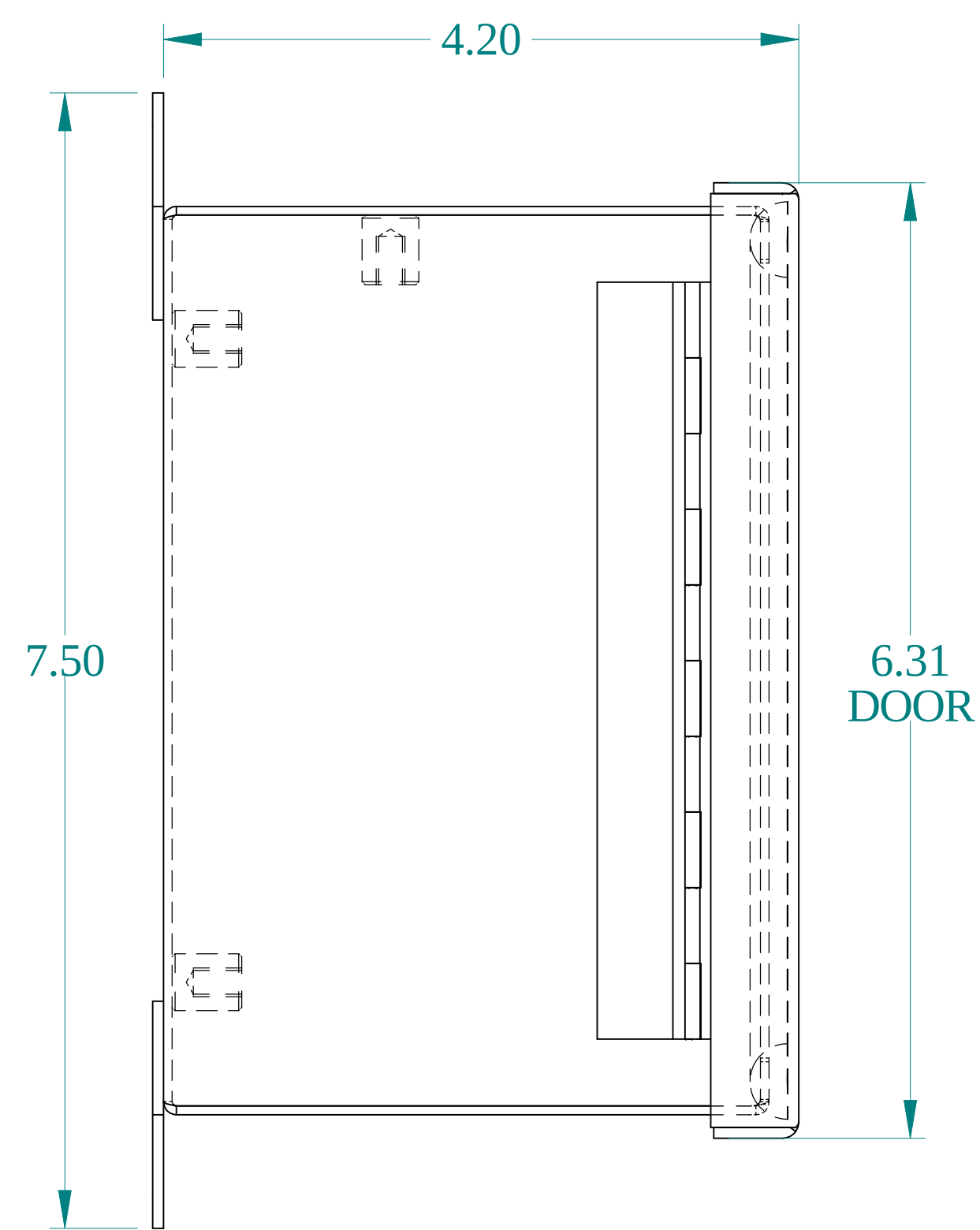
SIDE VIEW
