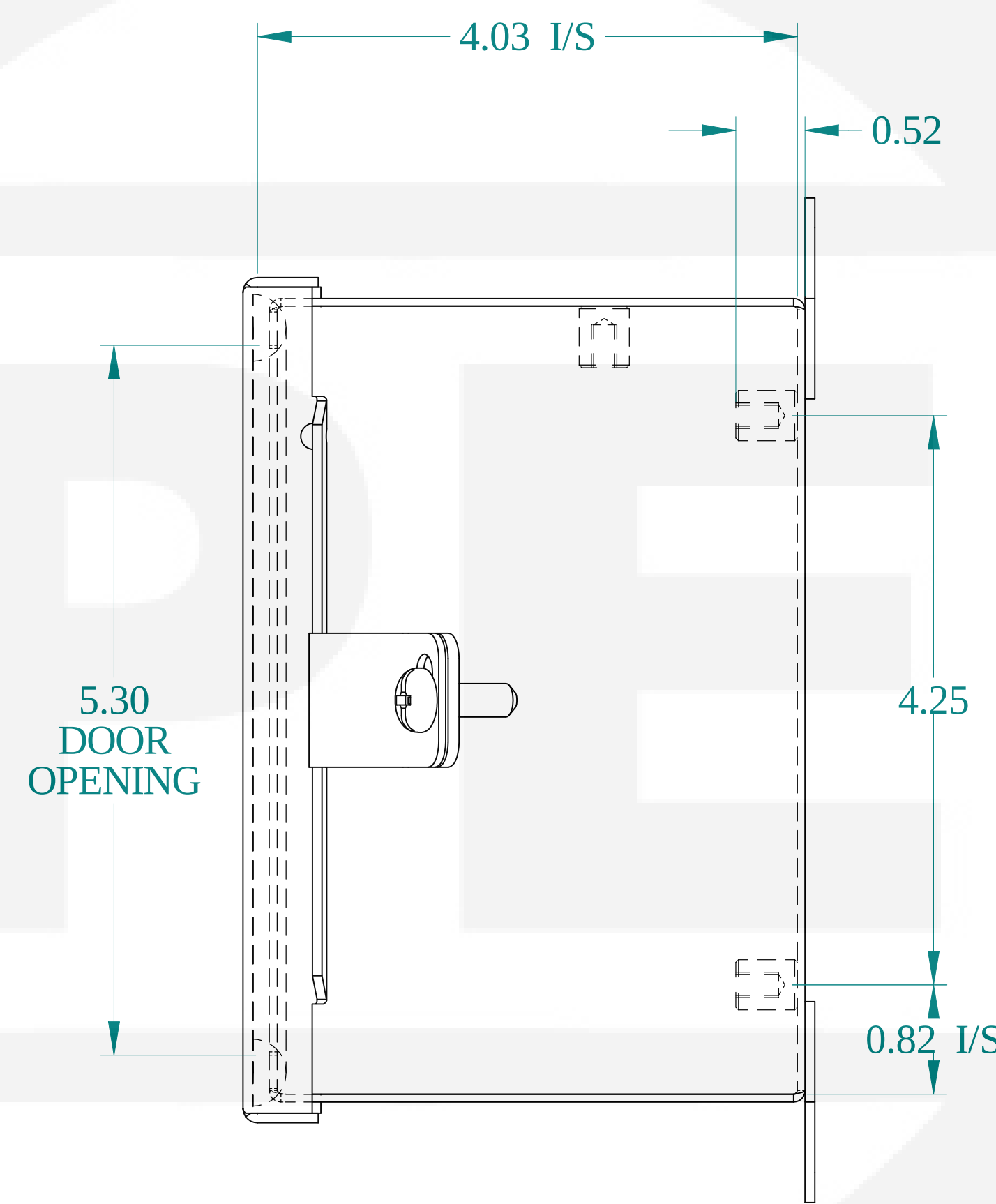
SIDE VIEW
