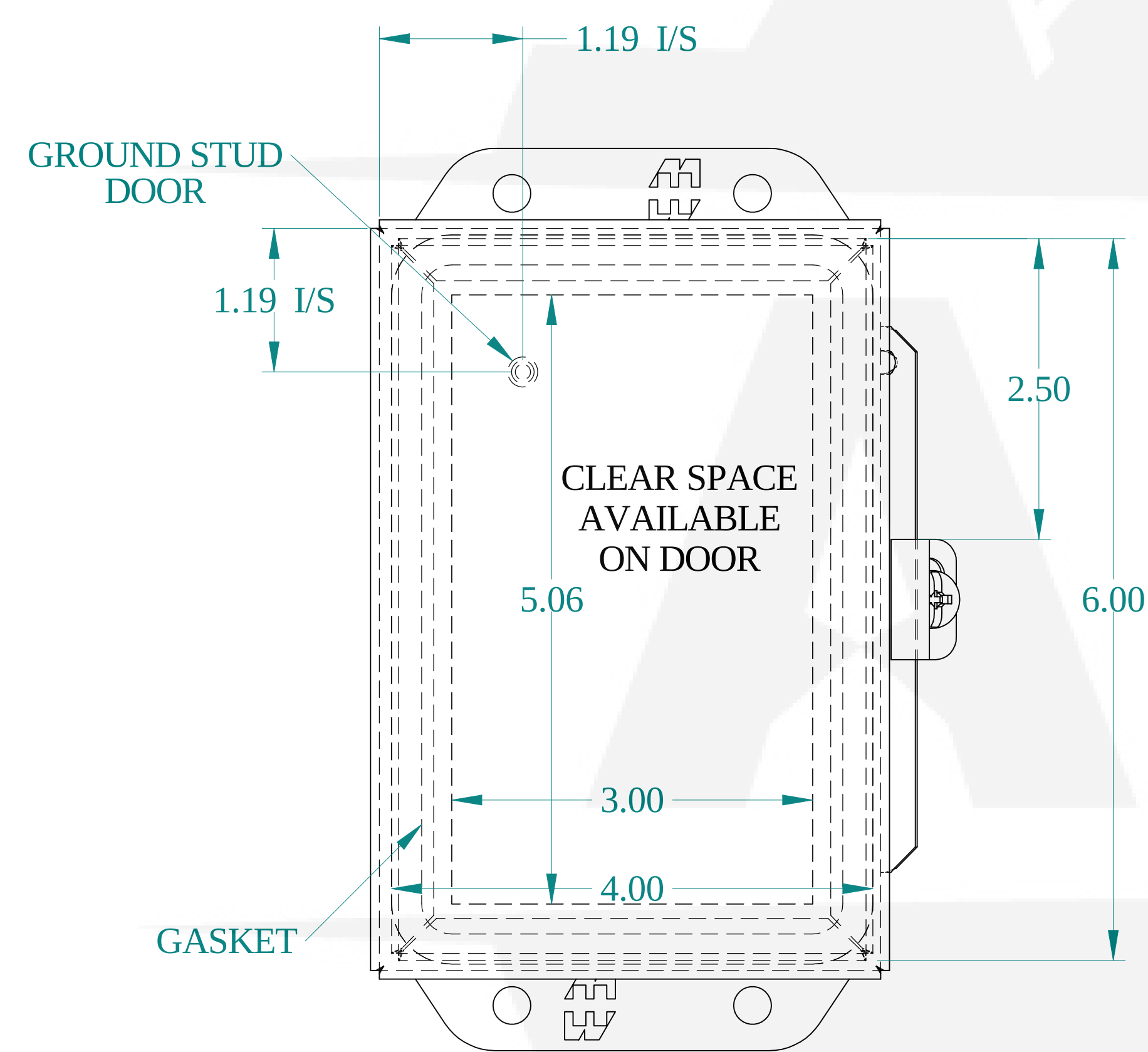
FRONT VIEW
