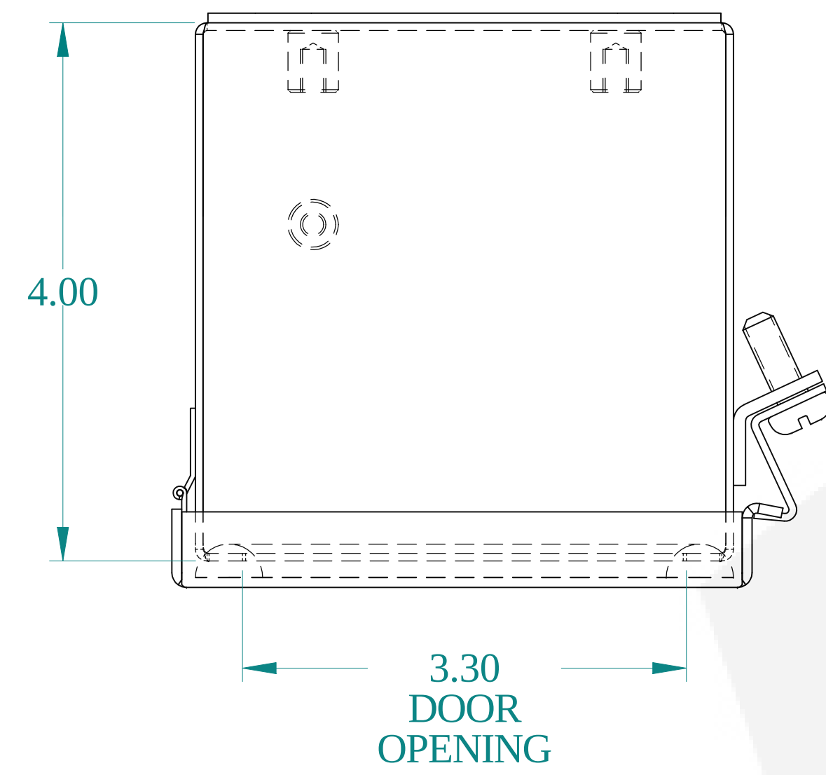
TOP VIEW
