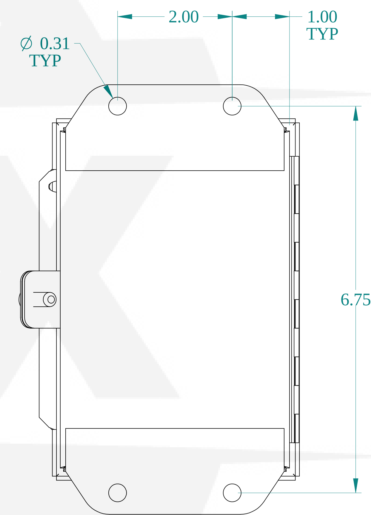
BACK VIEW
