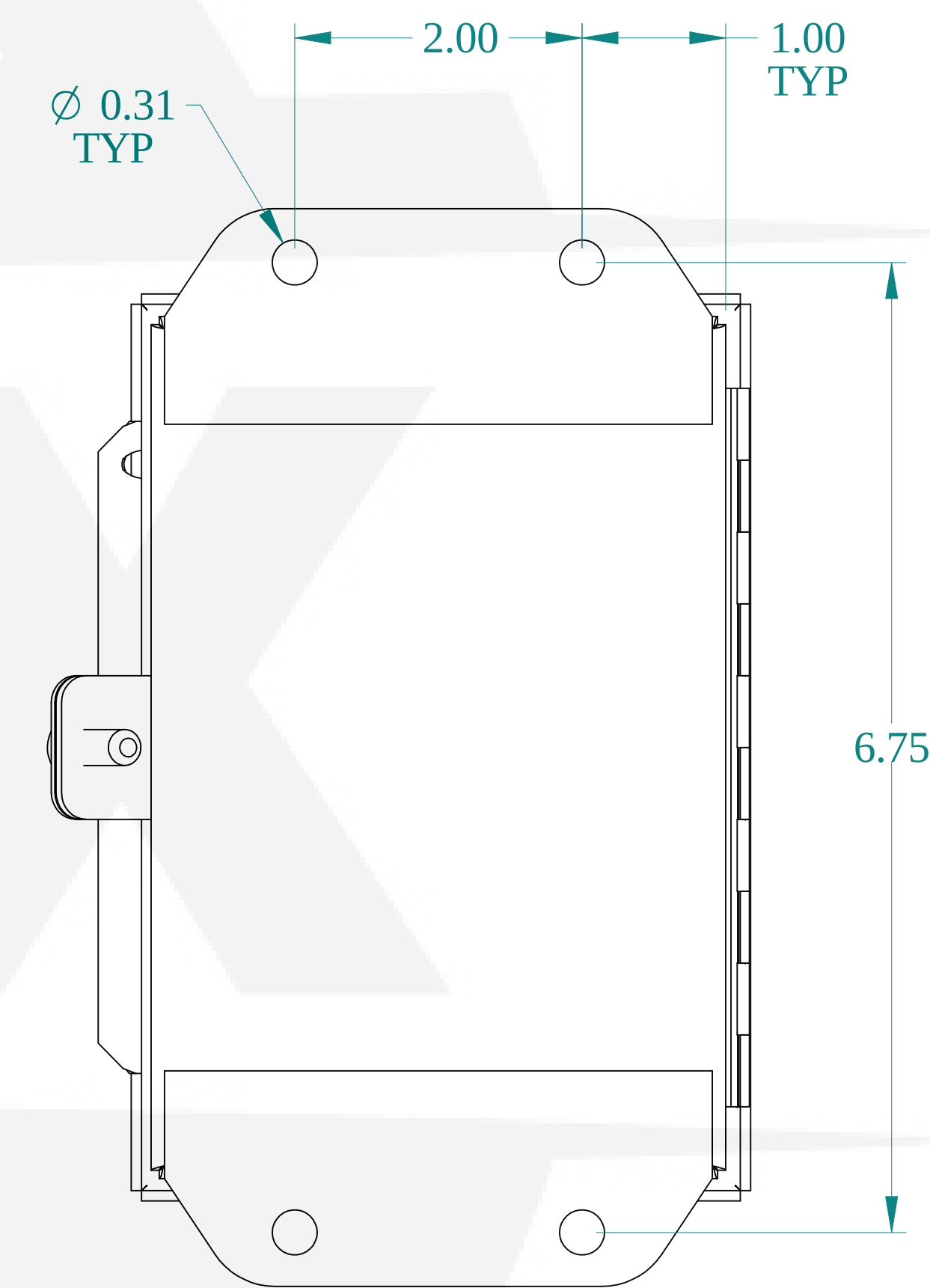
BACK VIEW
