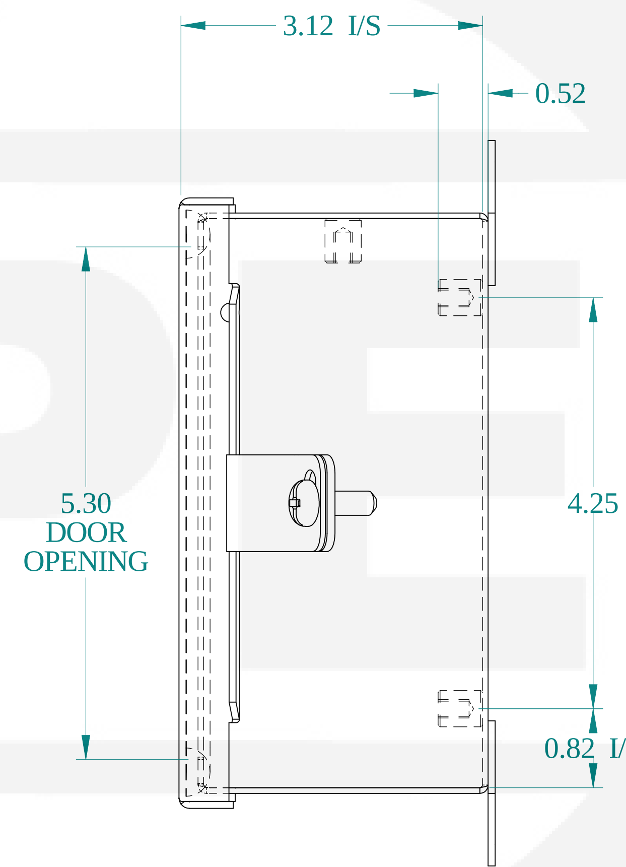
SIDE VIEW
