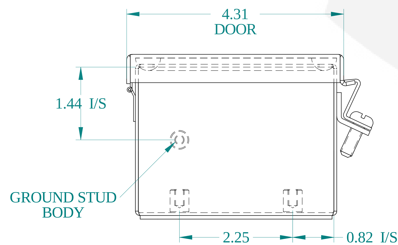
BOTTOM VIEW
