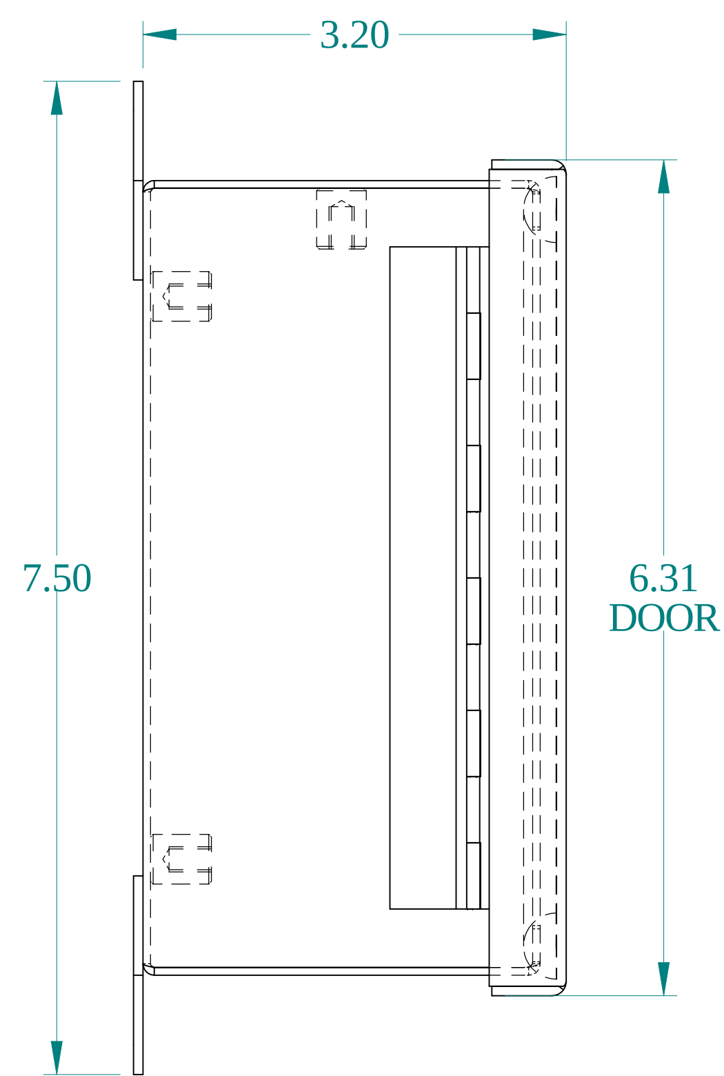
SIDE VIEW
