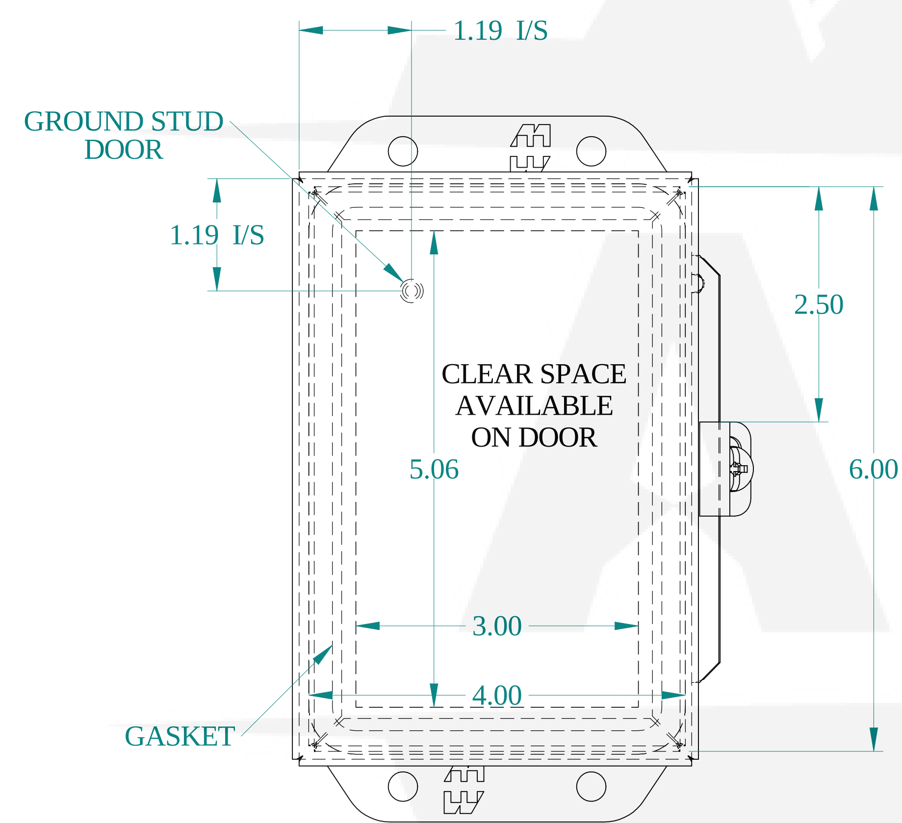
FRONT VIEW
