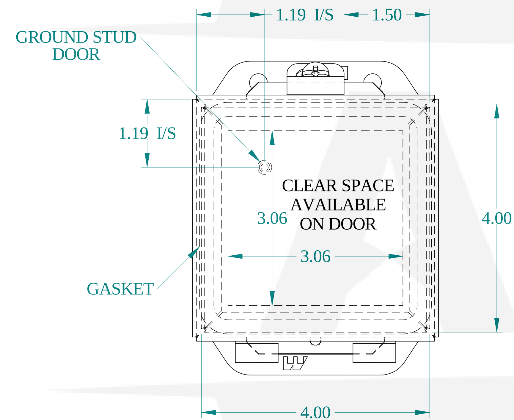
FRONT VIEW
