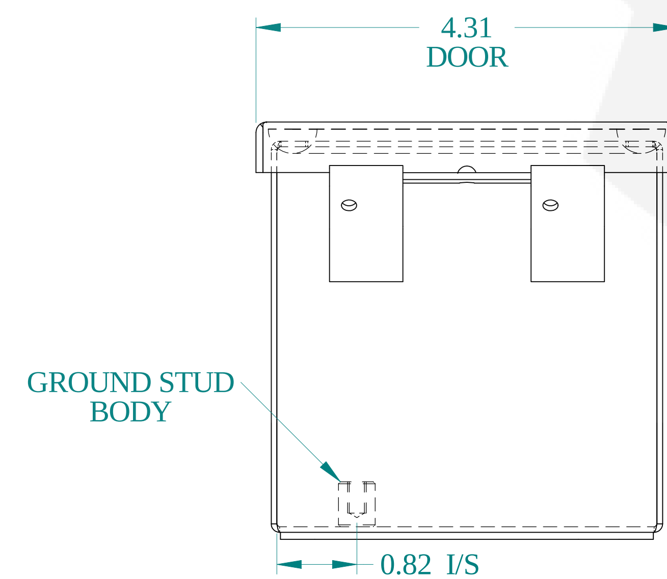
BOTTOM VIEW
