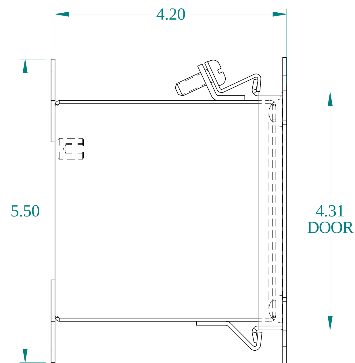
SIDE VIEW
