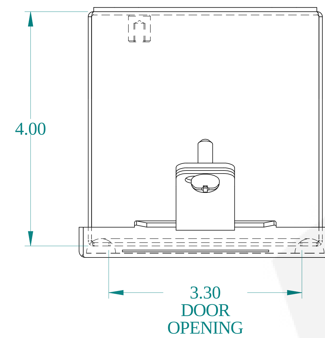
TOP VIEW
