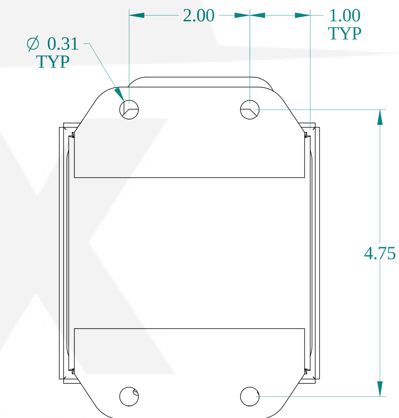
BACK VIEW
