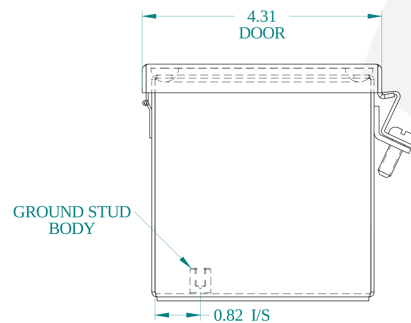
BOTTOM VIEW
