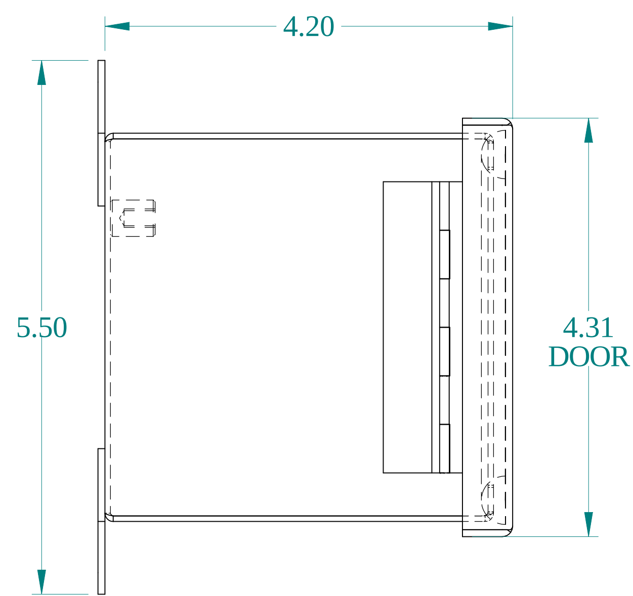
SIDE VIEW
