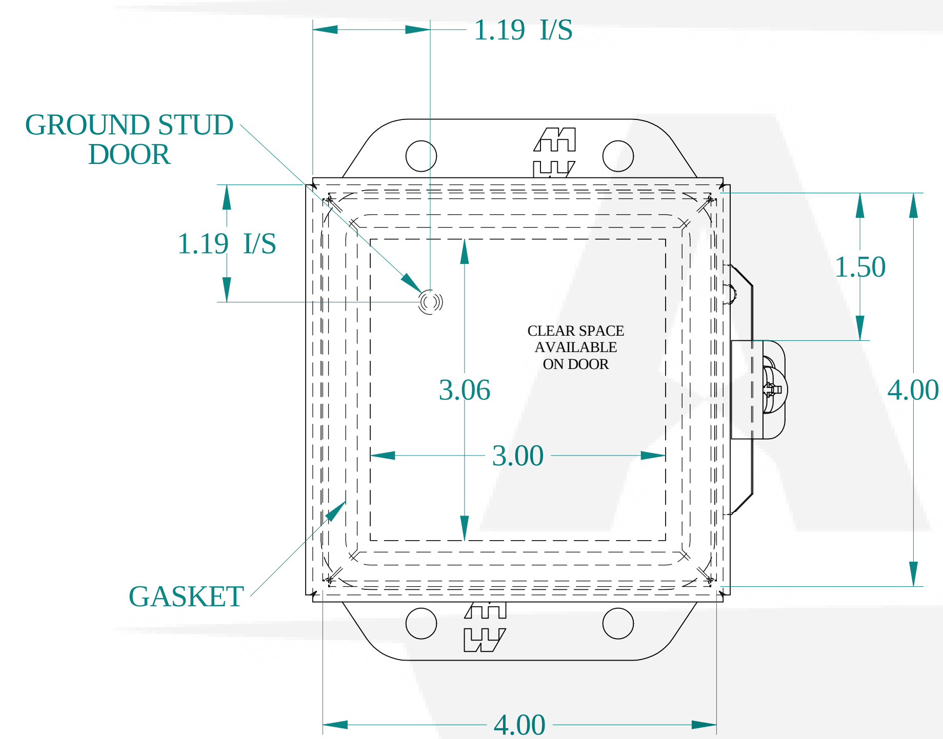
FRONT VIEW
