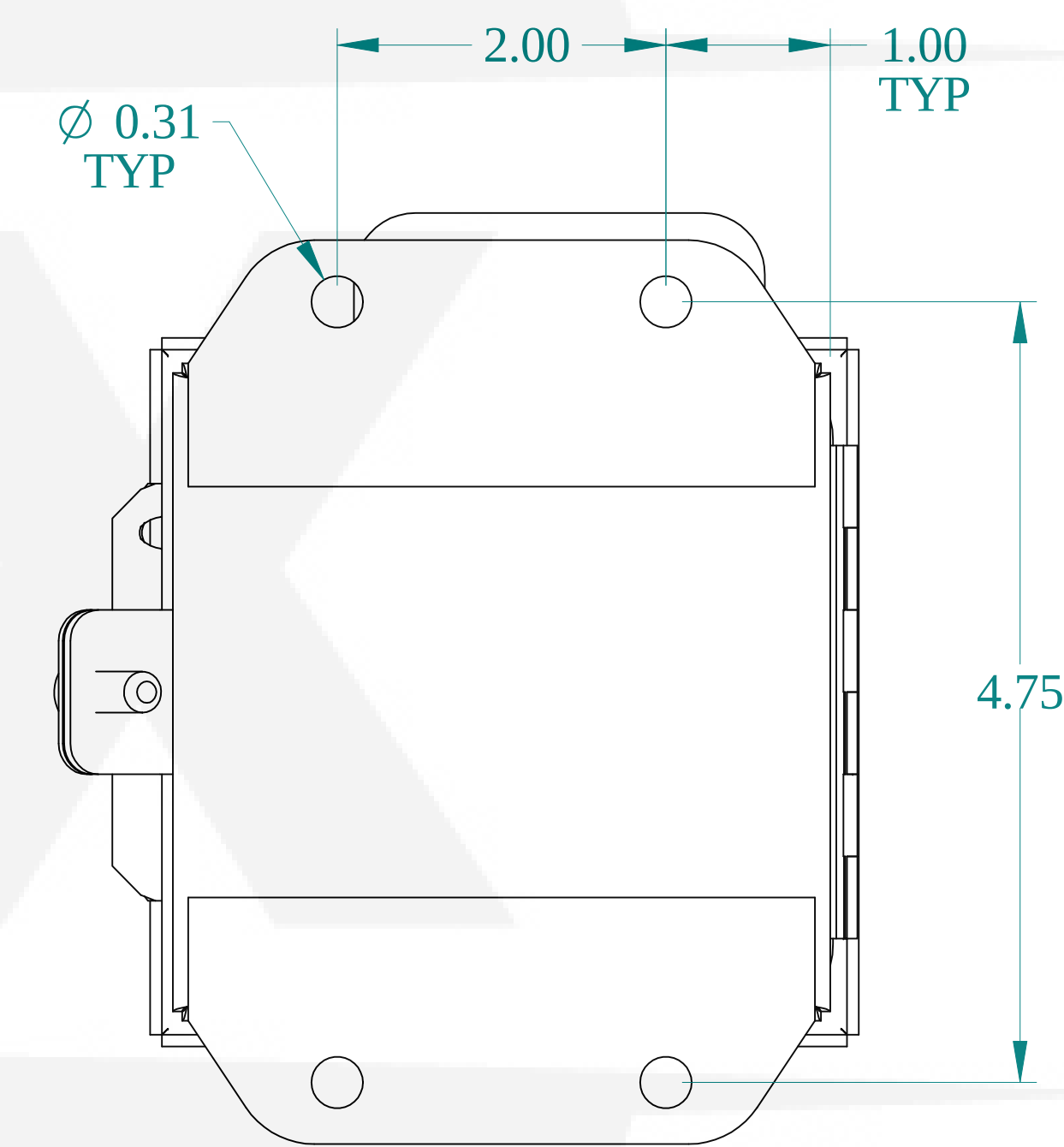
BACK VIEW
