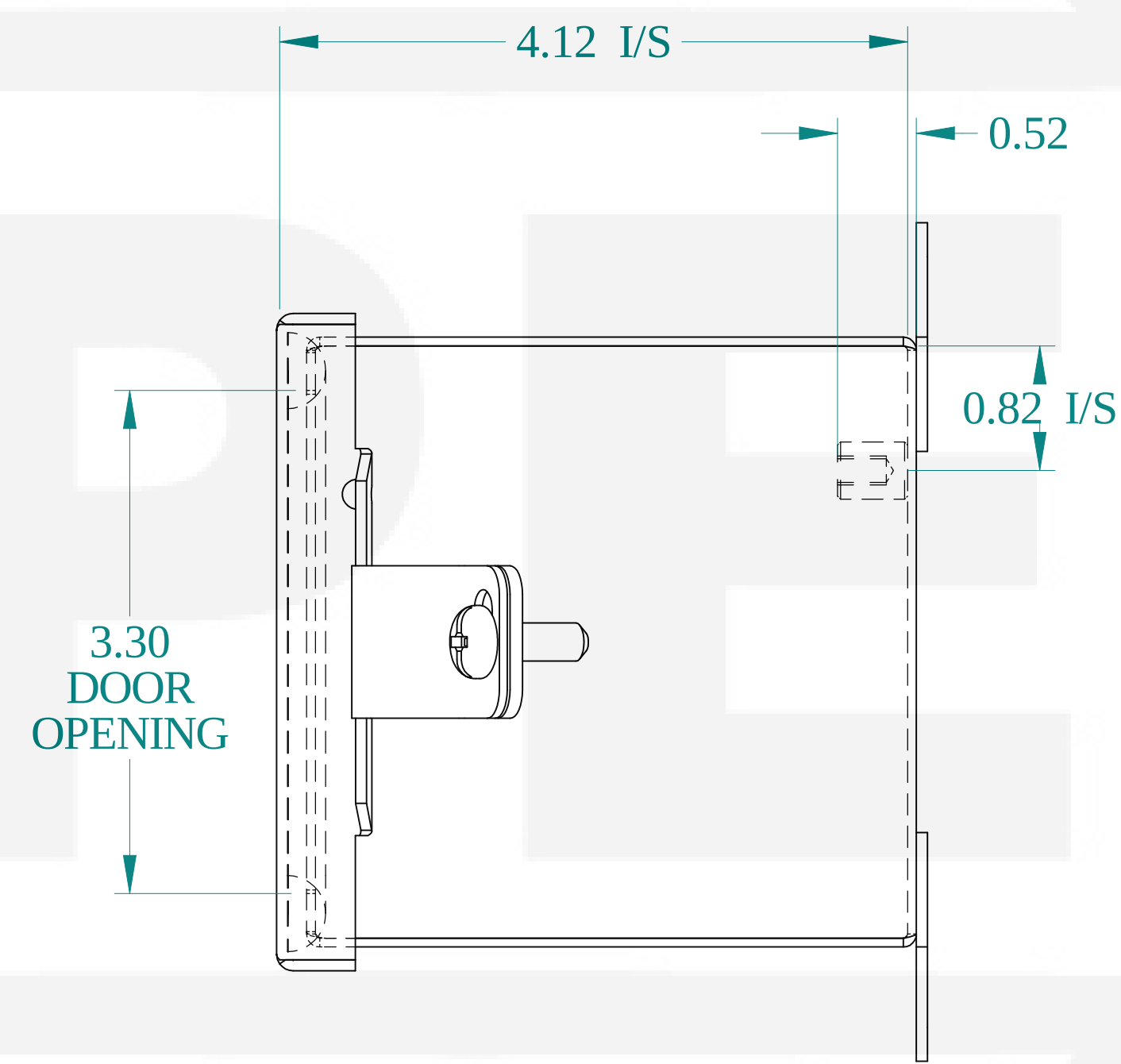
SIDE VIEW
