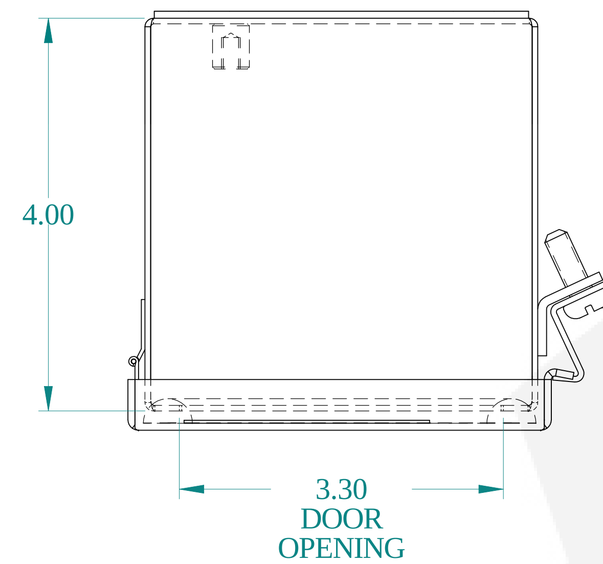
TOP VIEW
