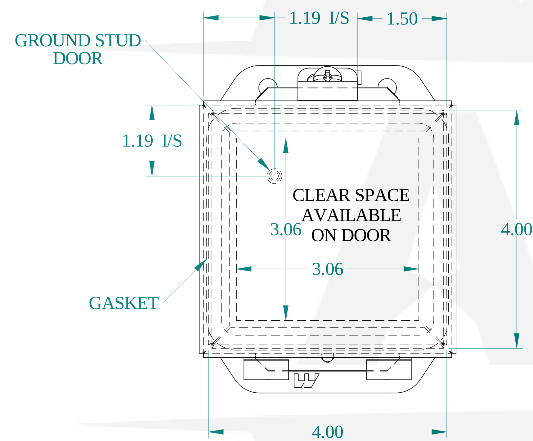
FRONT VIEW
