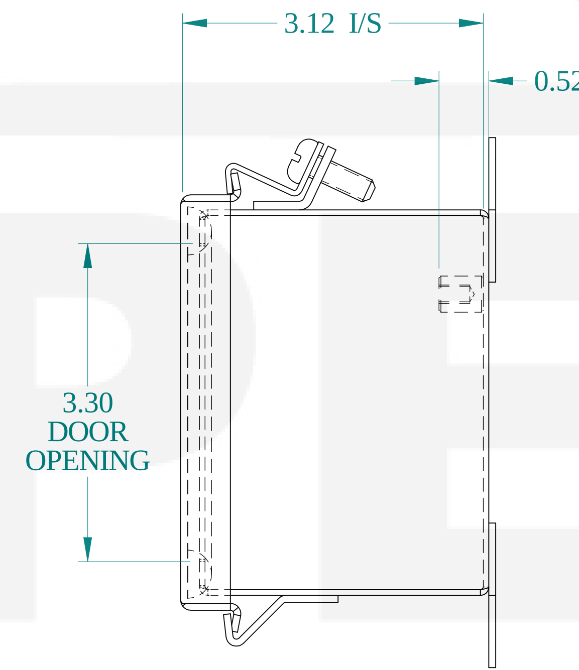
SIDE VIEW
