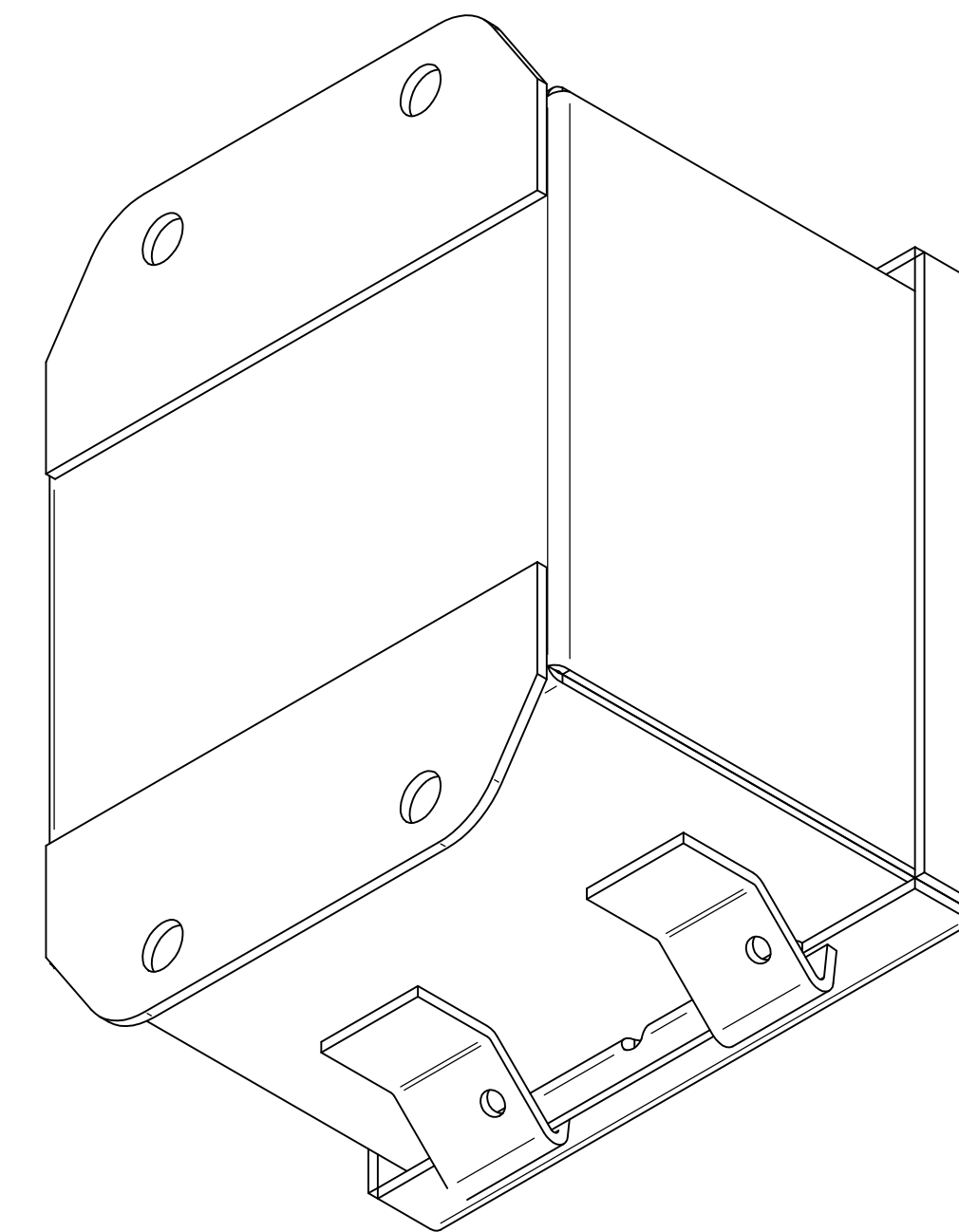
ISOMETRIC VIEWS
