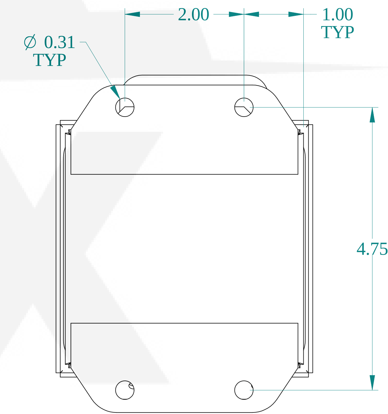
BACK VIEW
