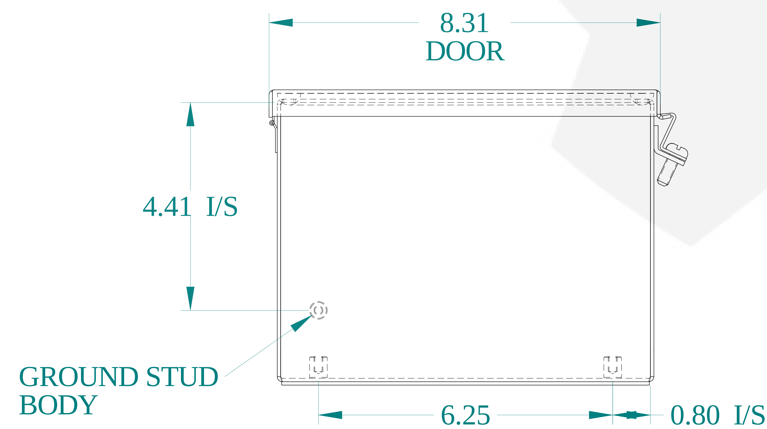
BOTTOM VIEW
