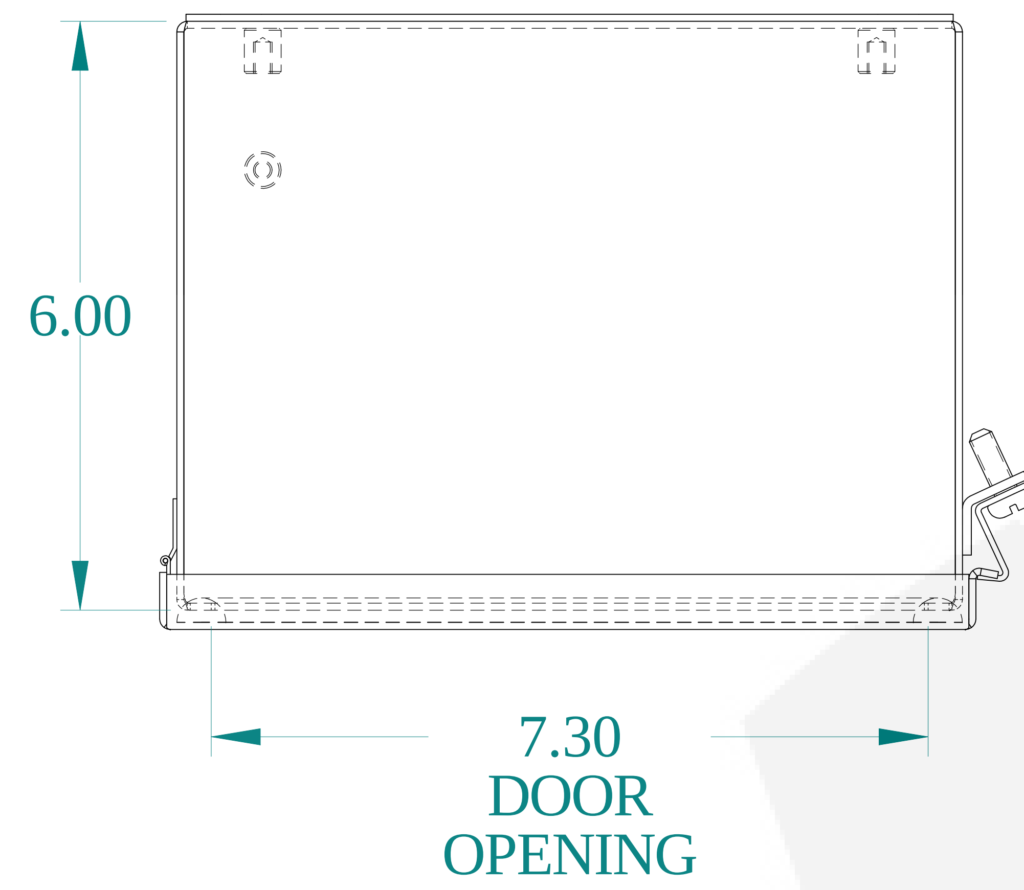
TOP VIEW
