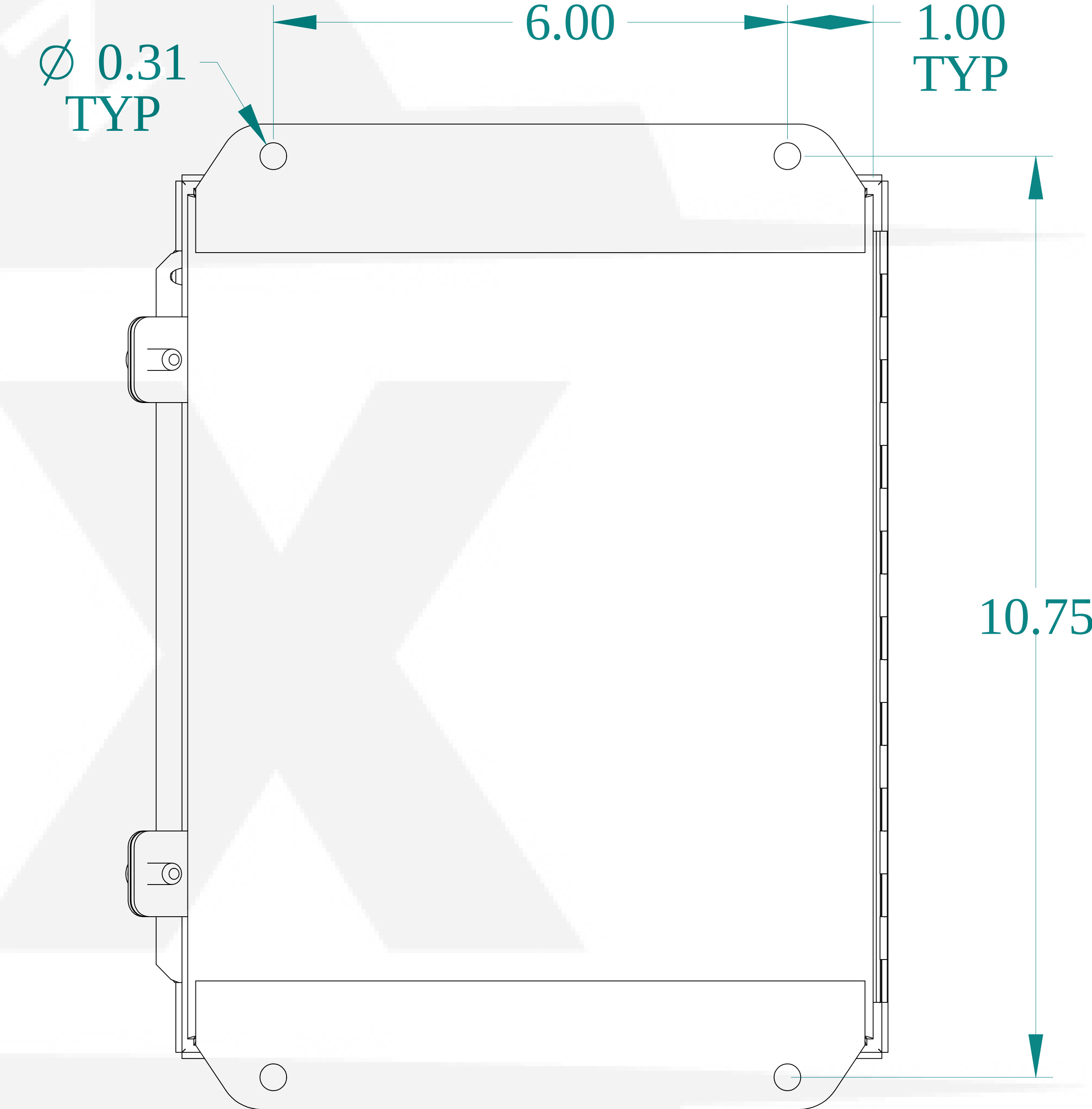
BACK VIEW
