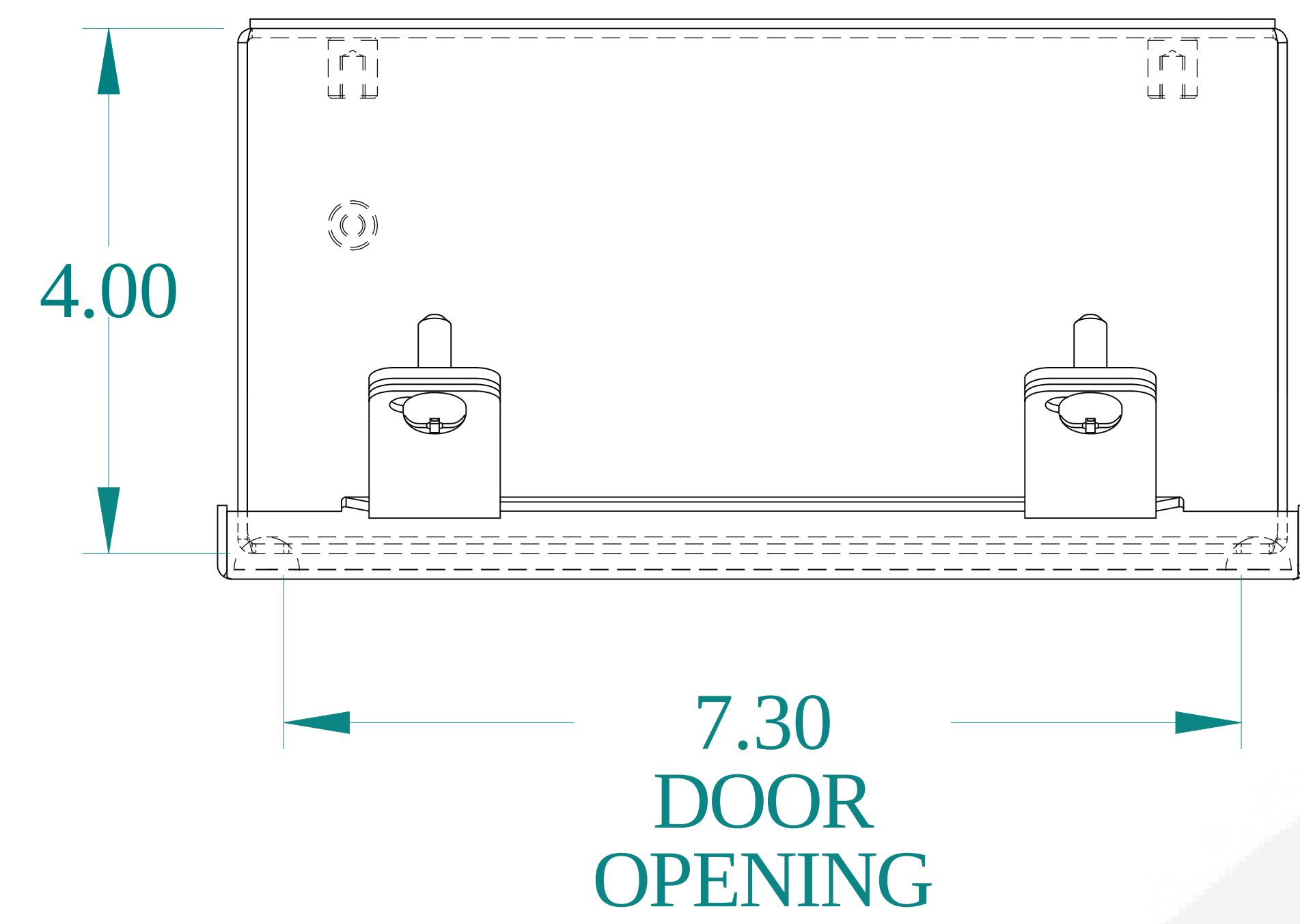
TOP VIEW
