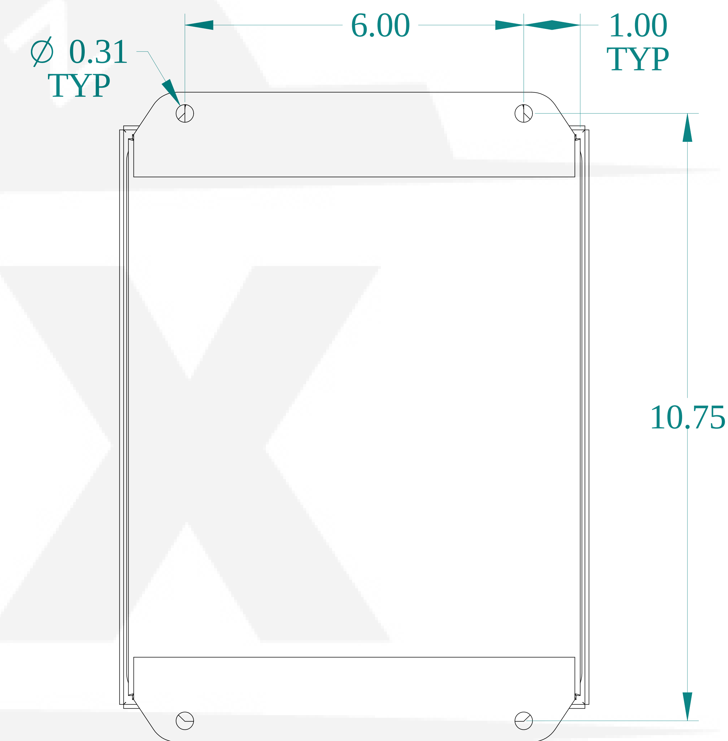
BACK VIEW
