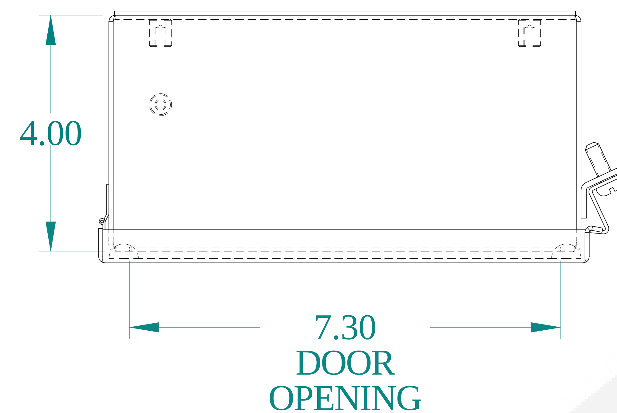
TOP VIEW
