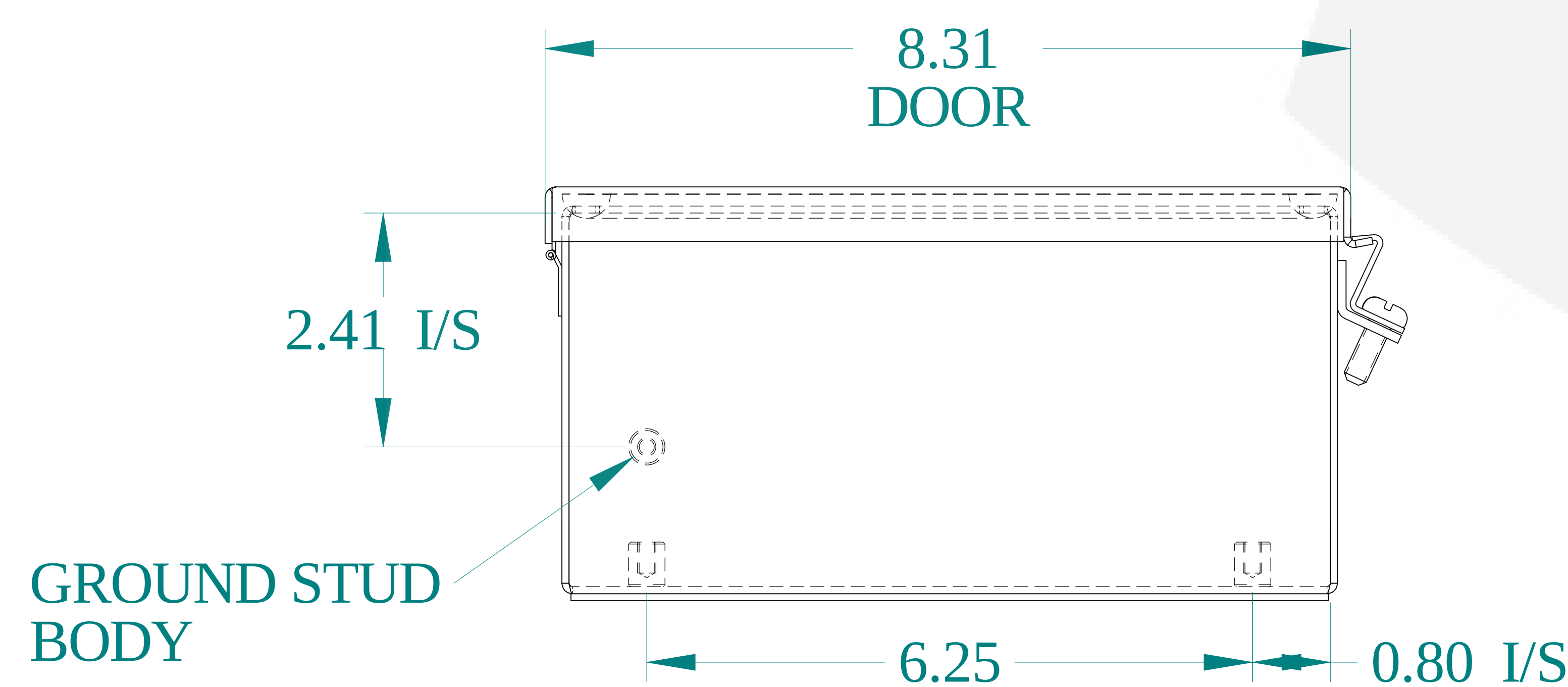
BOTTOM VIEW
