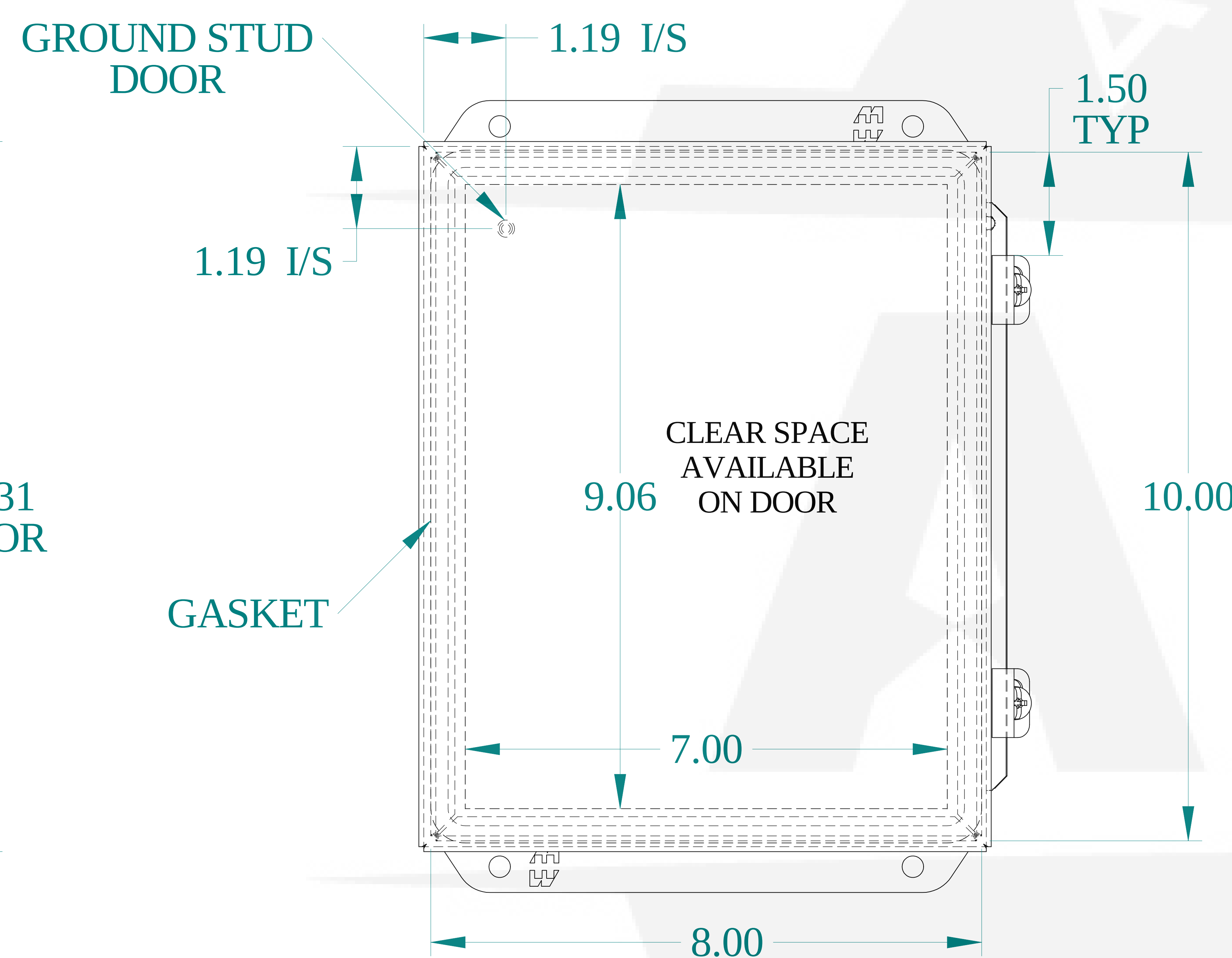
FRONT VIEW
