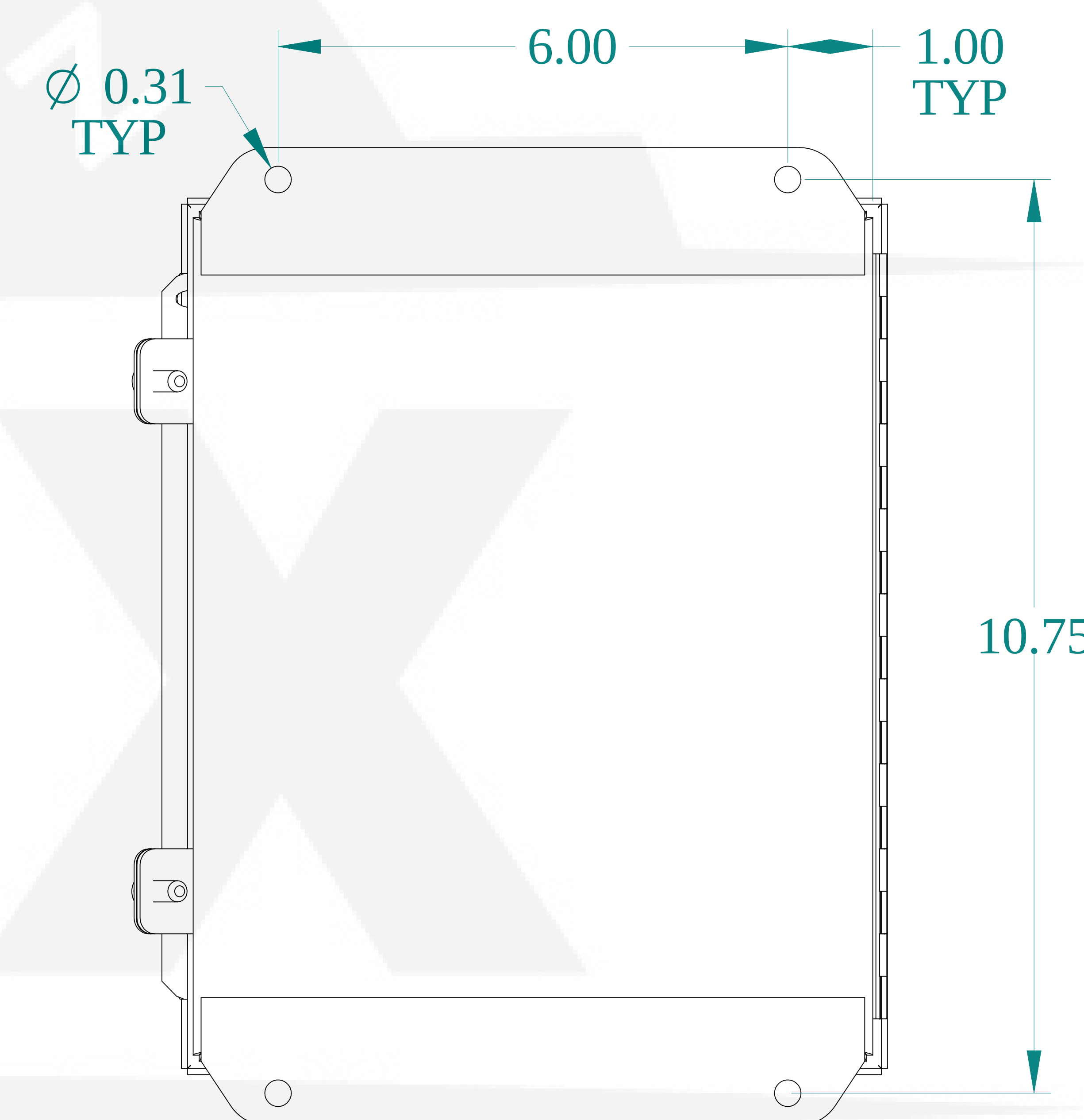
BACK VIEW
