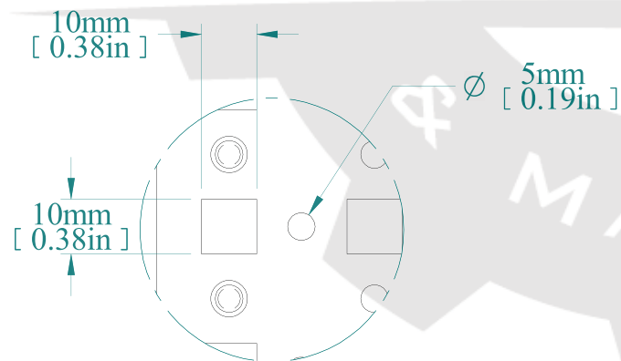
DETAIL A
