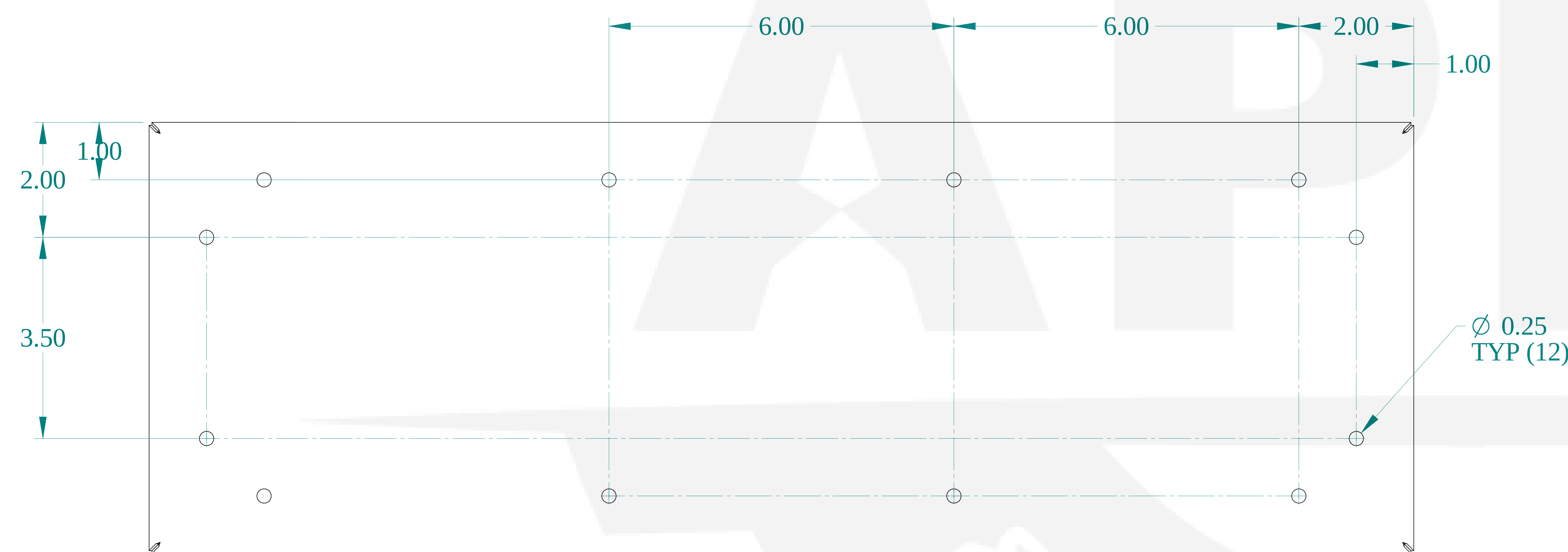
FRONT VIEW
