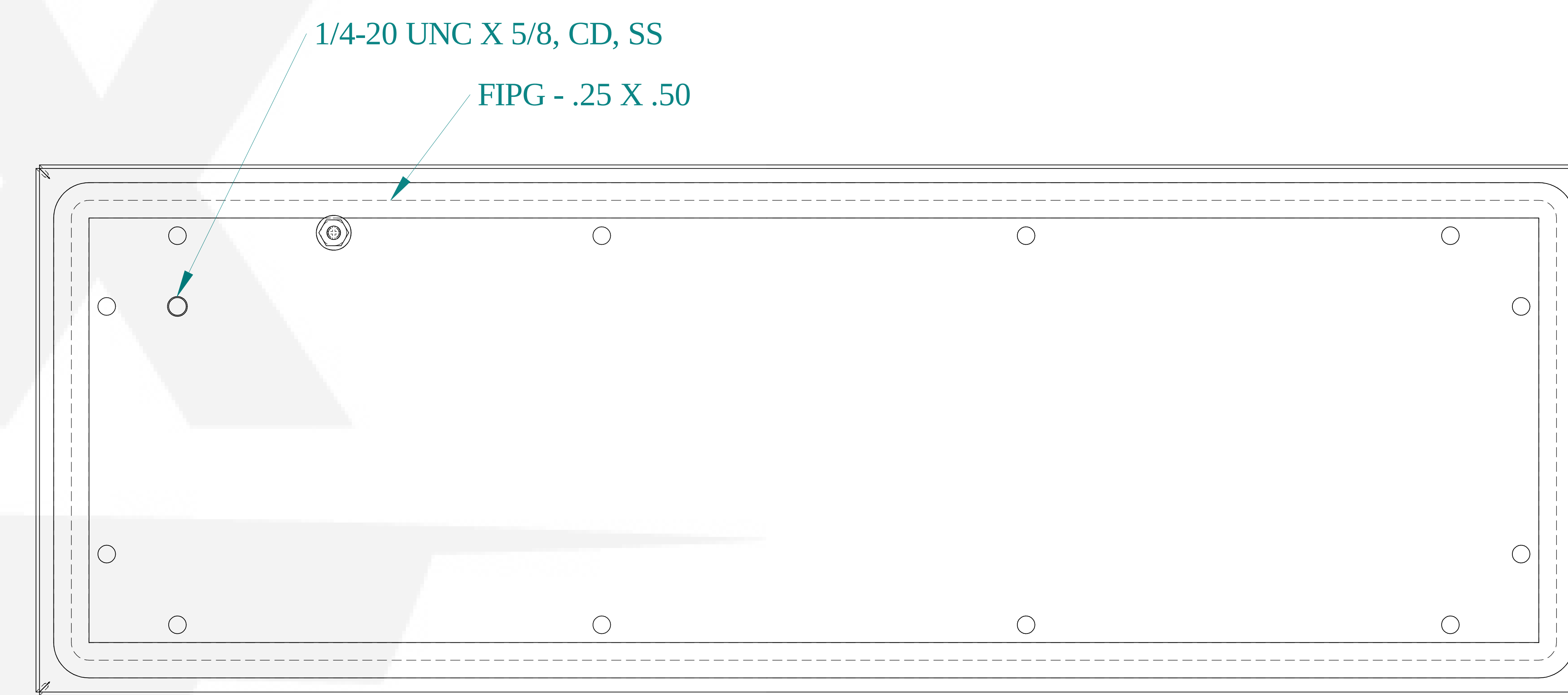
INSIDE VIEW
