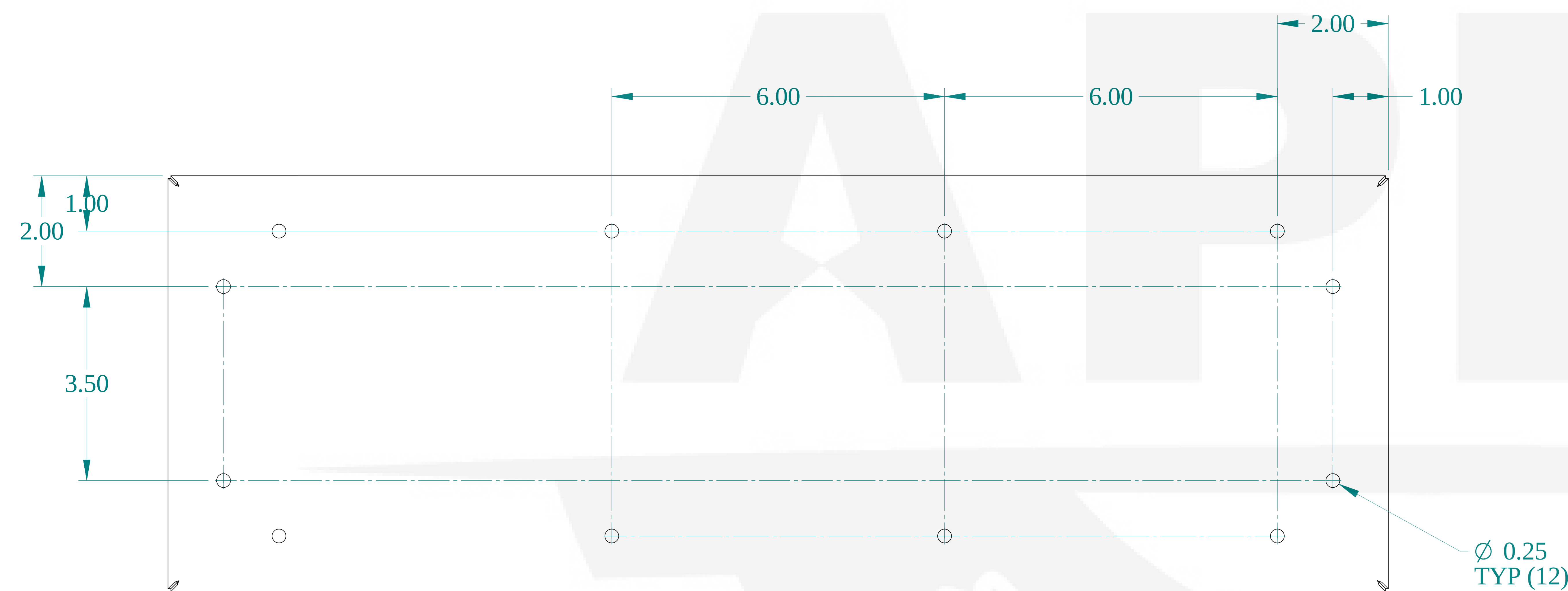
FRONT VIEW
