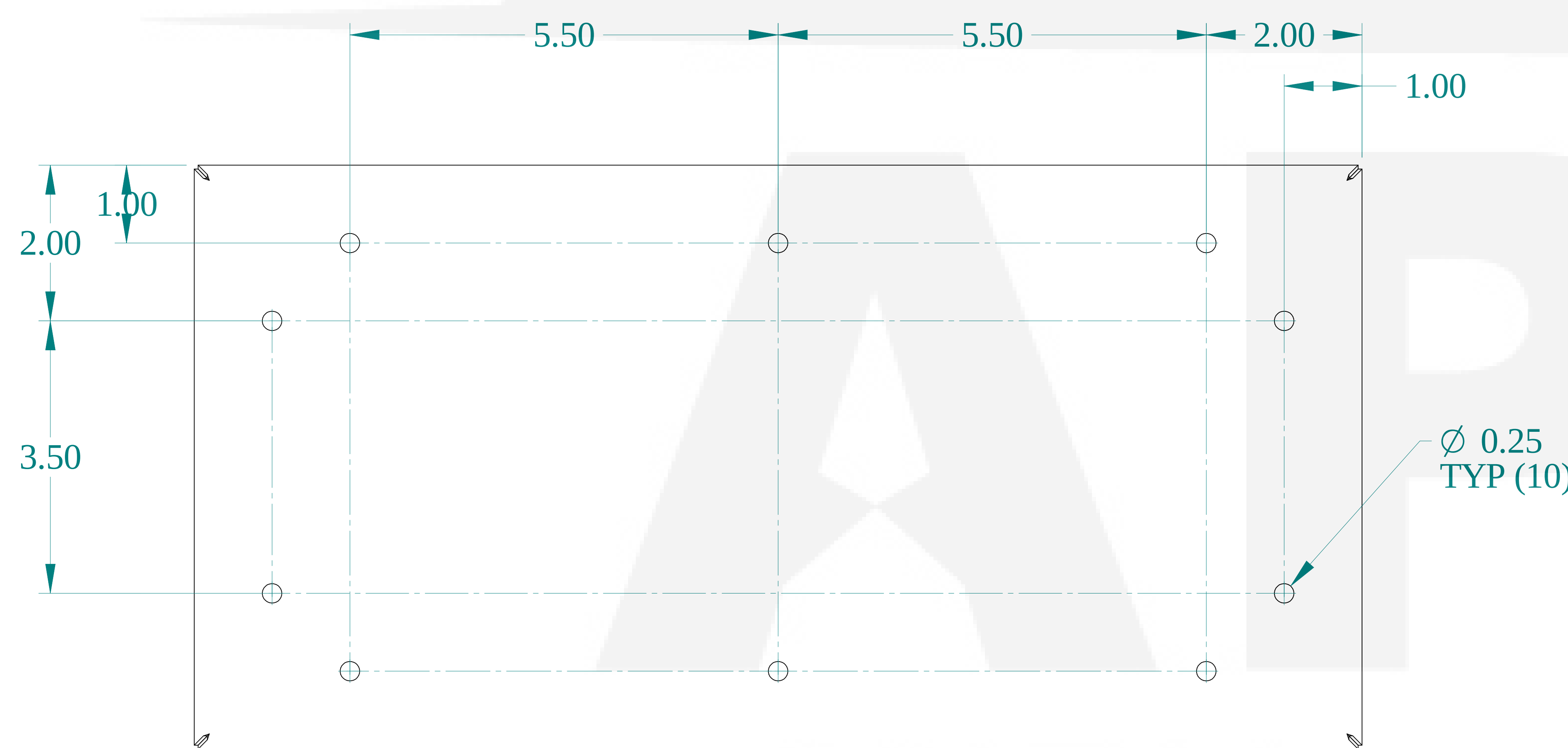
FRONT VIEW
