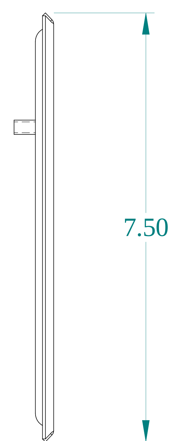
SIDE VIEW
