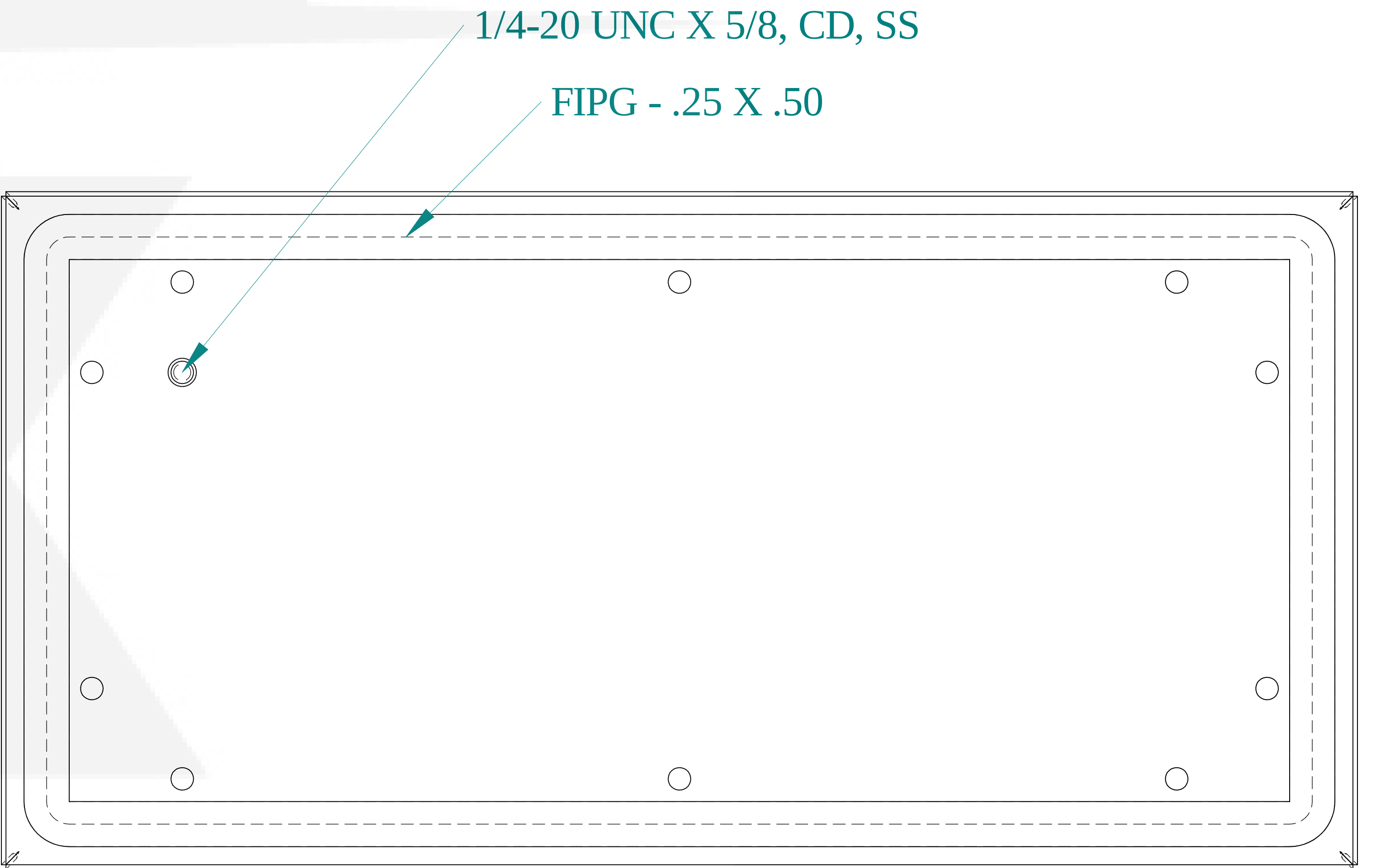
INSIDE VIEW
