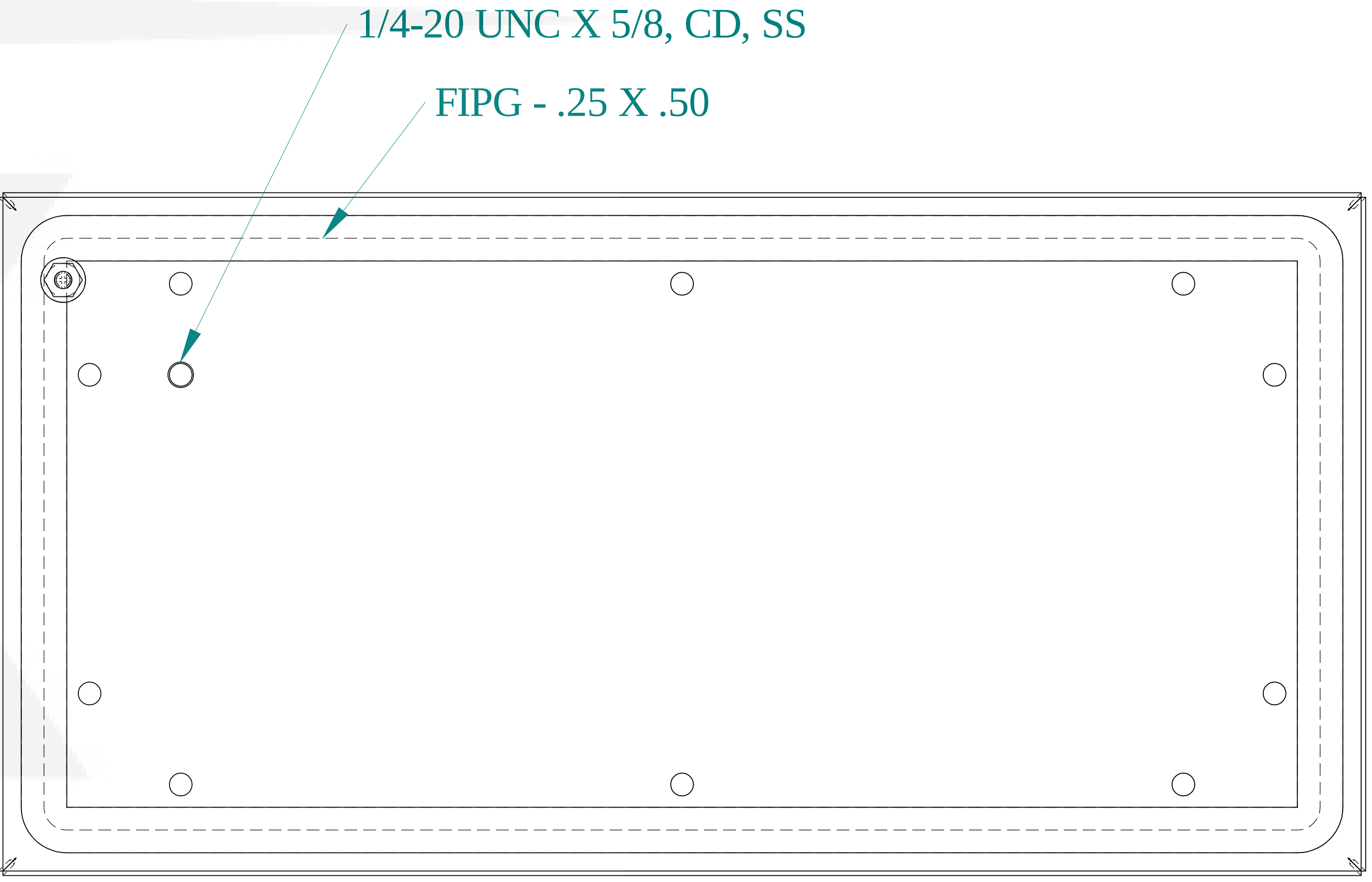
INSIDE VIEW
