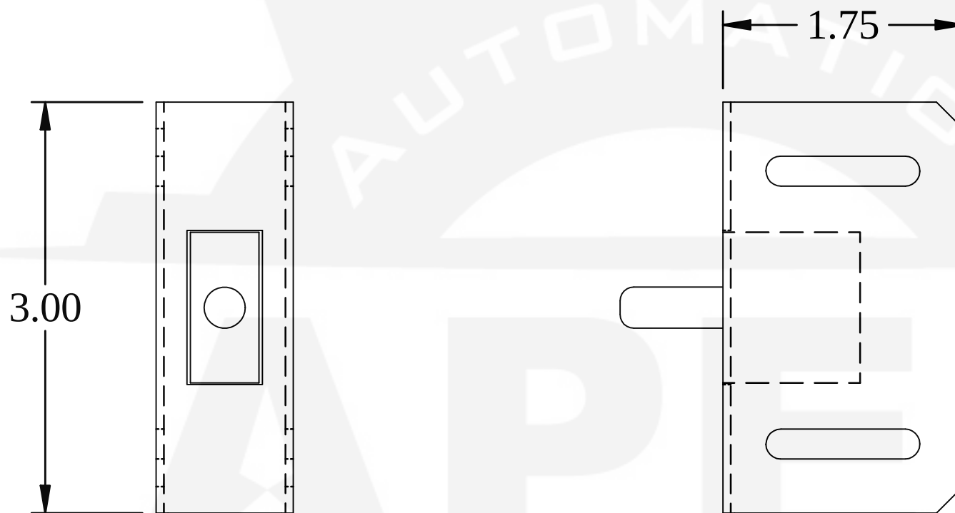
FRONT VIEW
