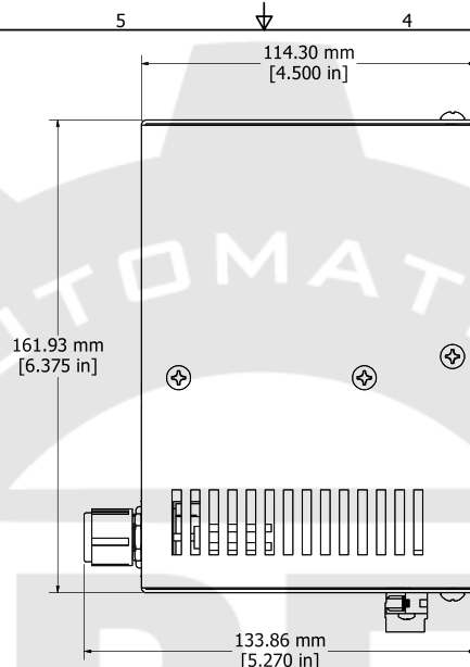
ASSEMBLY - VIEW FROM SIDE
