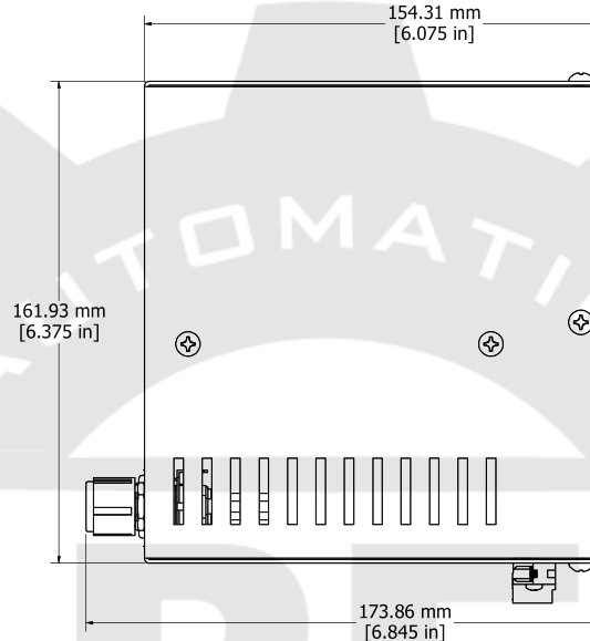
ASSEMBLY - VIEW FROM SIDE
