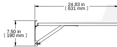
L.S. VIEW
