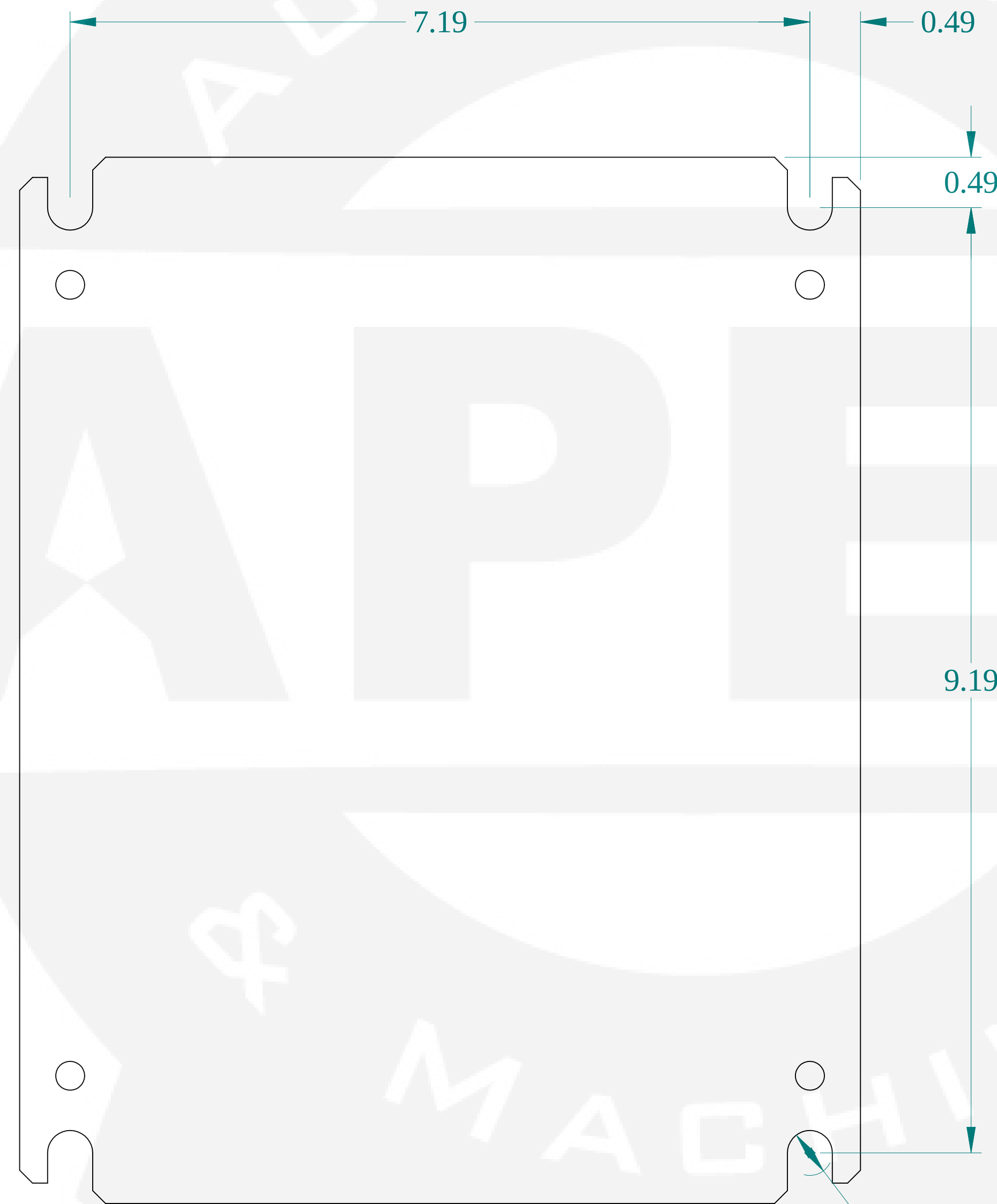
FRONT VIEW
