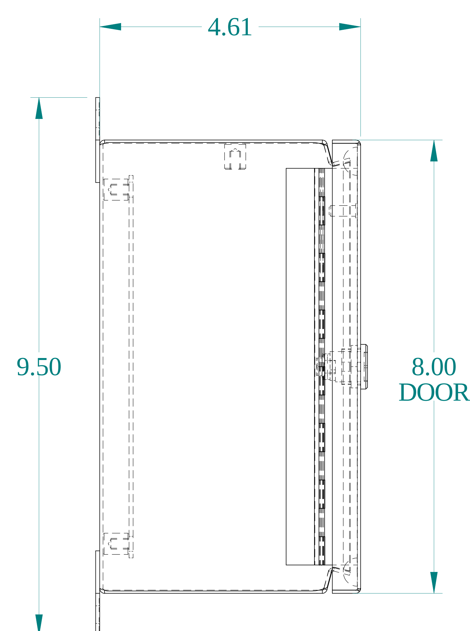
SIDE VIEW
