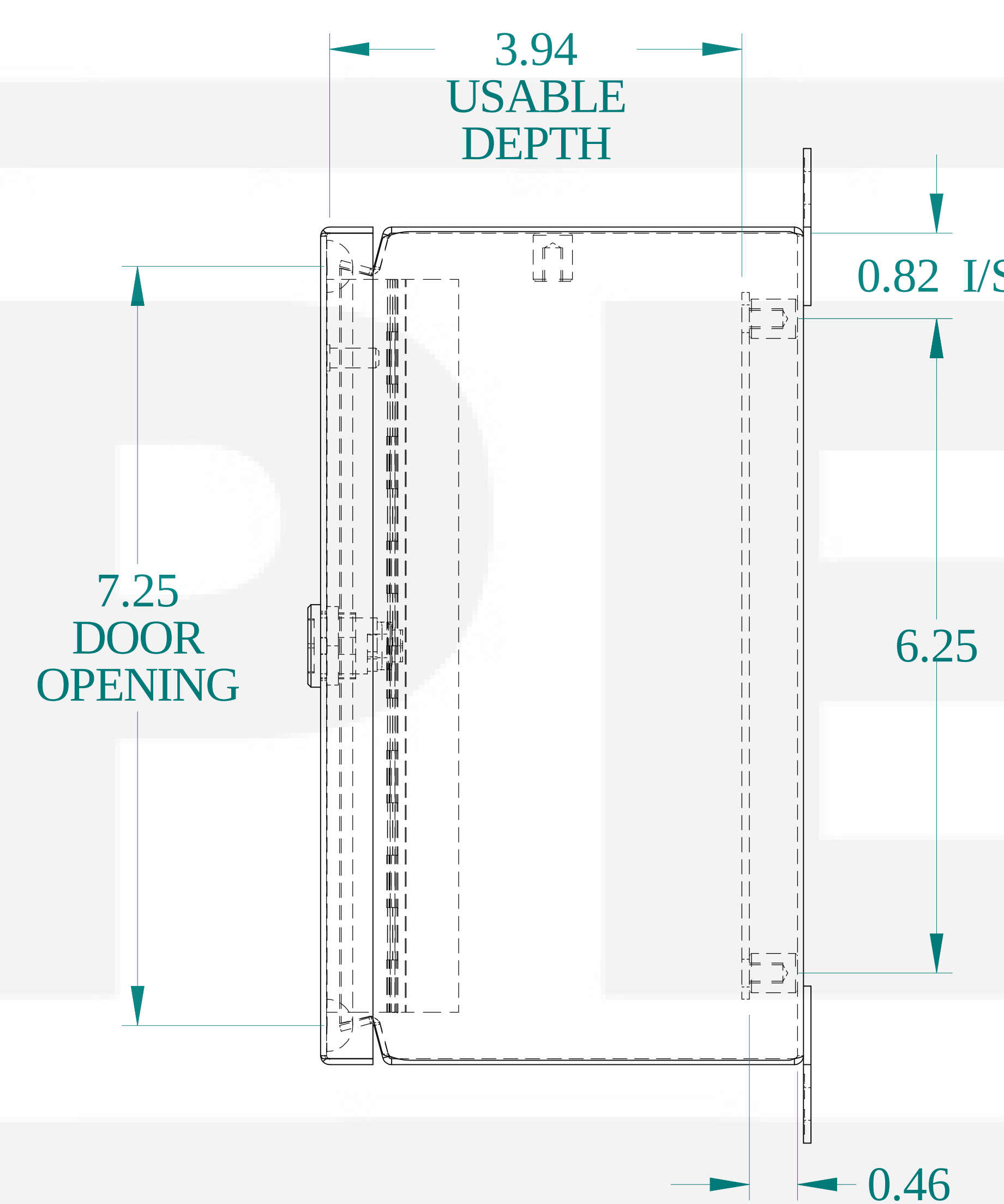
SIDE VIEW
