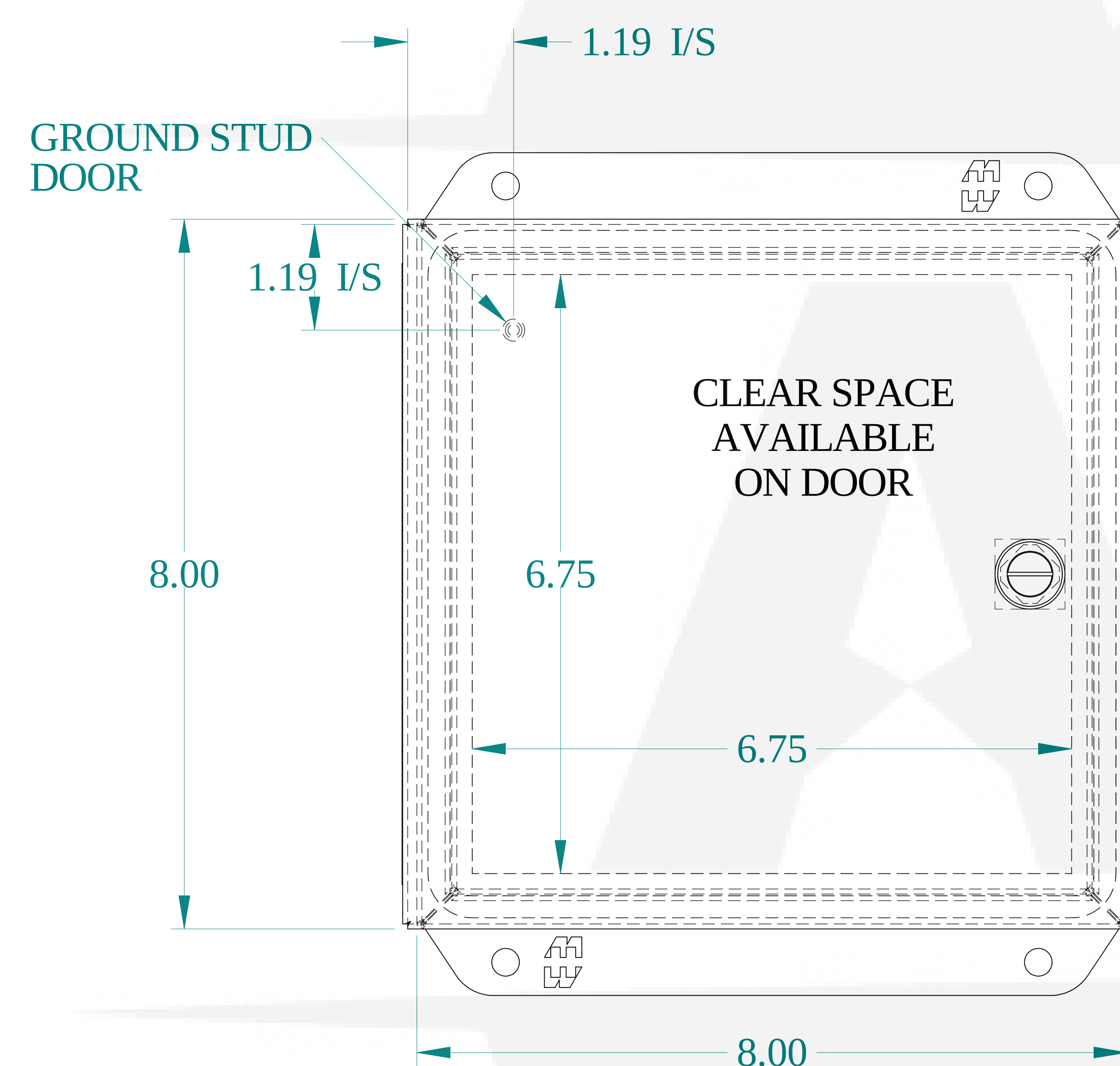
FRONT VIEW
