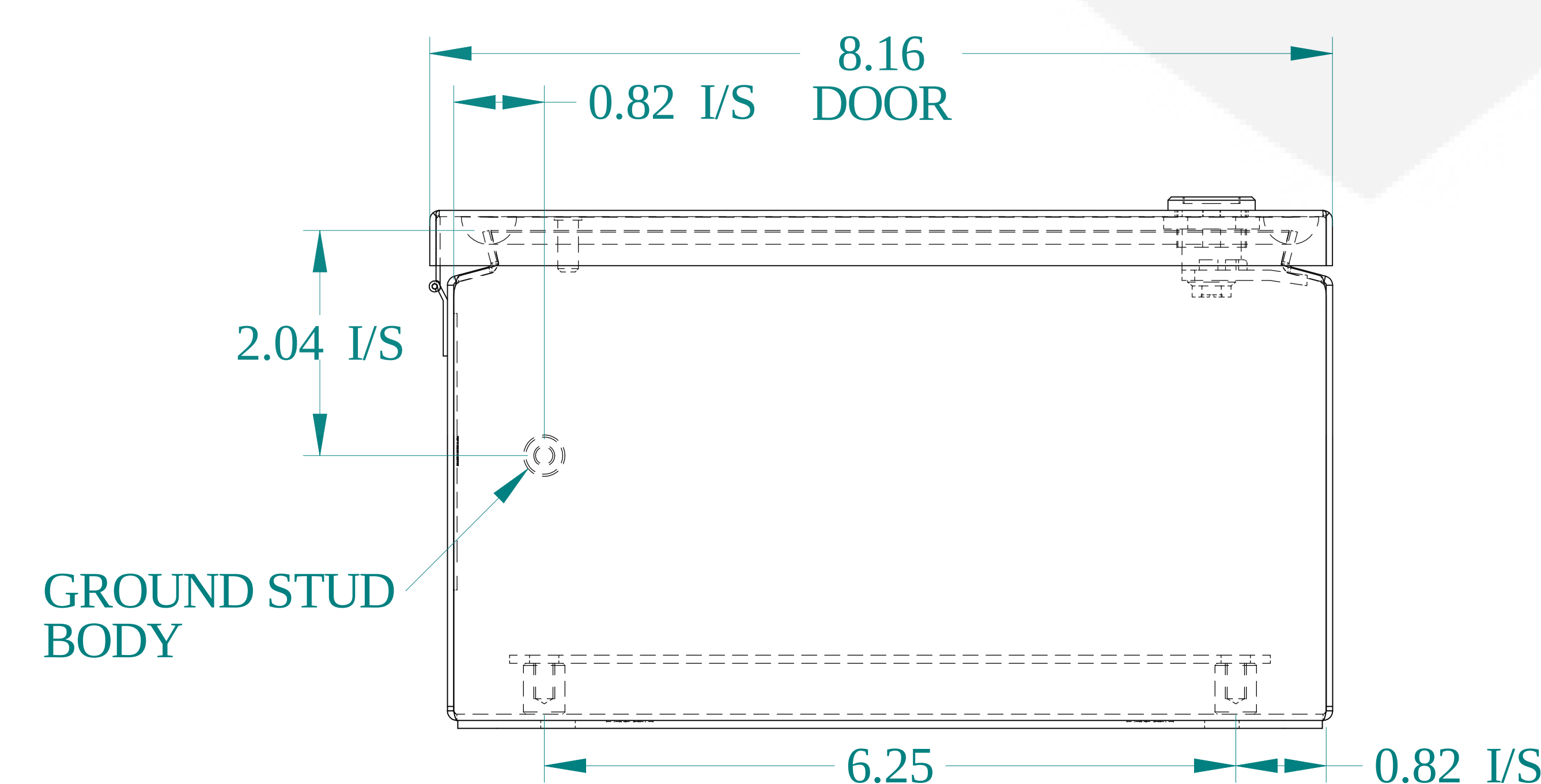
BOTTOM VIEW
