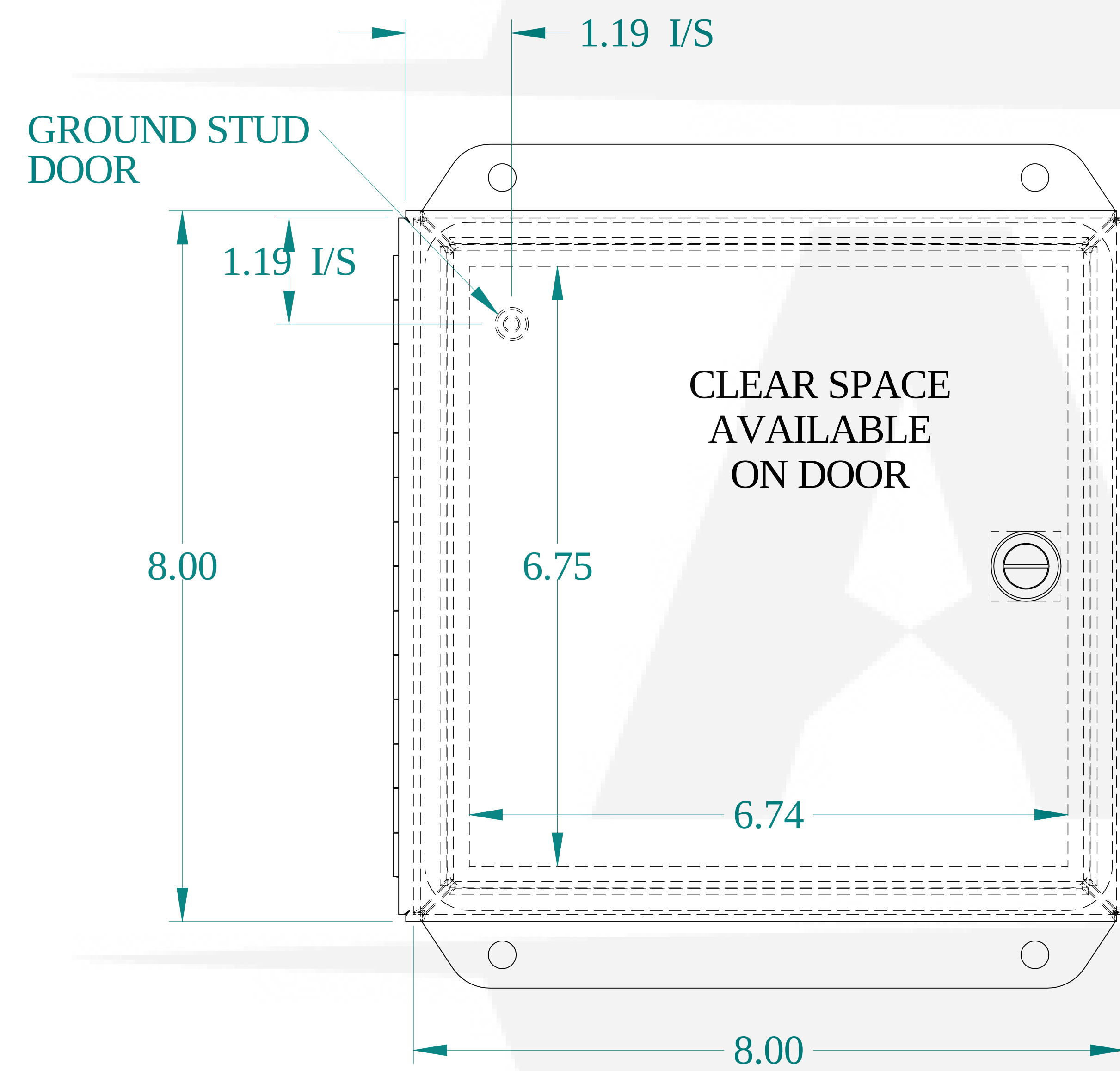
FRONT VIEW
