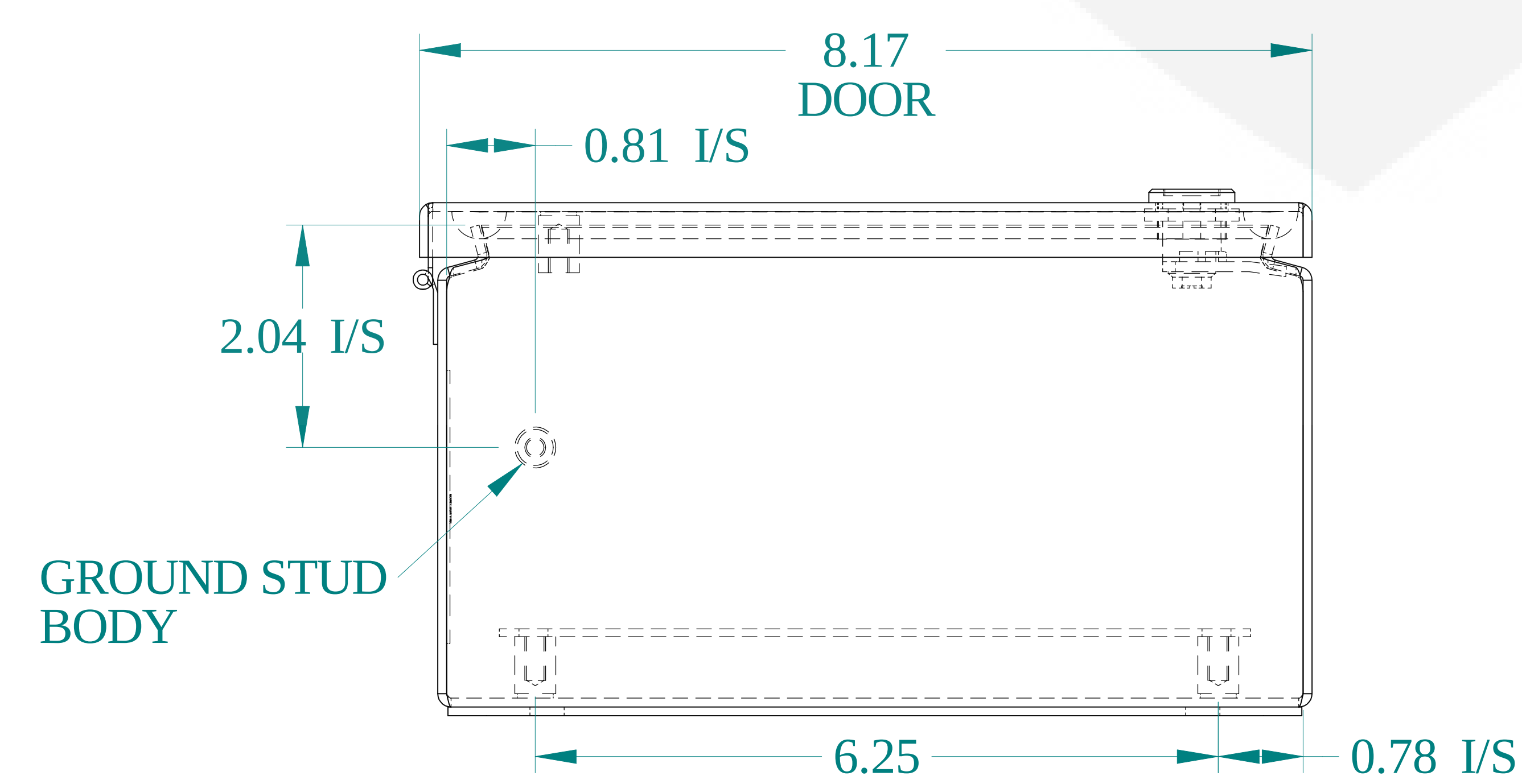
BOTTOM VIEW
