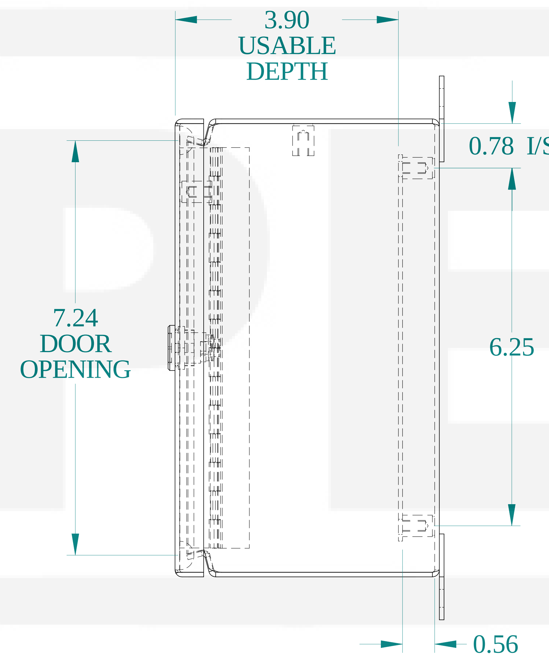
SIDE VIEW
