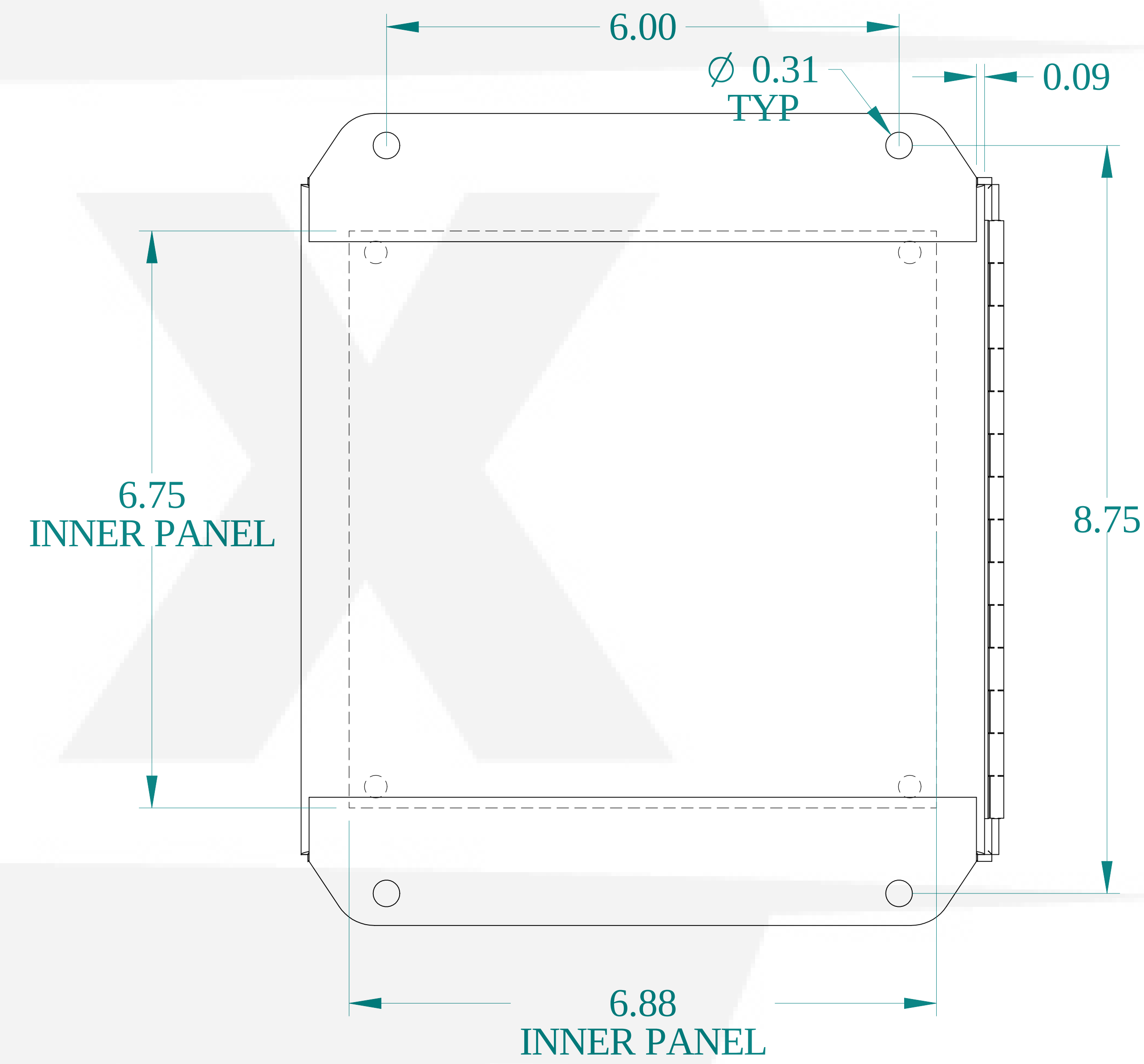
BACK VIEW
