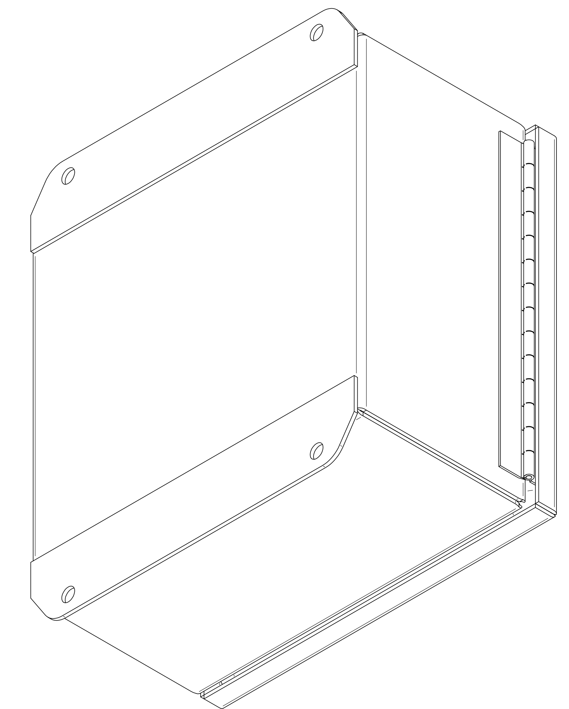
ISOMETRIC VIEWS
