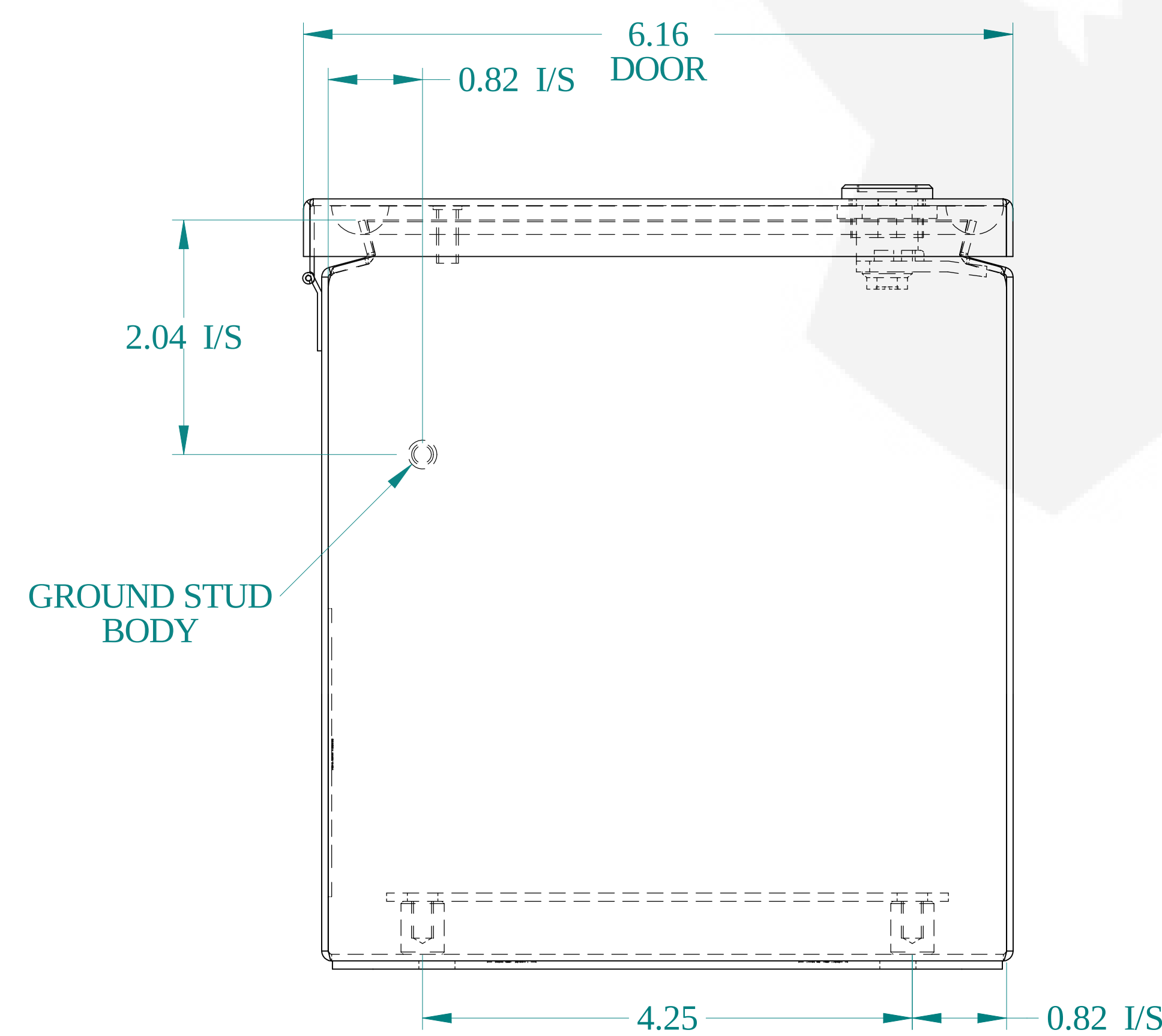
BOTTOM VIEW
