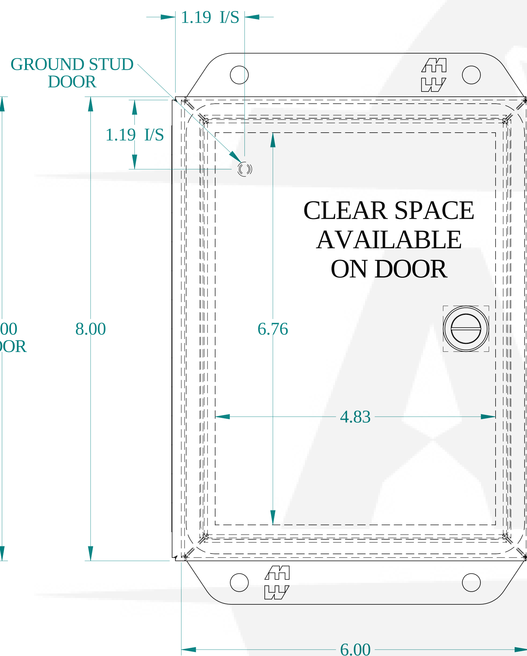
FRONT VIEW
