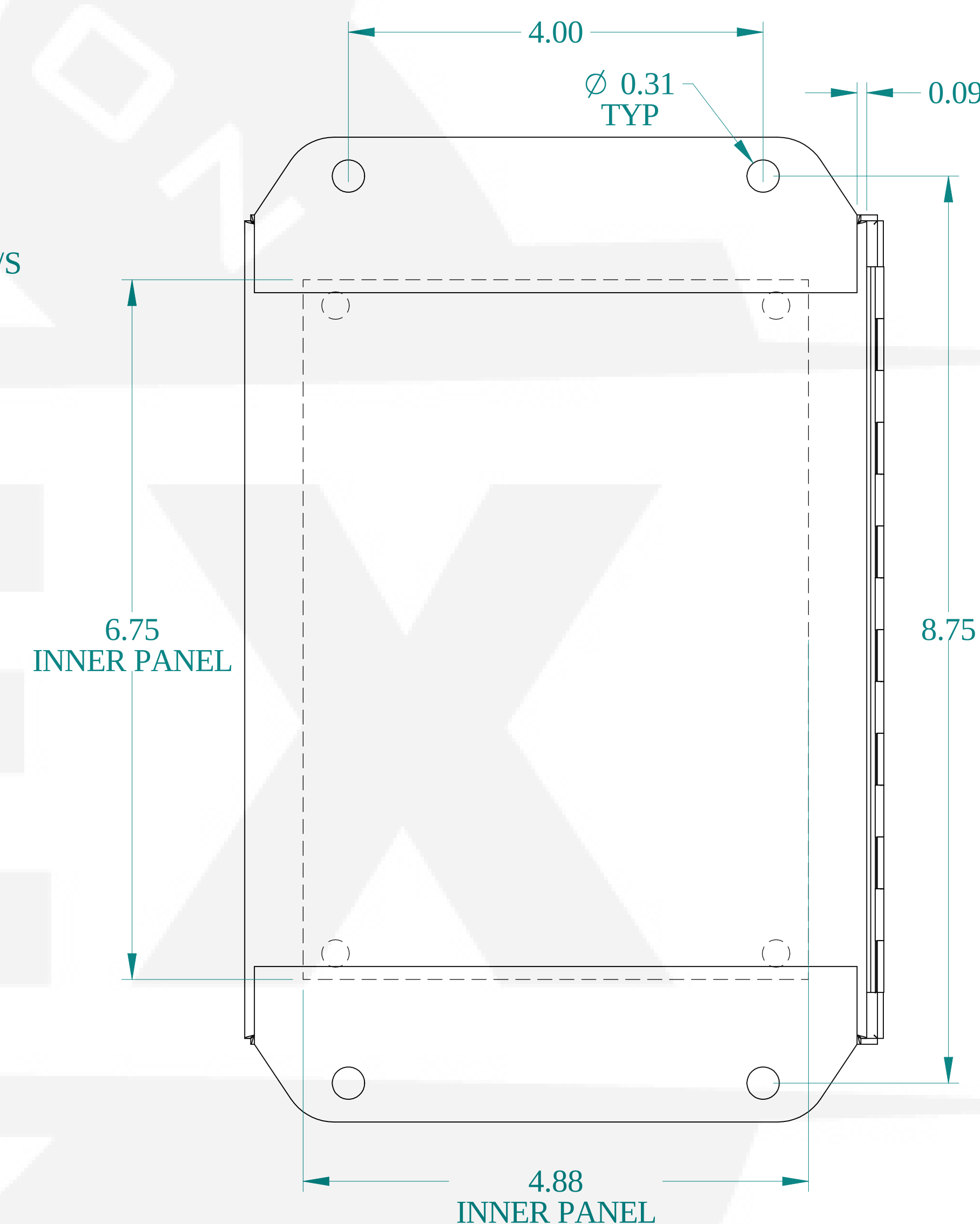
BACK VIEW
