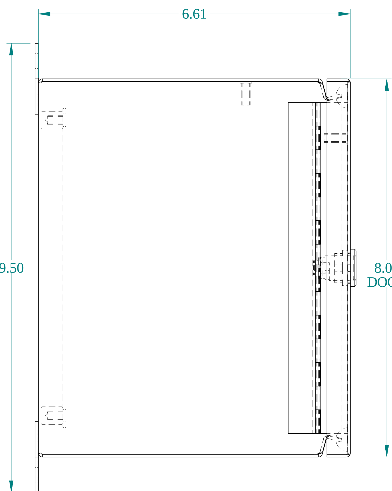
SIDE VIEW
