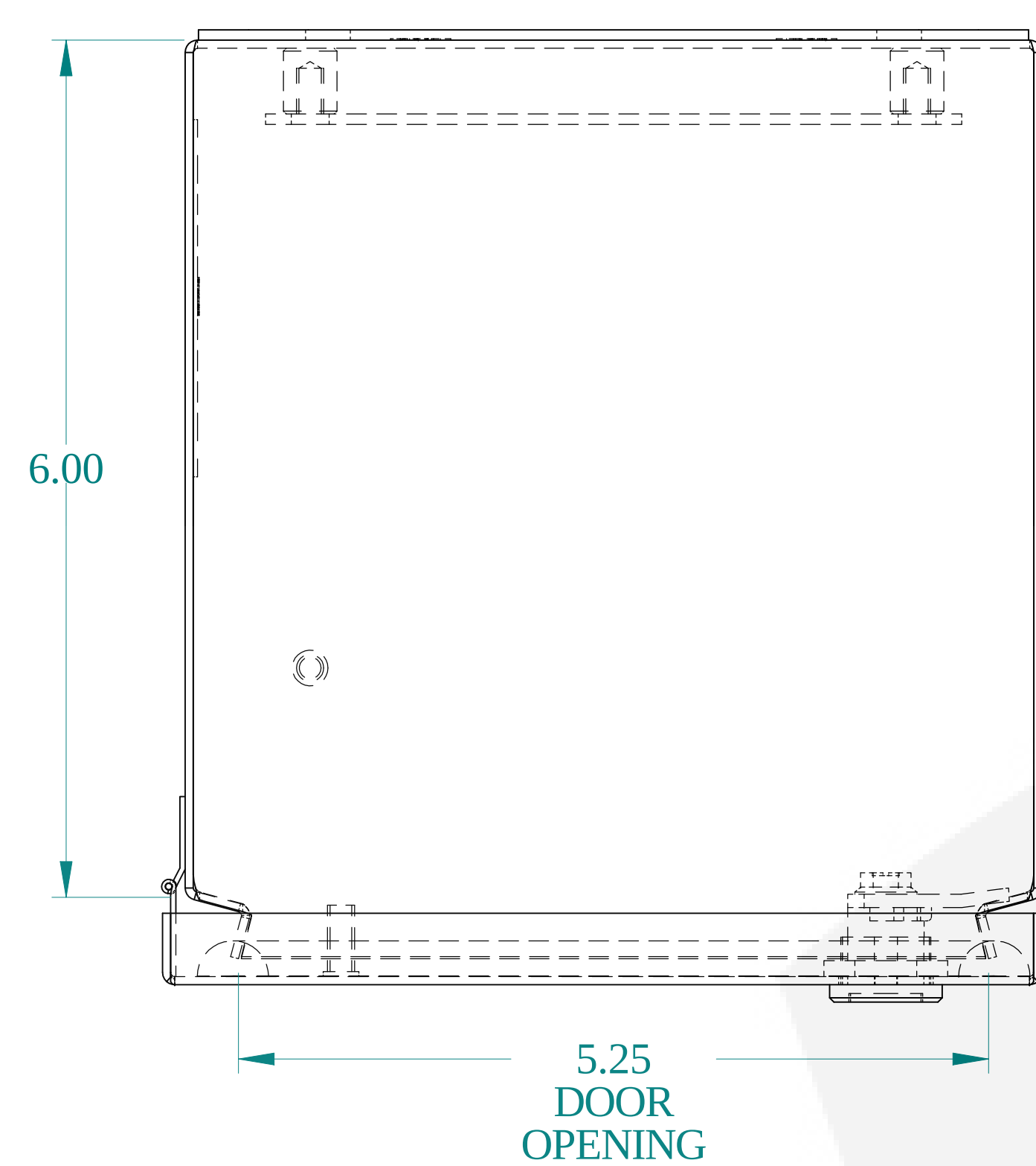
TOP VIEW
