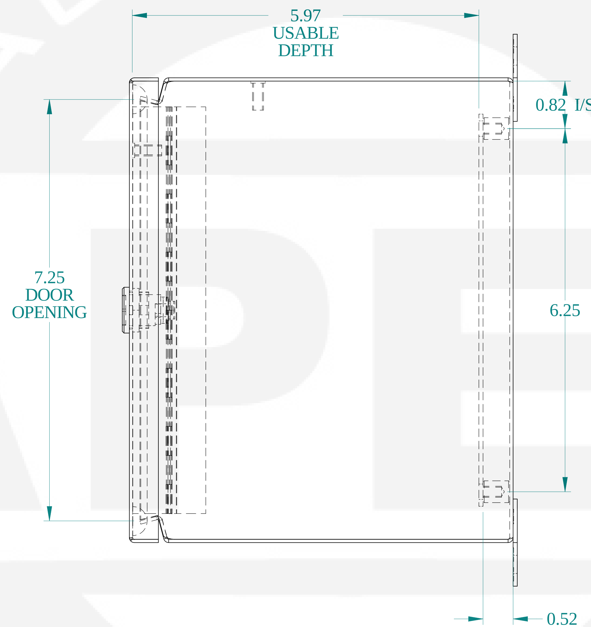
SIDE VIEW
