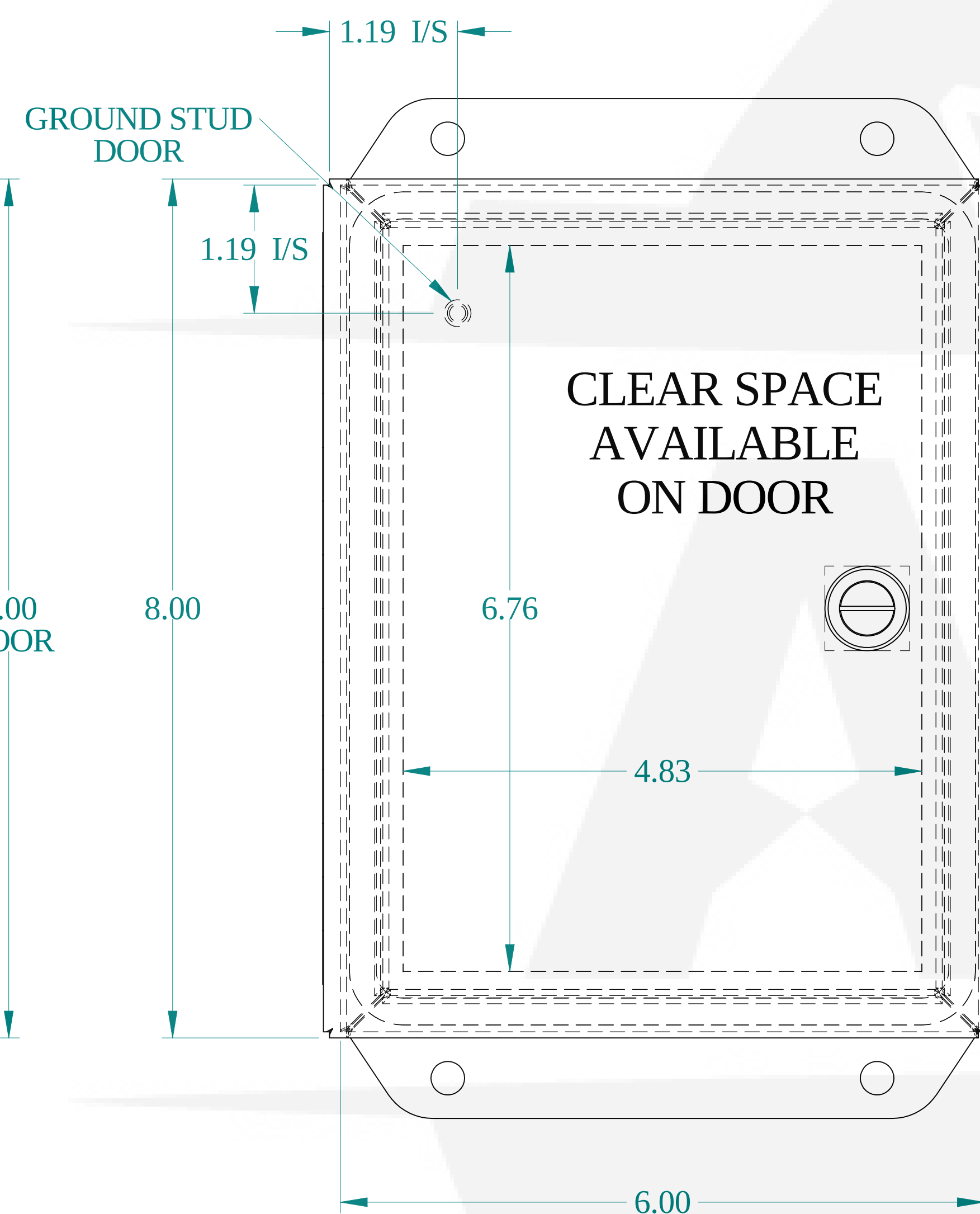
FRONT VIEW
