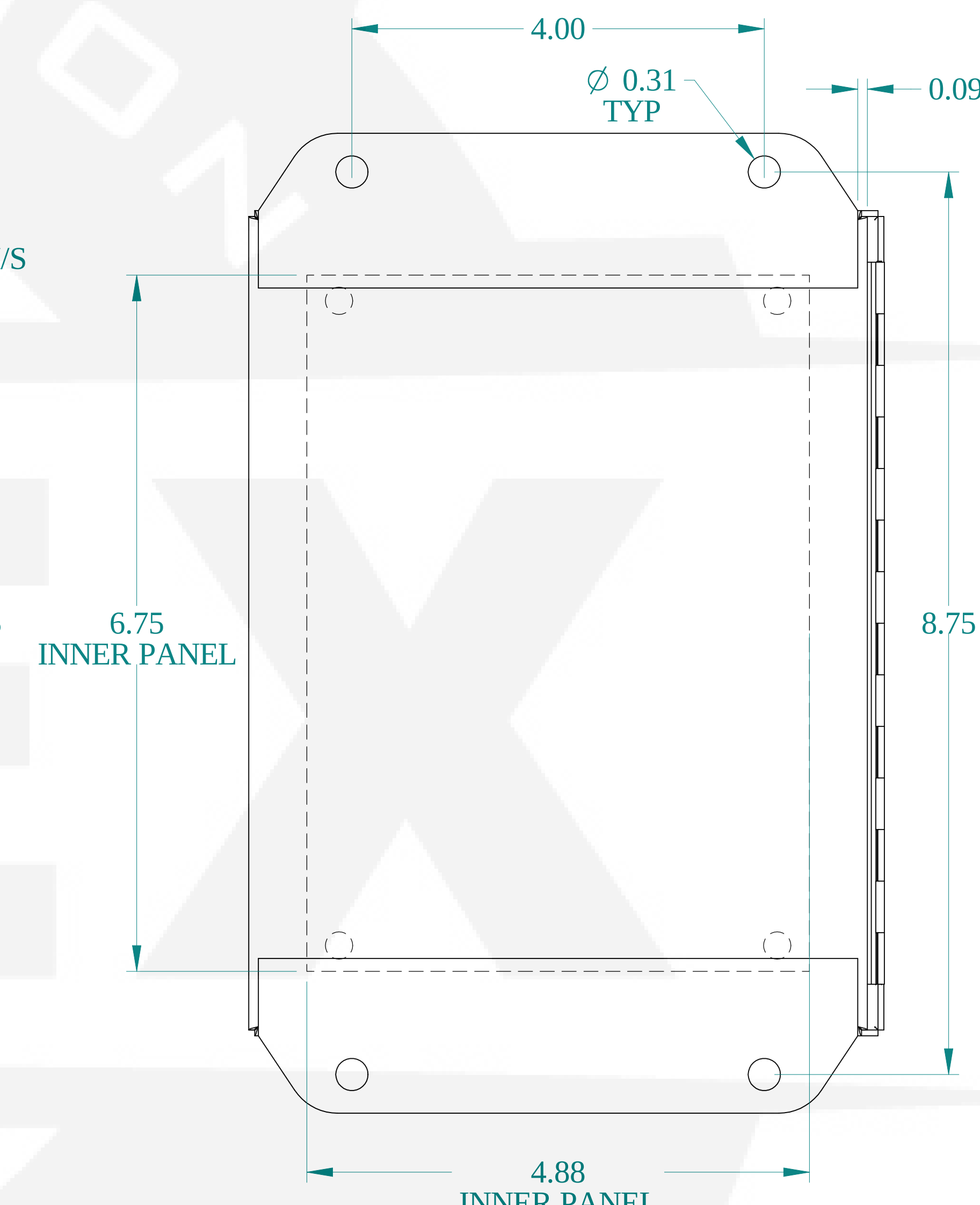
BACK VIEW
