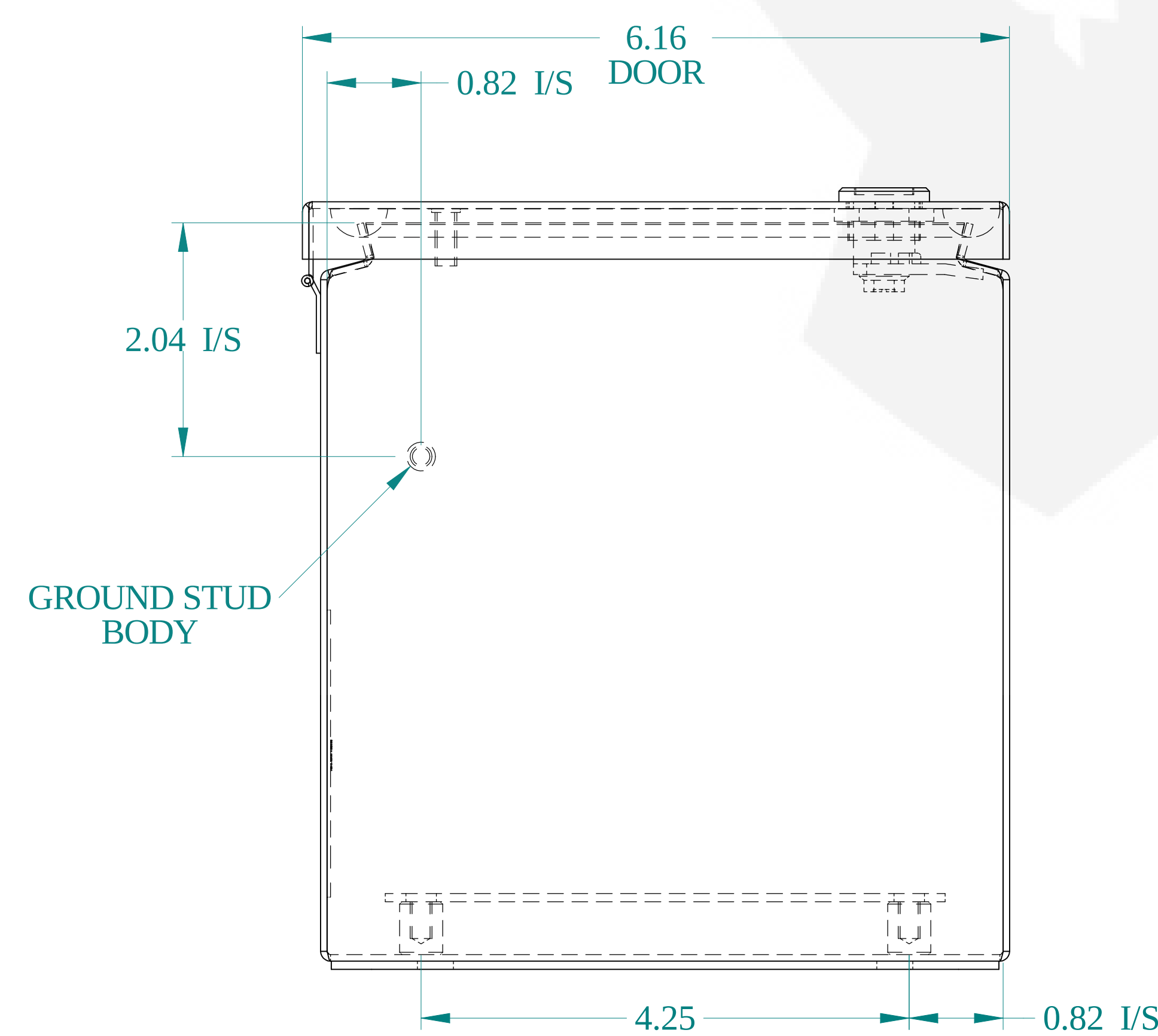
BOTTOM VIEW
