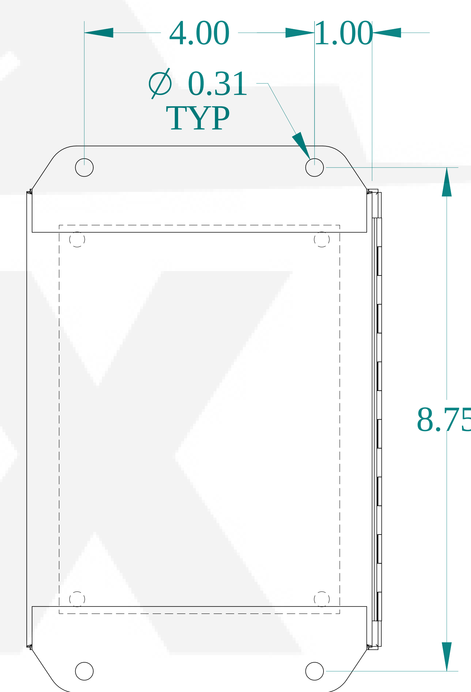
BACK VIEW
