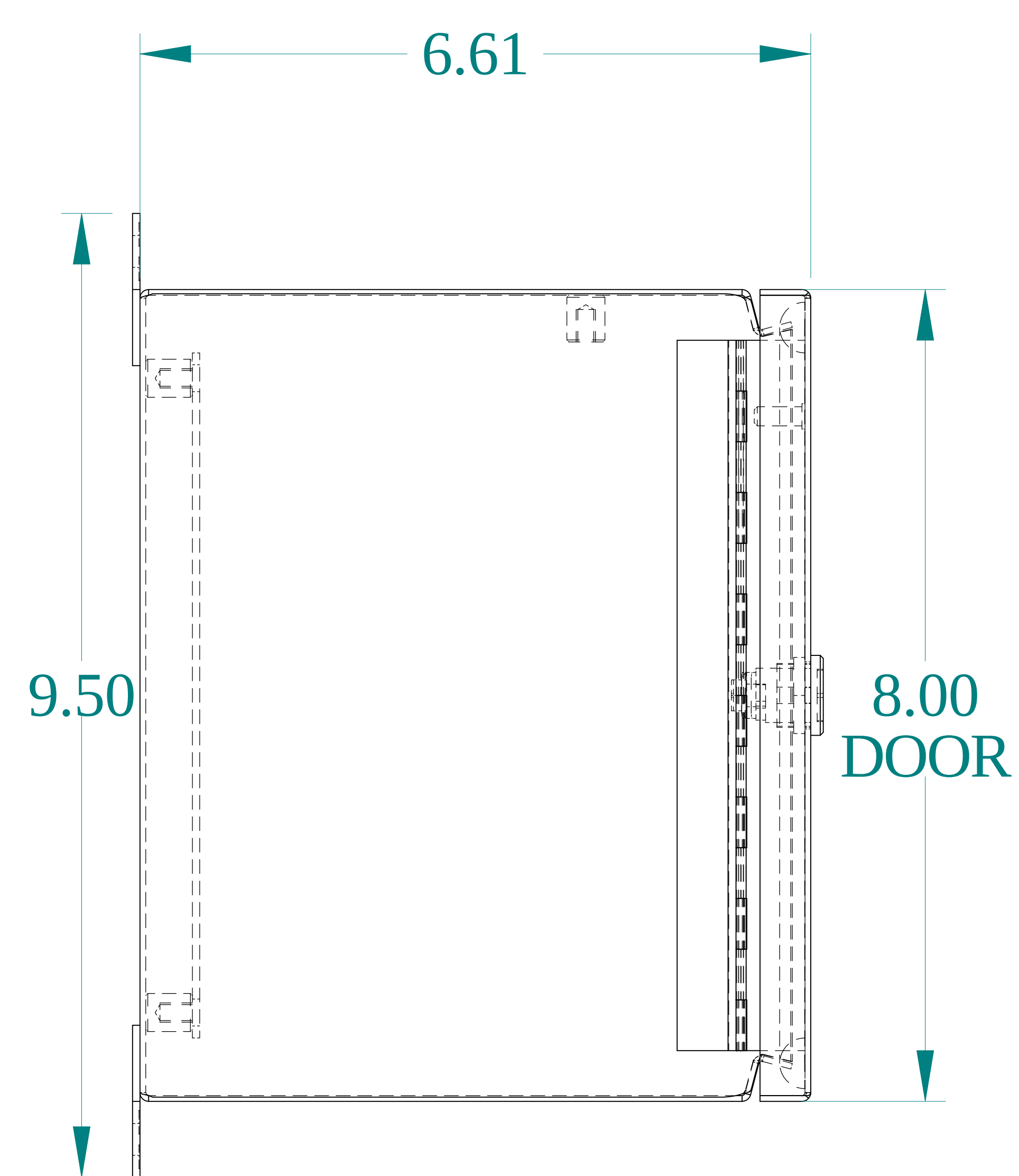
SIDE VIEW
