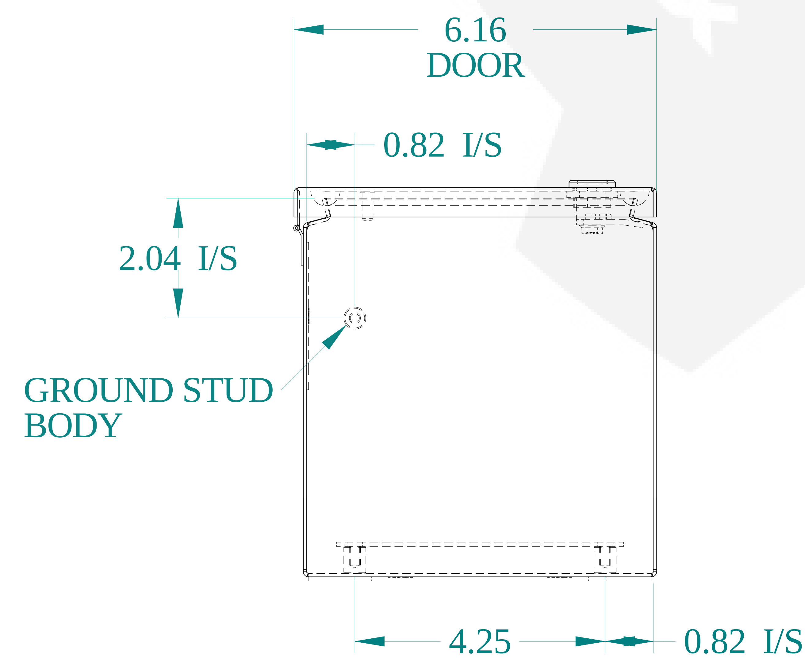
BOTTOM VIEW
