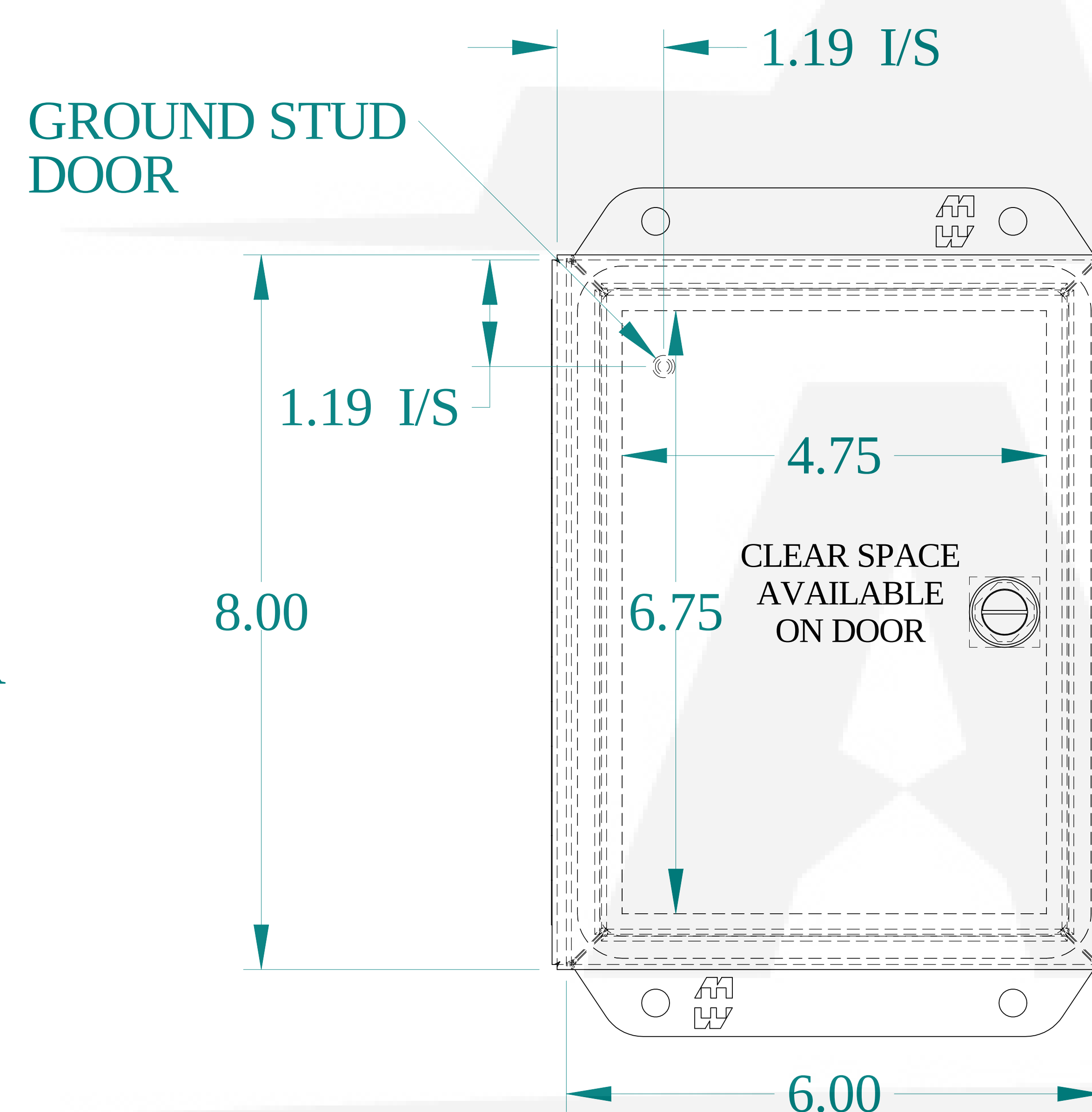
FRONT VIEW
