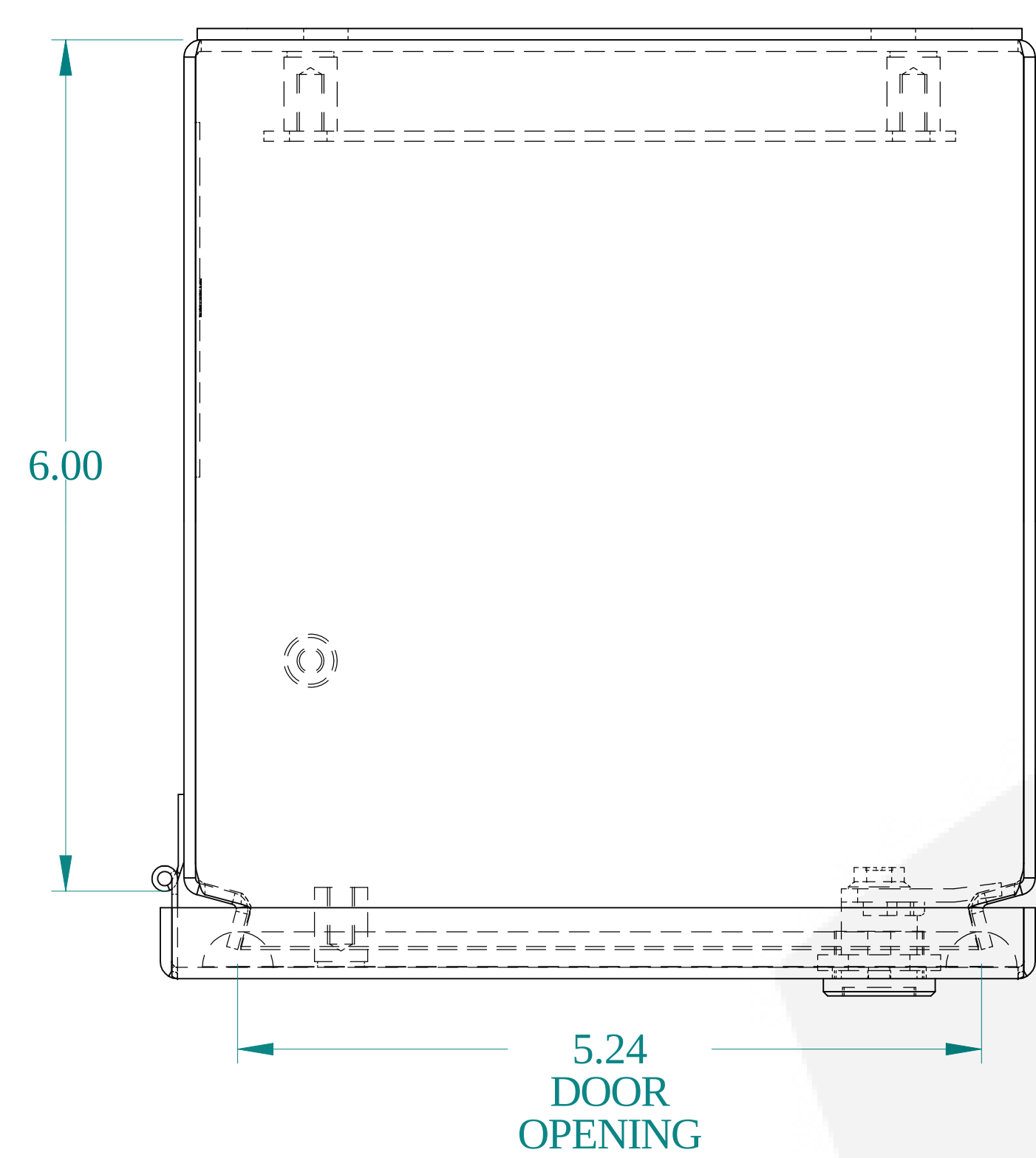
TOP VIEW
