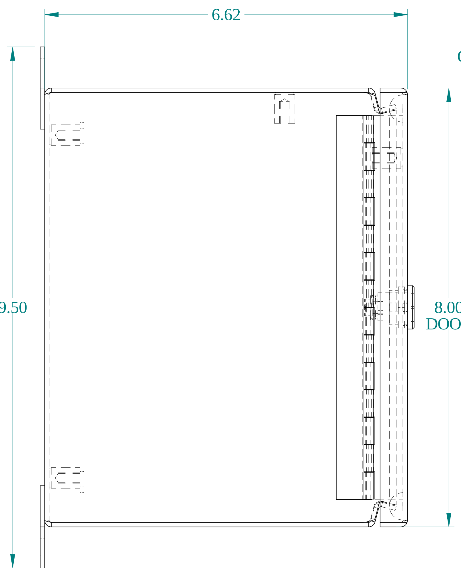
SIDE VIEW
