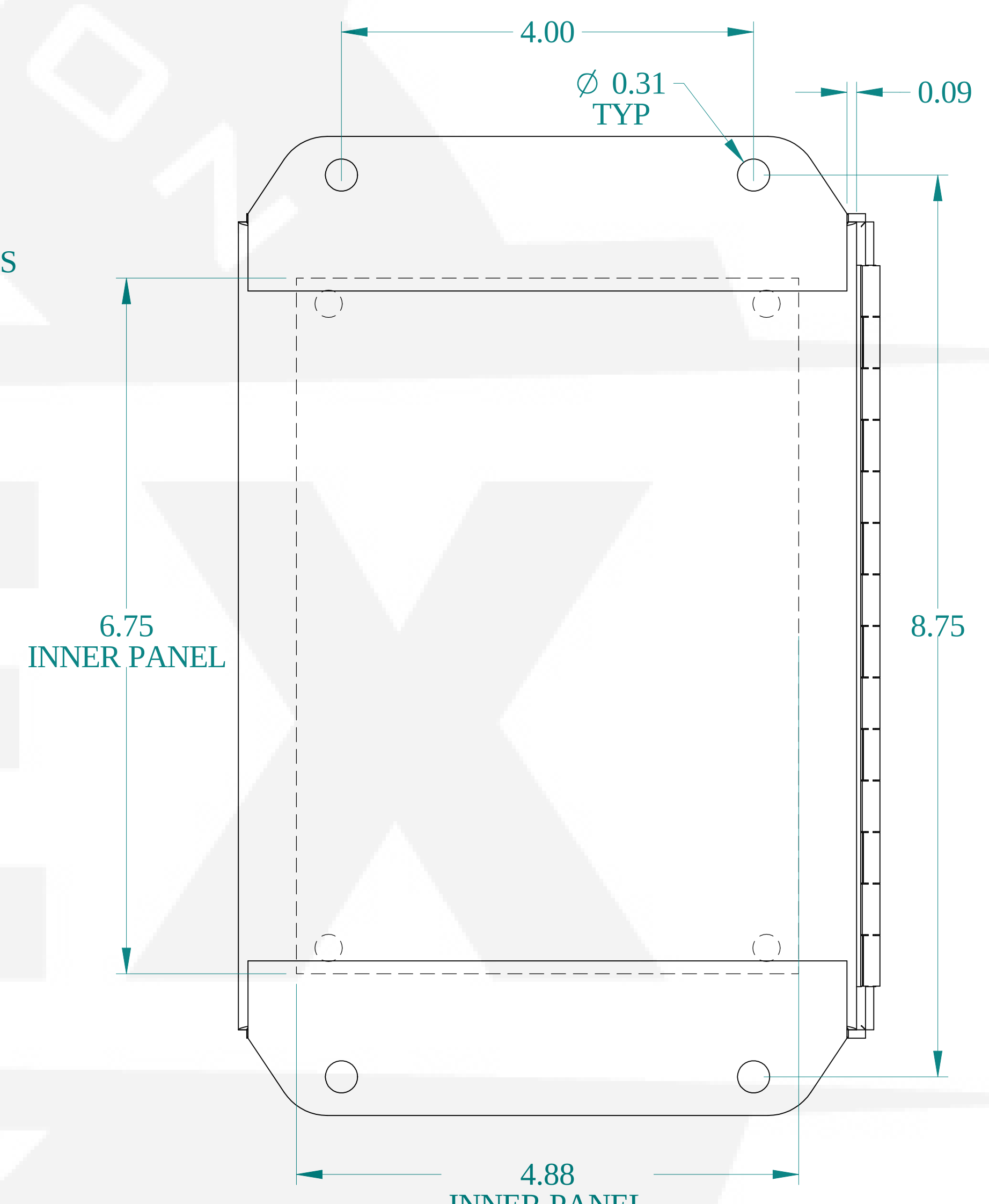
BACK VIEW
