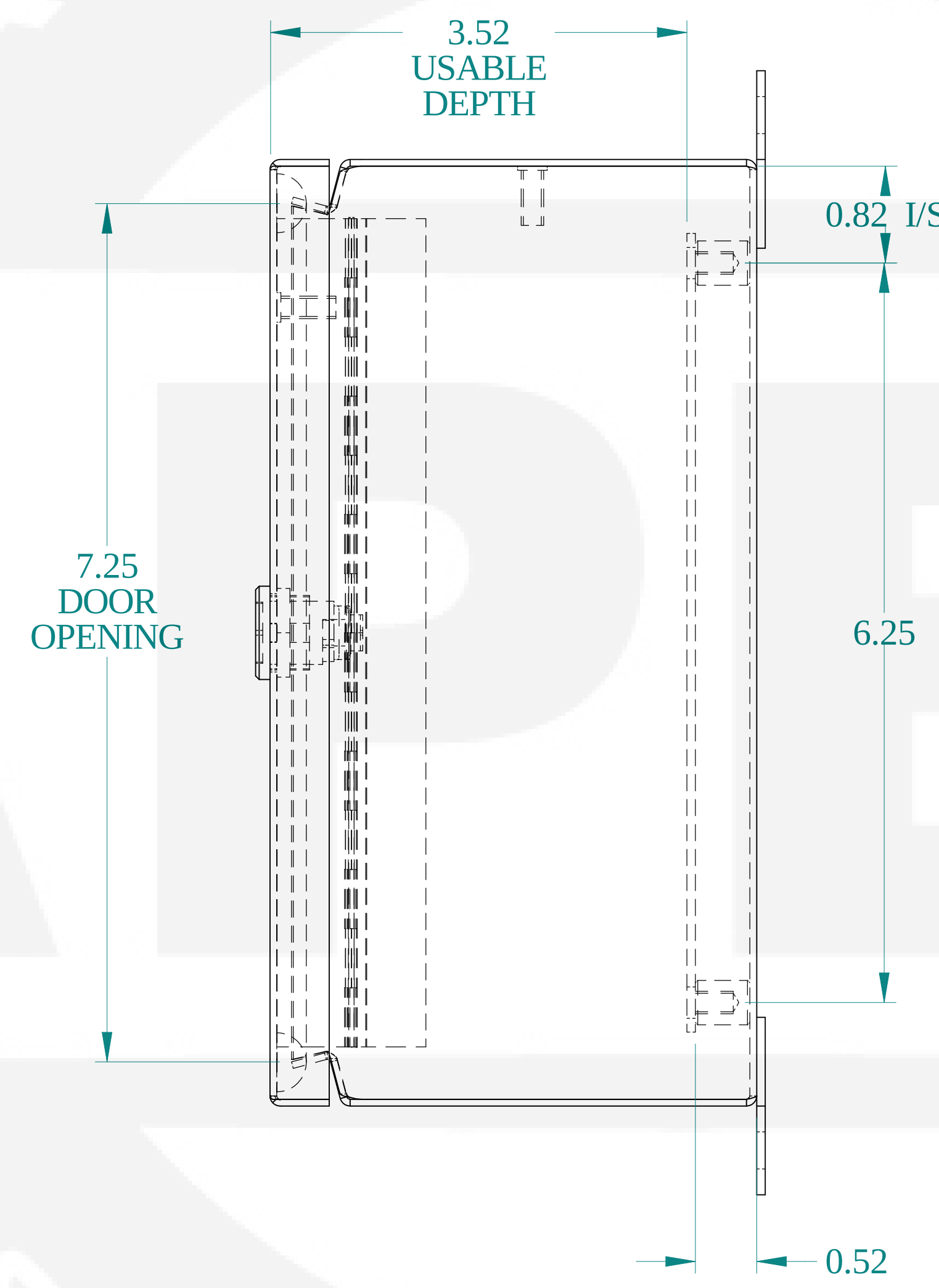
SIDE VIEW
