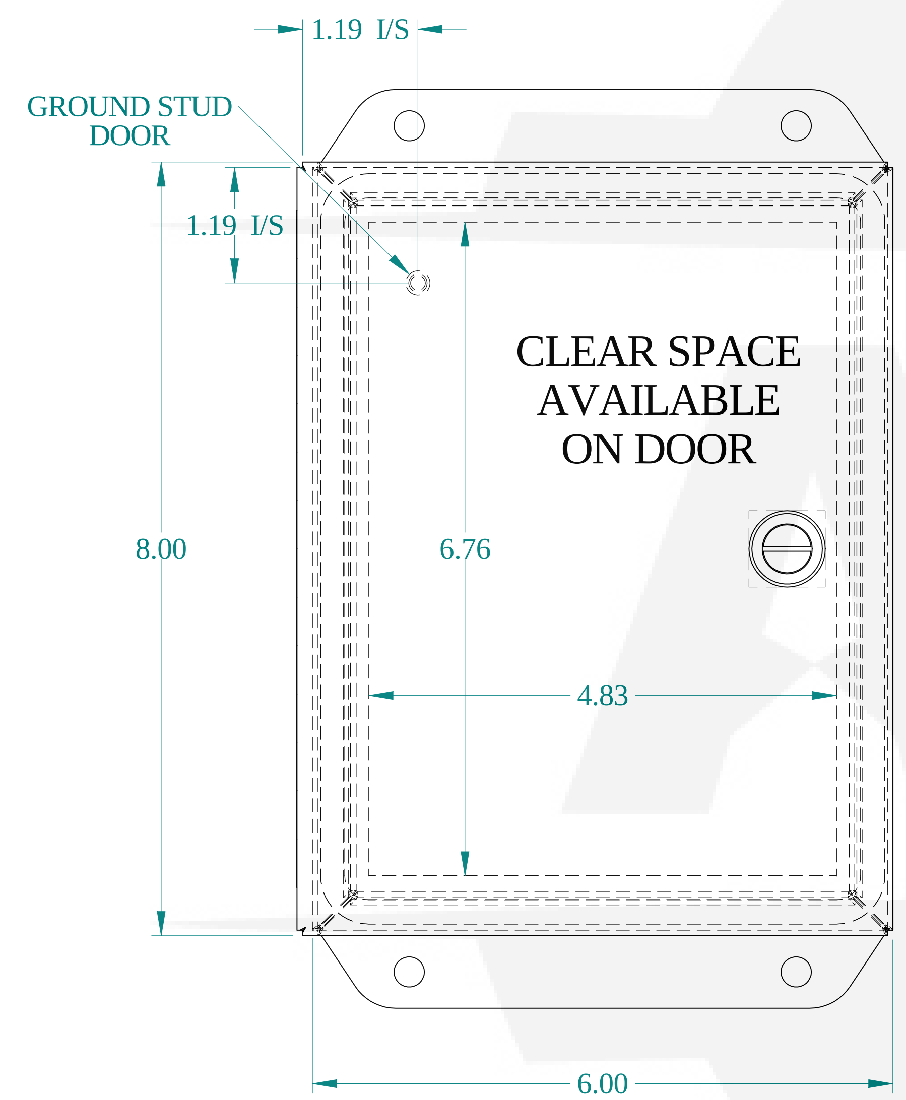
FRONT VIEW
