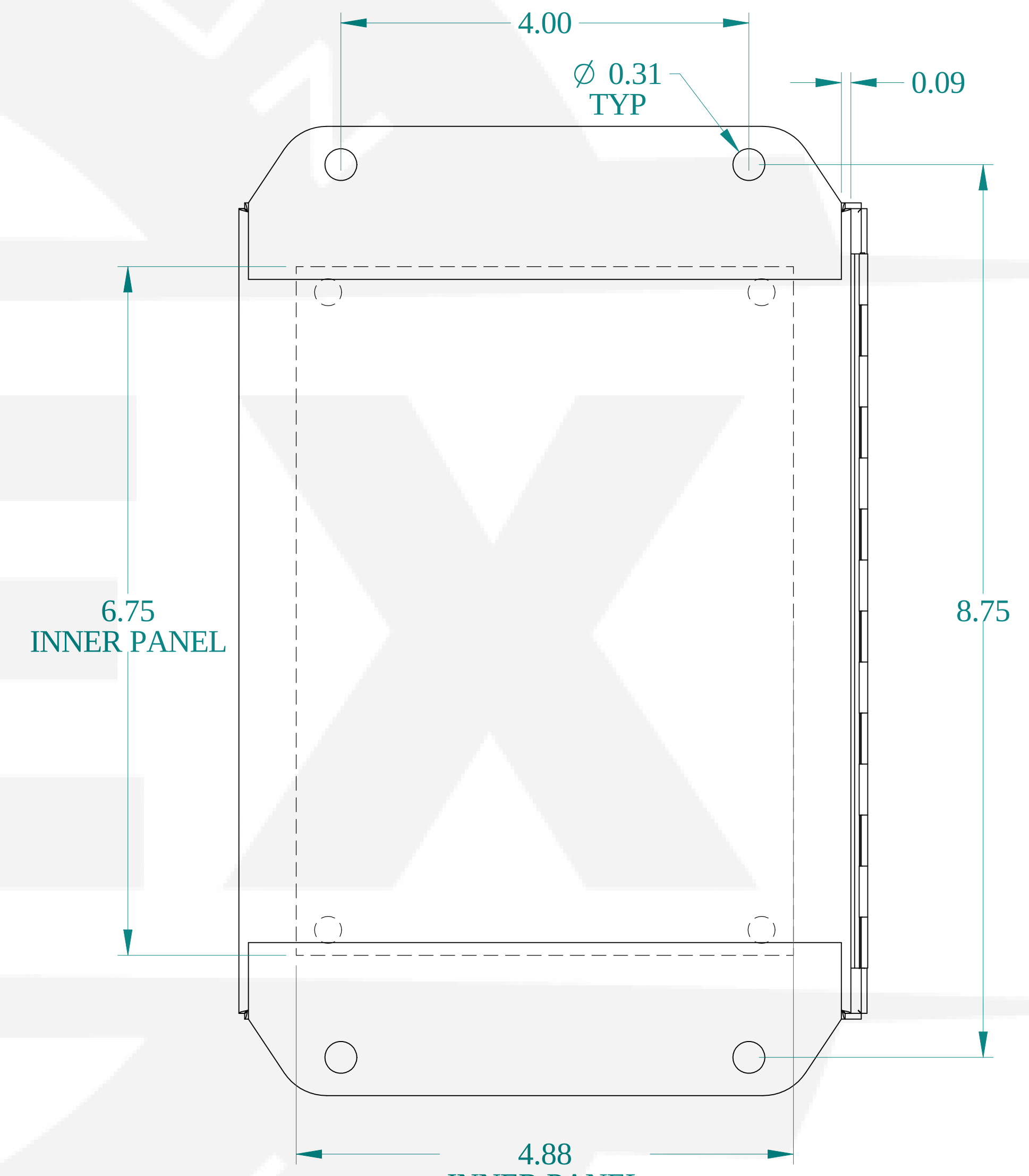
BACK VIEW
