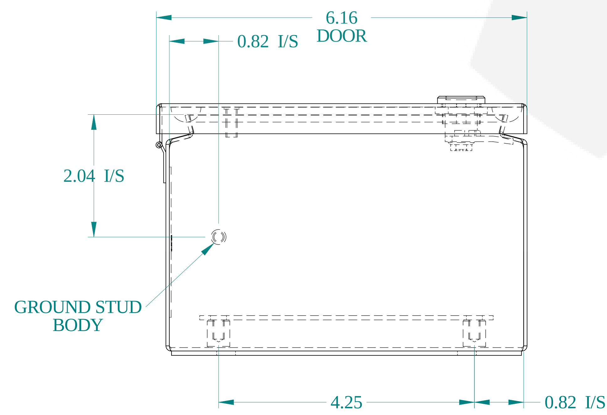
BOTTOM VIEW
