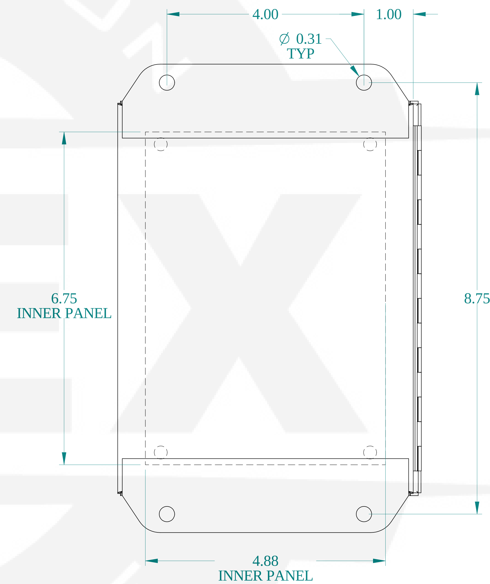
BACK VIEW
