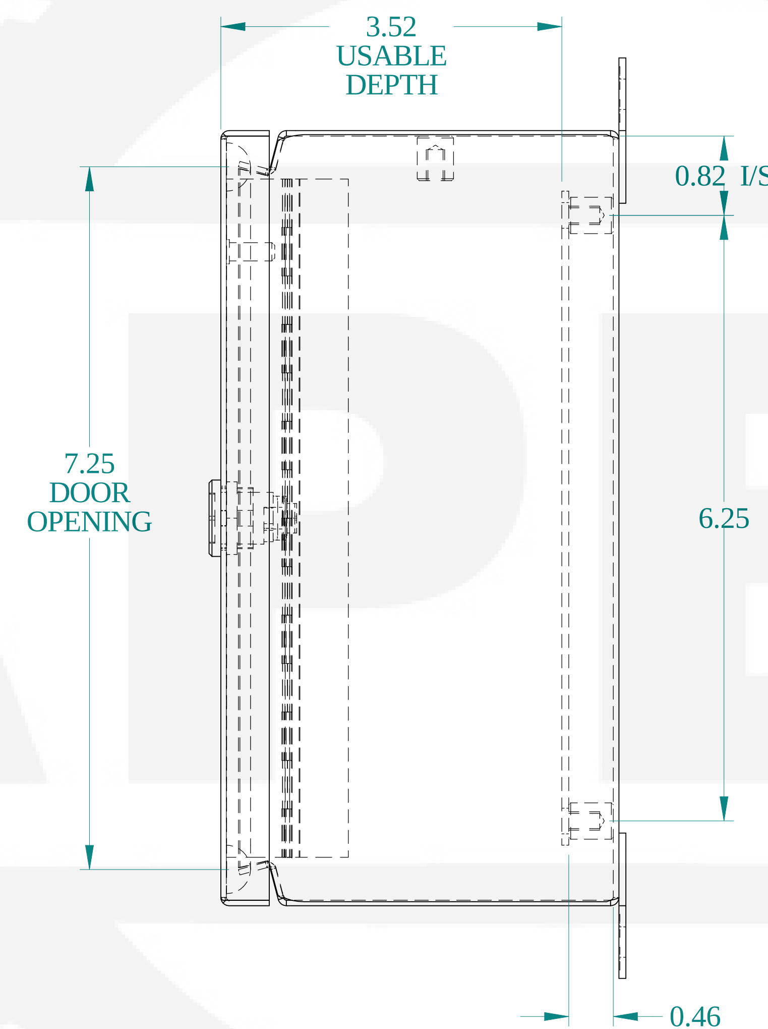
SIDE VIEW
