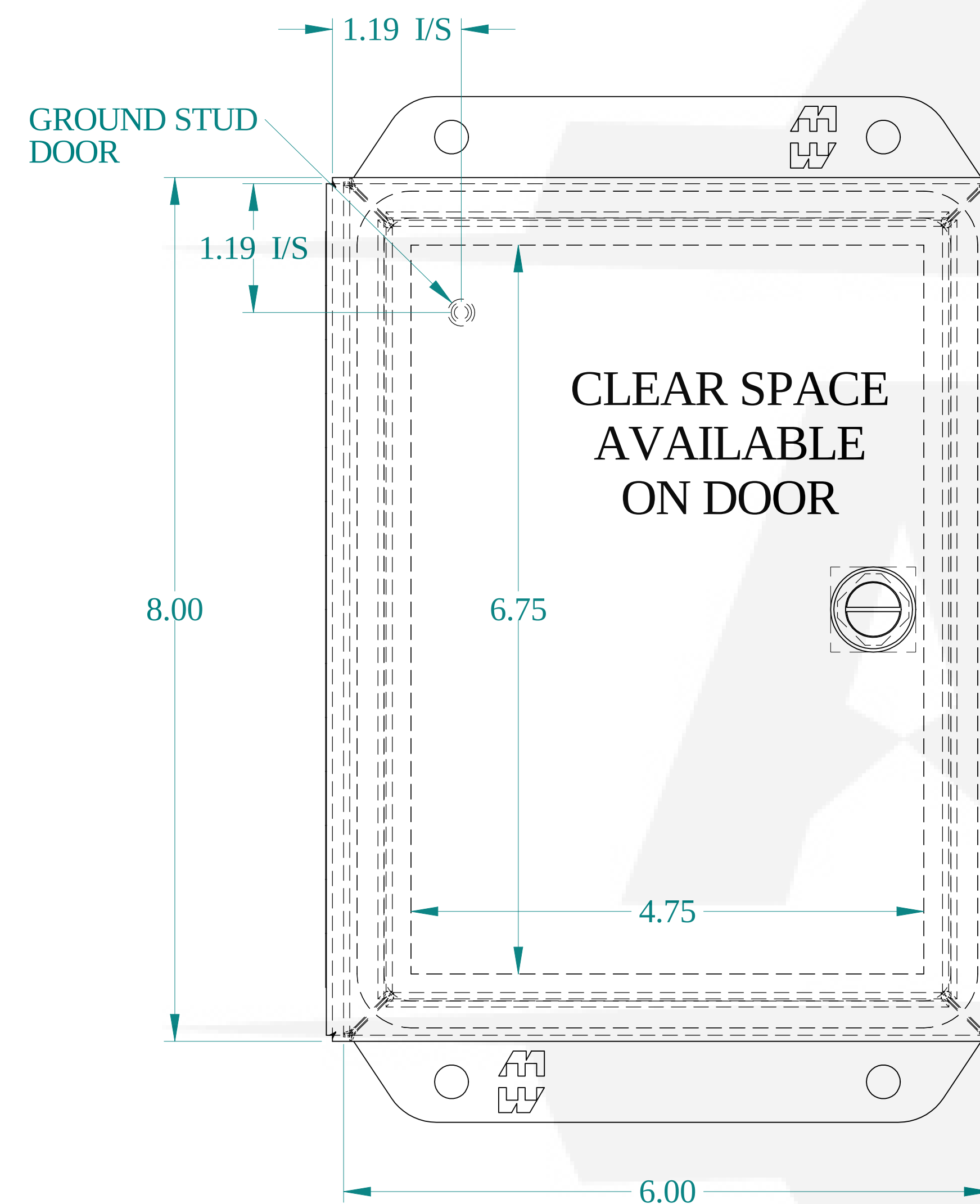
FRONT VIEW
