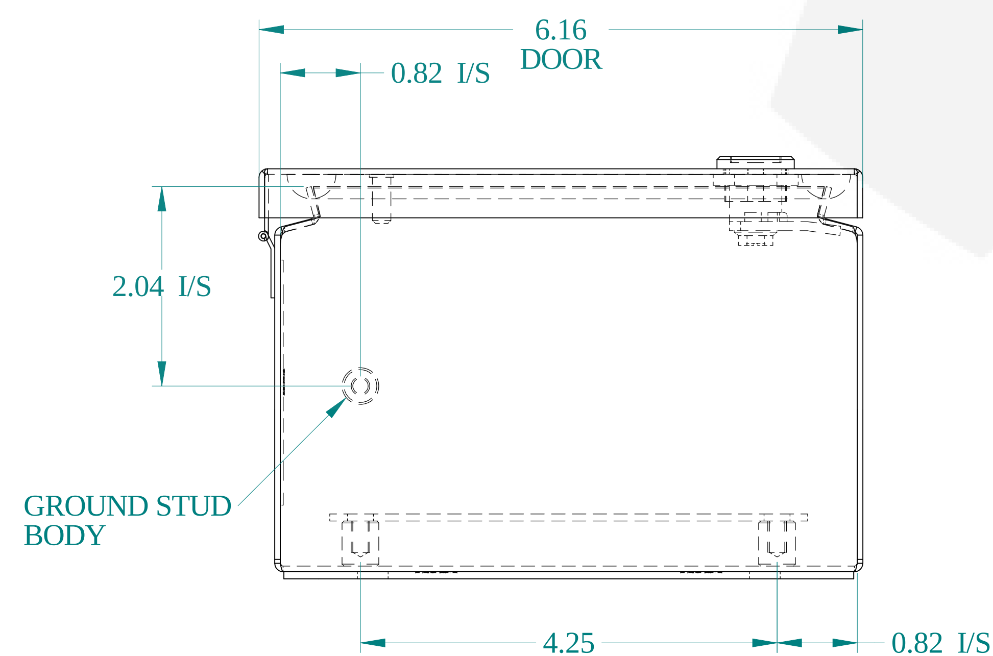
BOTTOM VIEW
