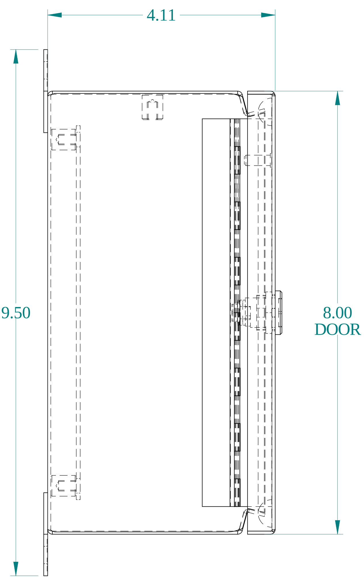
SIDE VIEW
