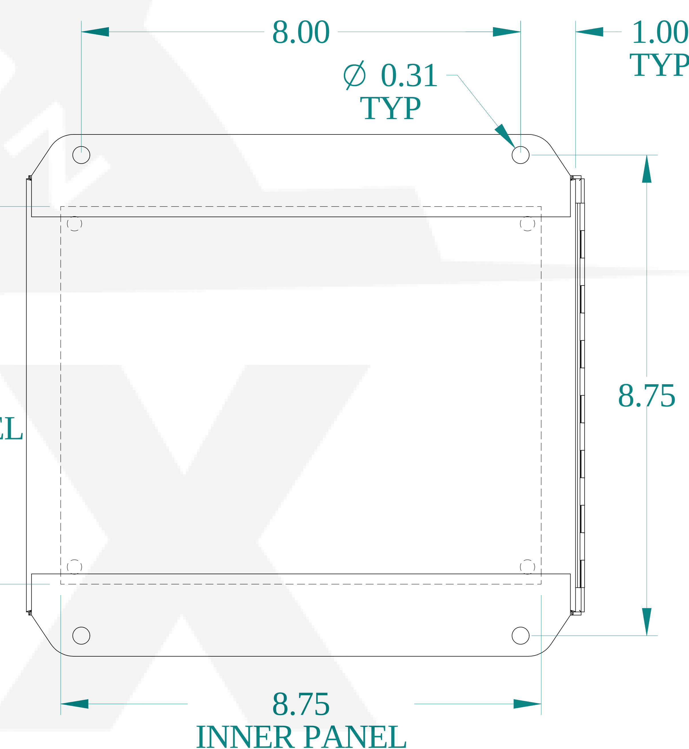
BACK VIEW
