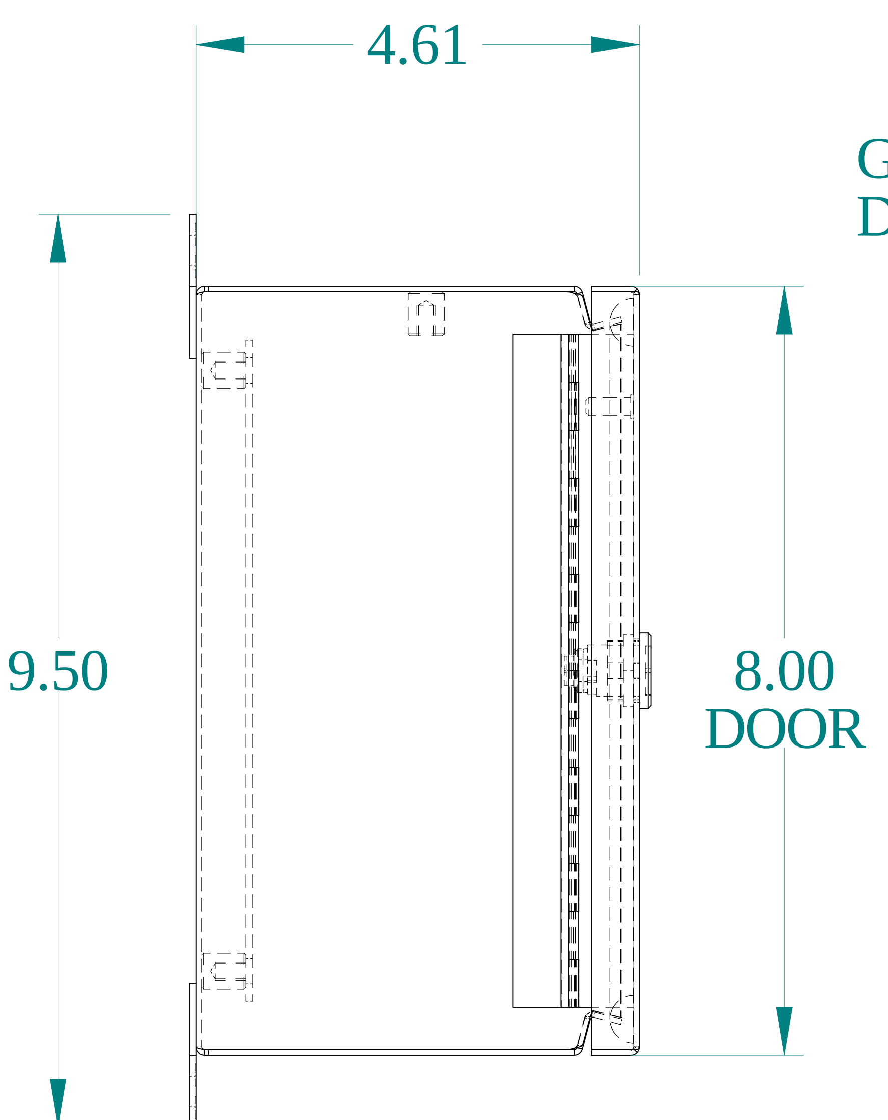
SIDE VIEW
