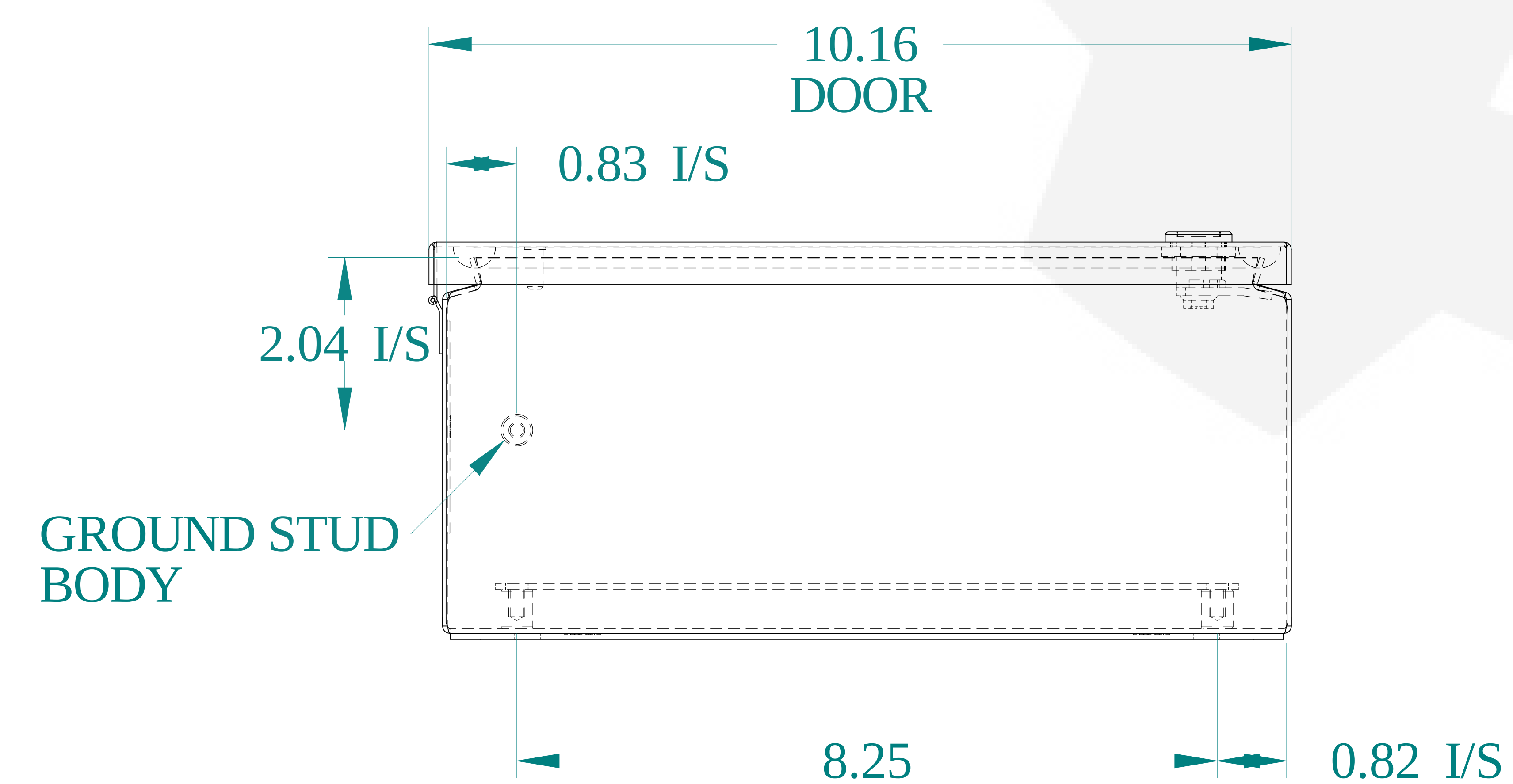
BOTTOM VIEW
