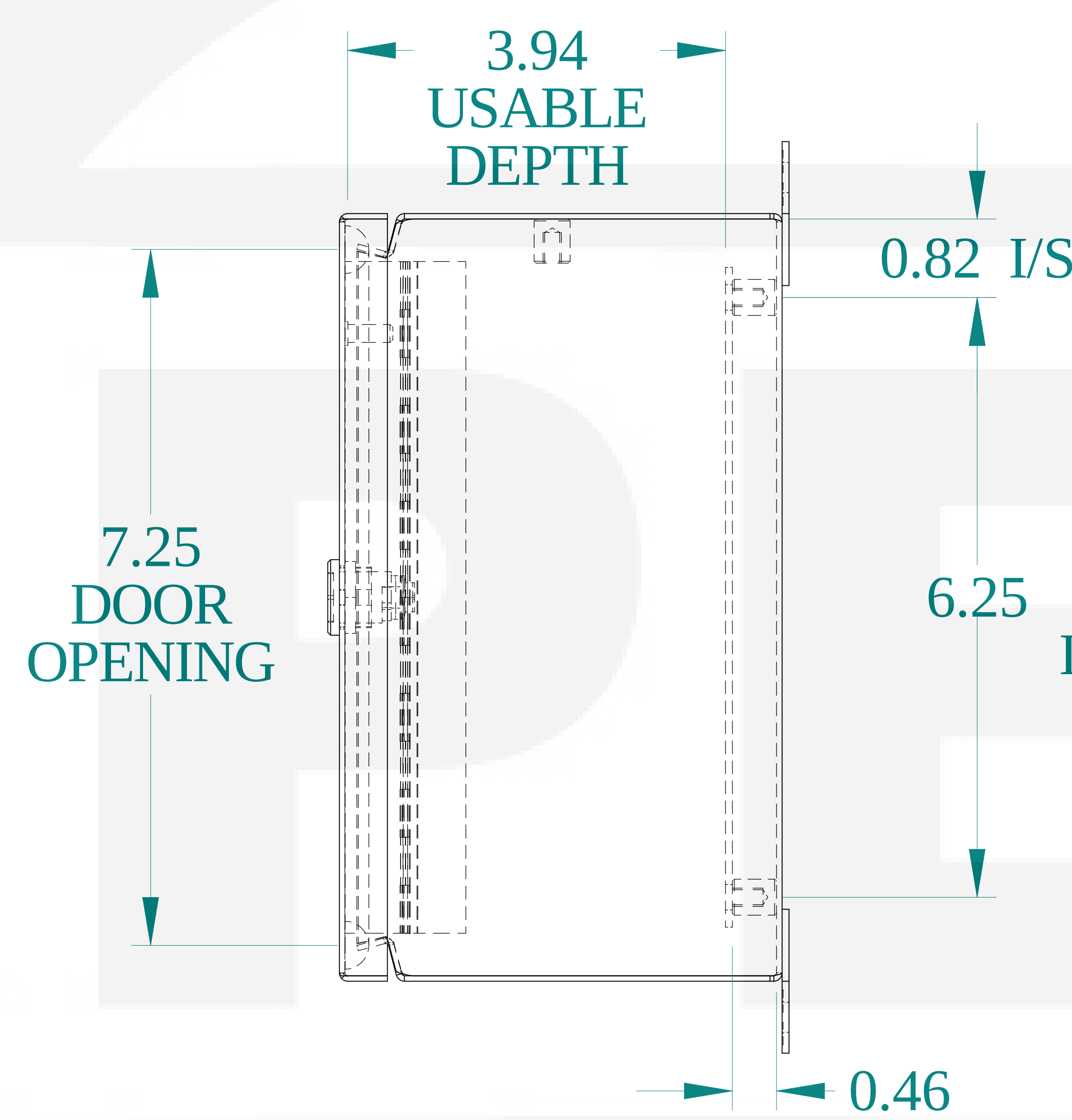
SIDE VIEW
