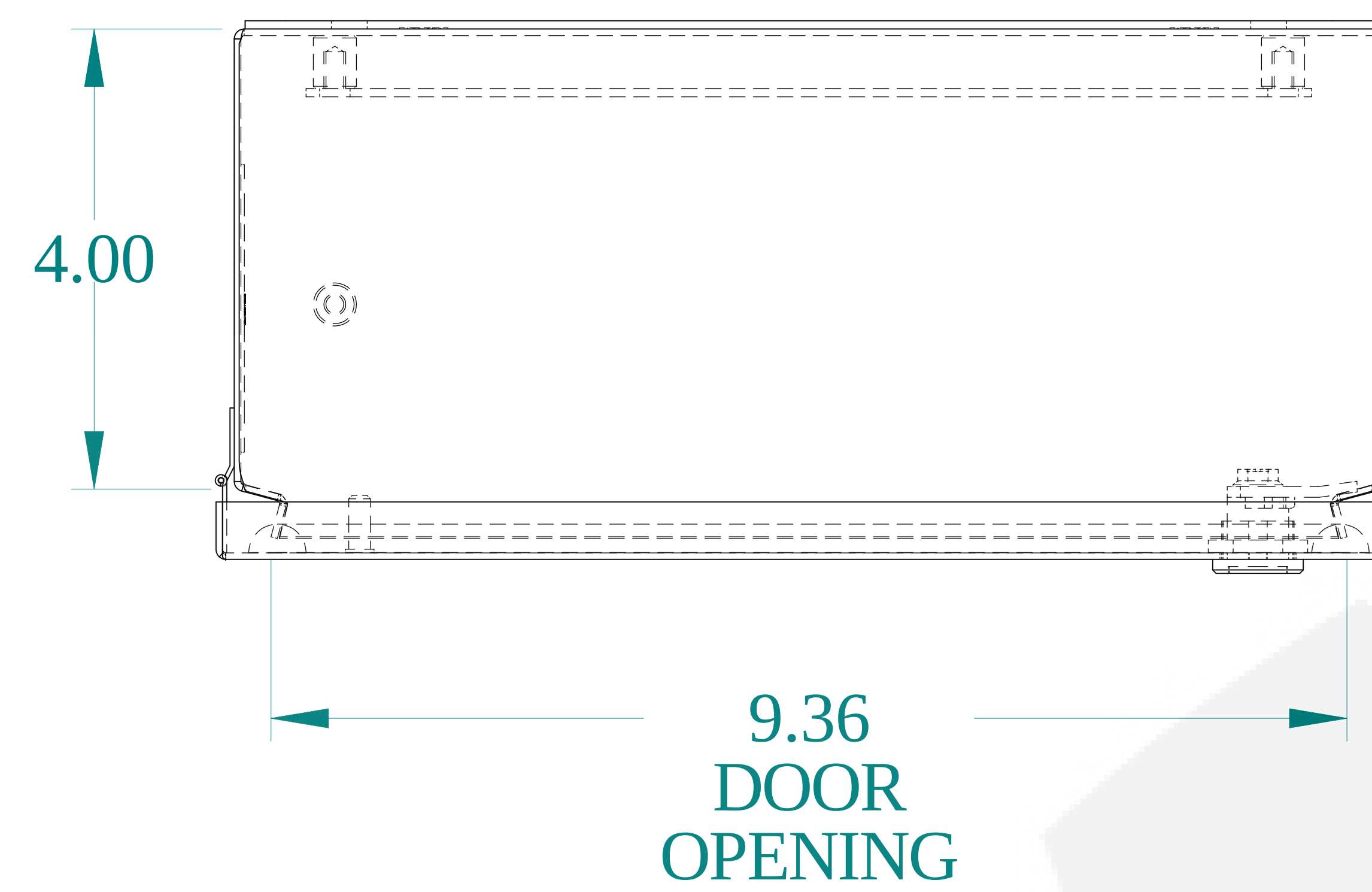
TOP VIEW
