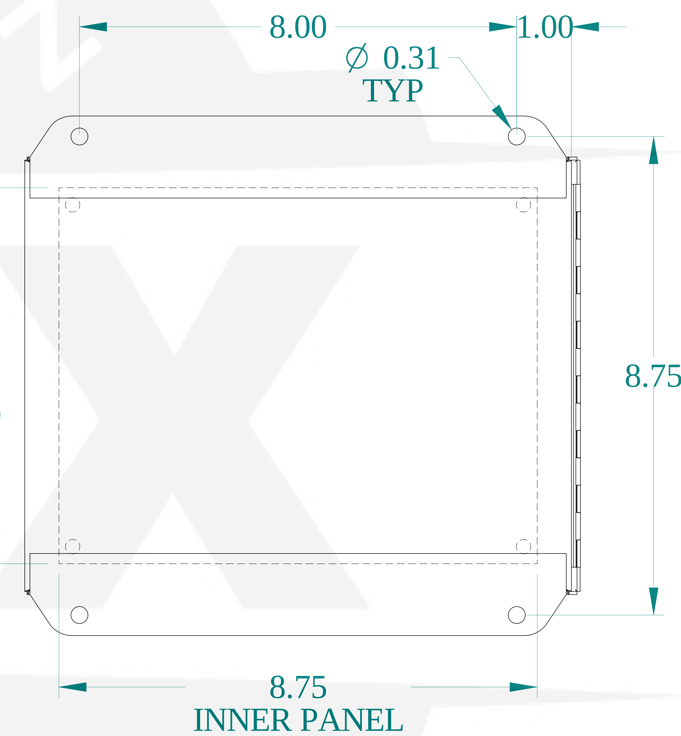
BACK VIEW
