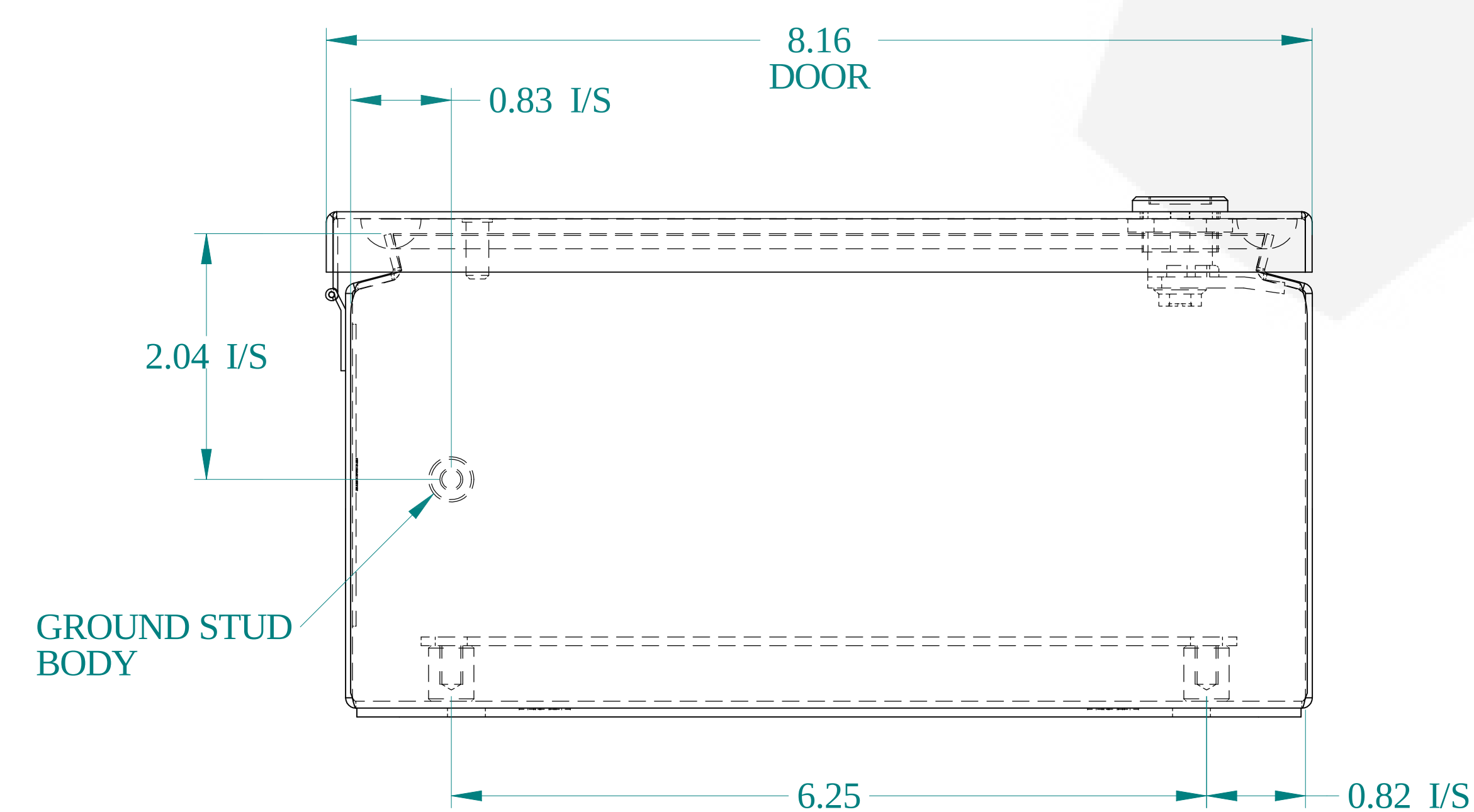
BOTTOM VIEW
