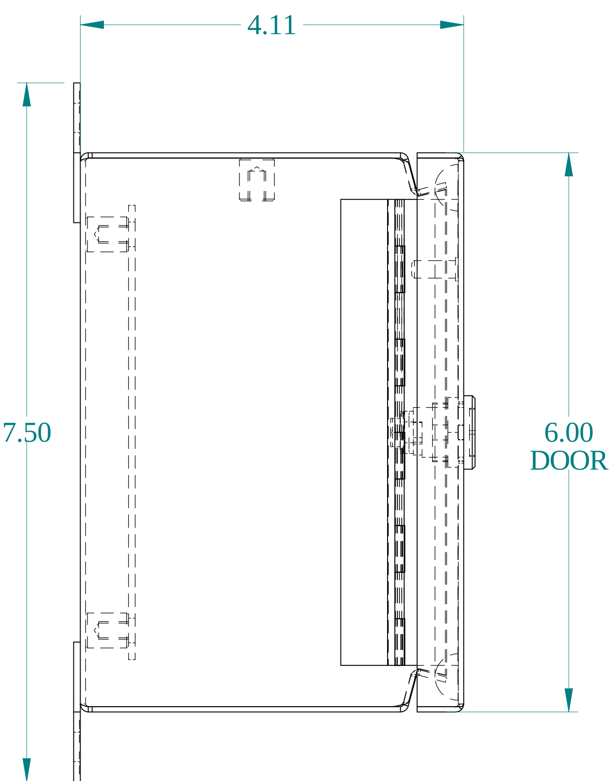
SIDE VIEW
