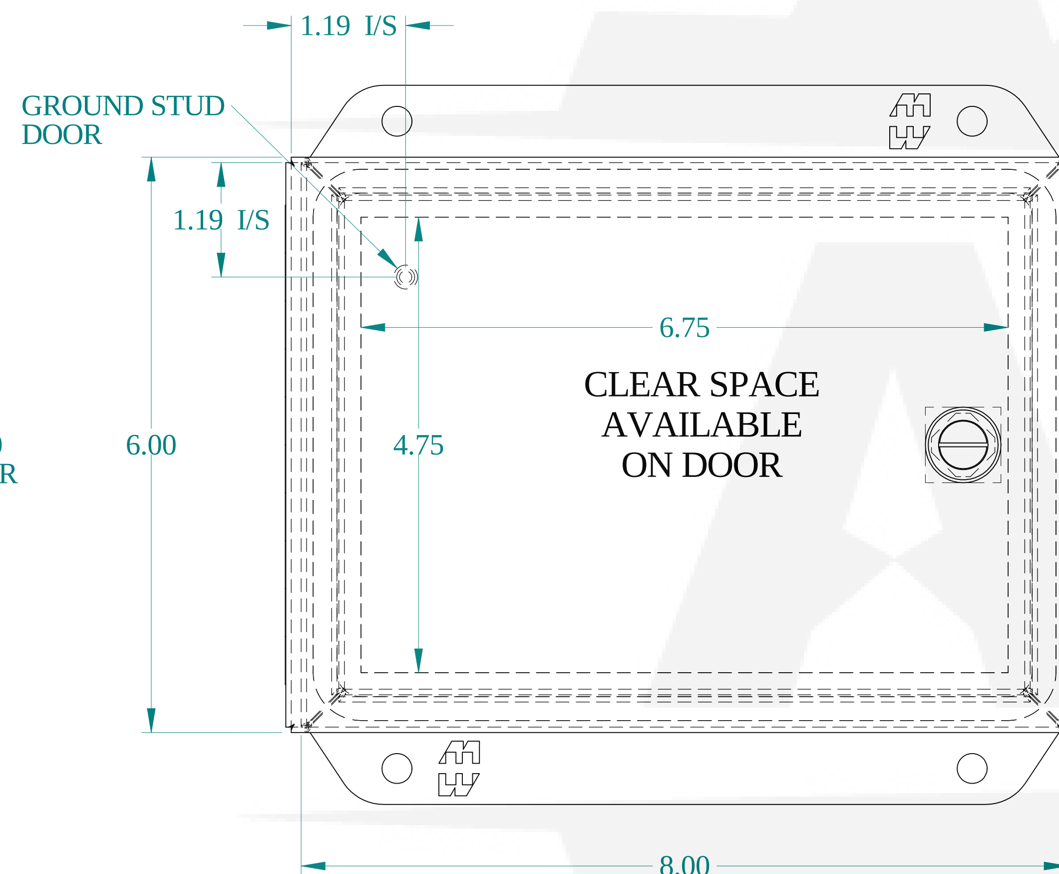
FRONT VIEW
