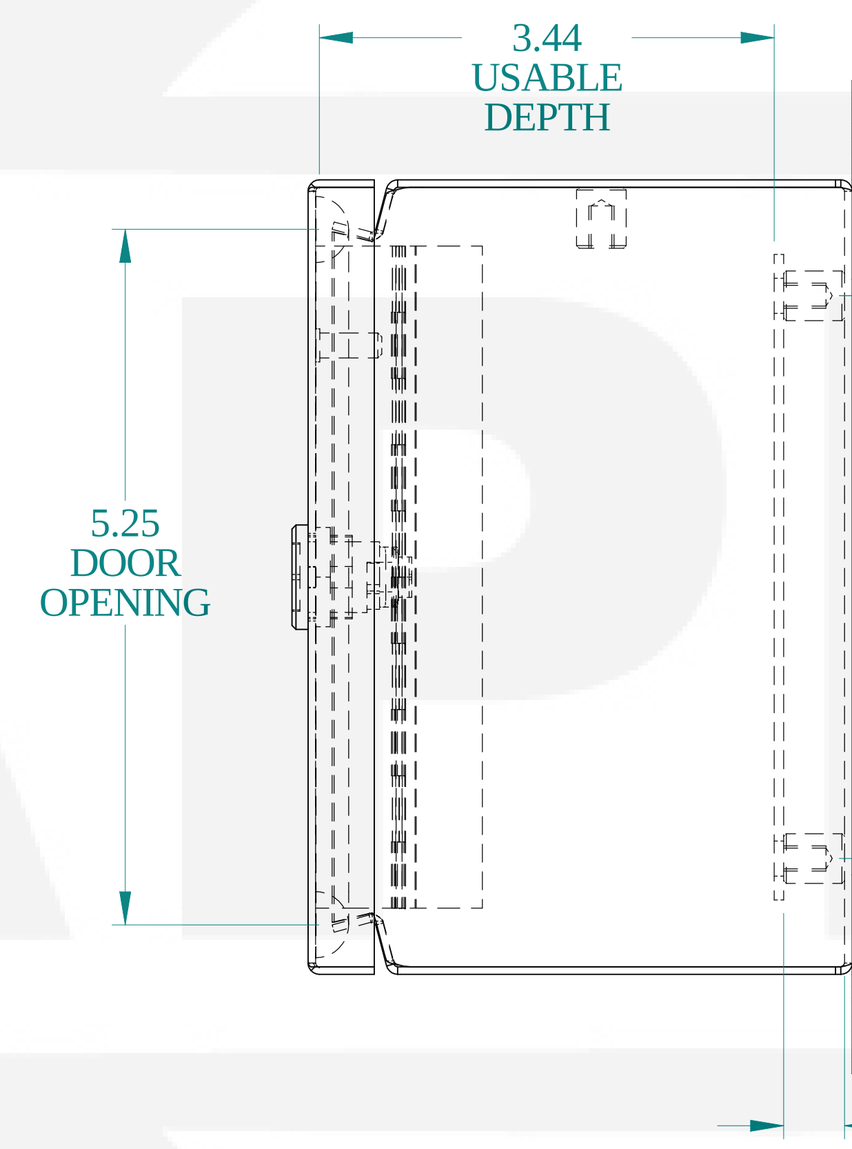
SIDE VIEW
