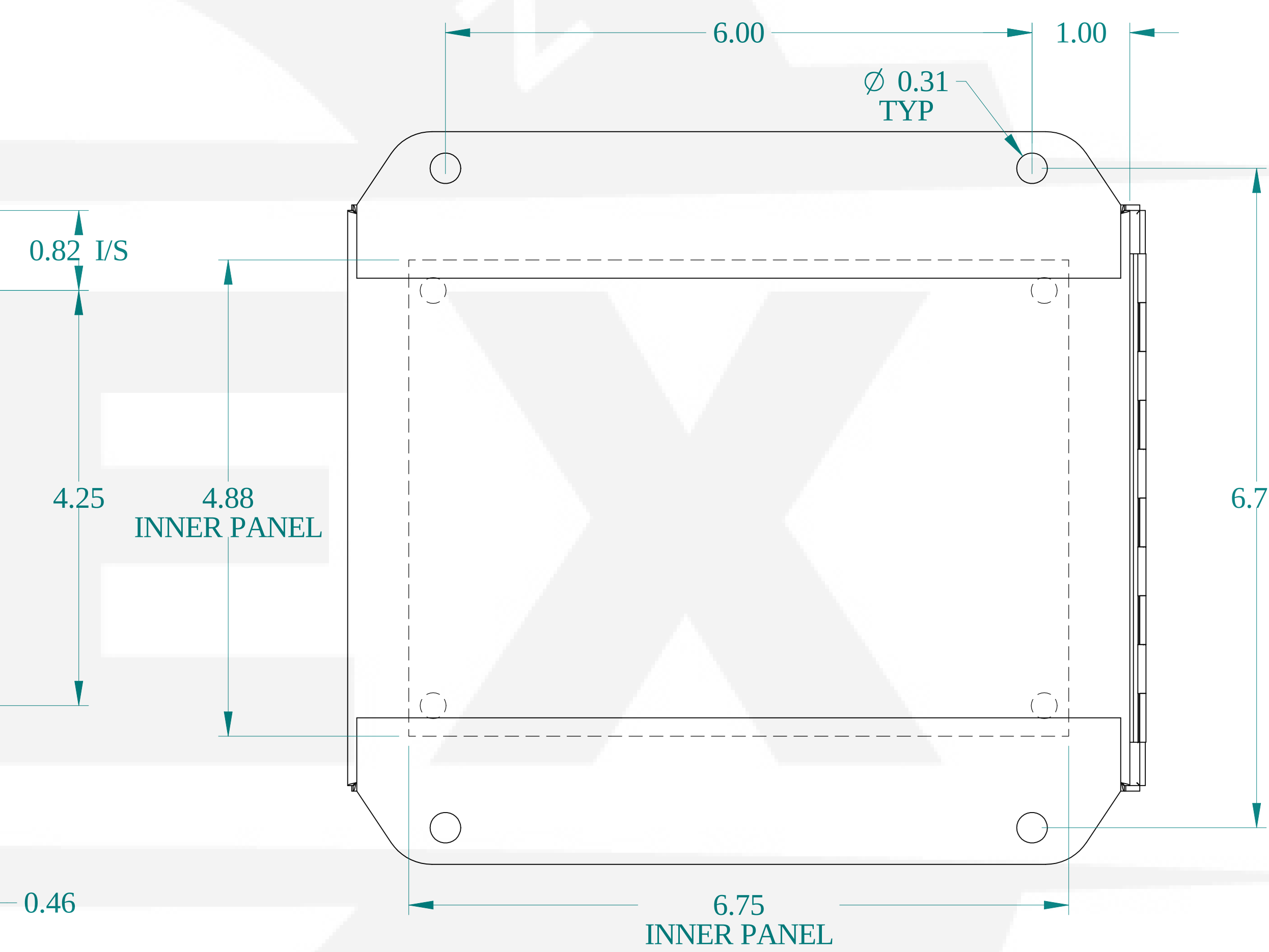
BACK VIEW
