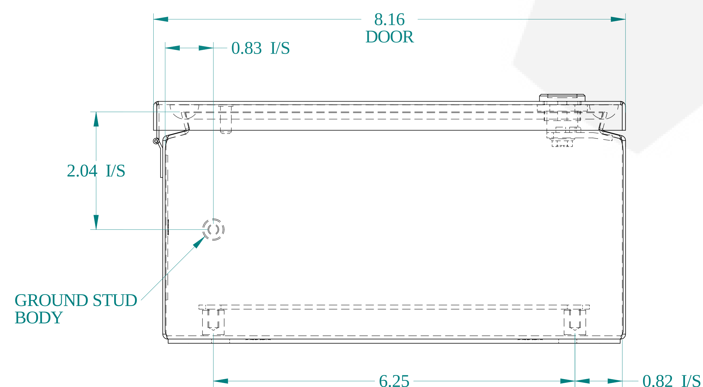
BOTTOM VIEW
