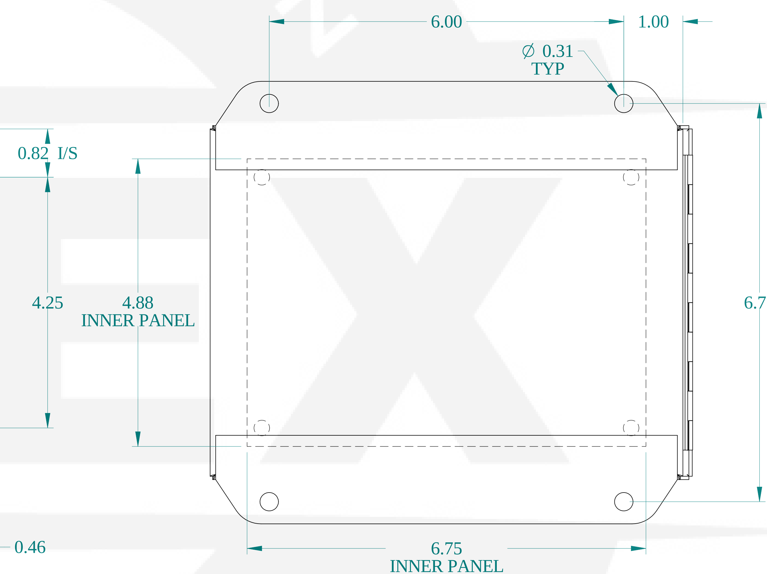
BACK VIEW
