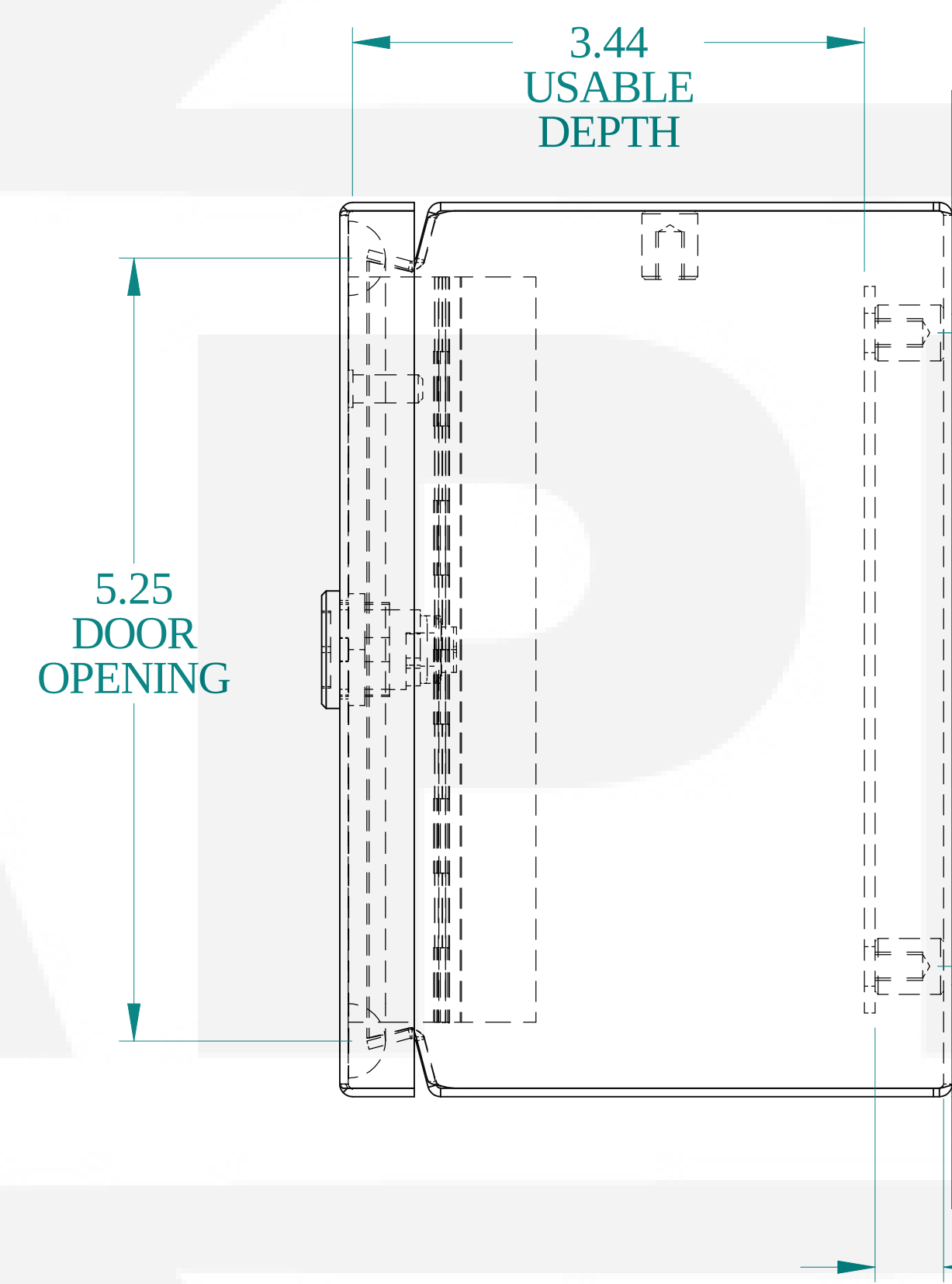
SIDE VIEW
