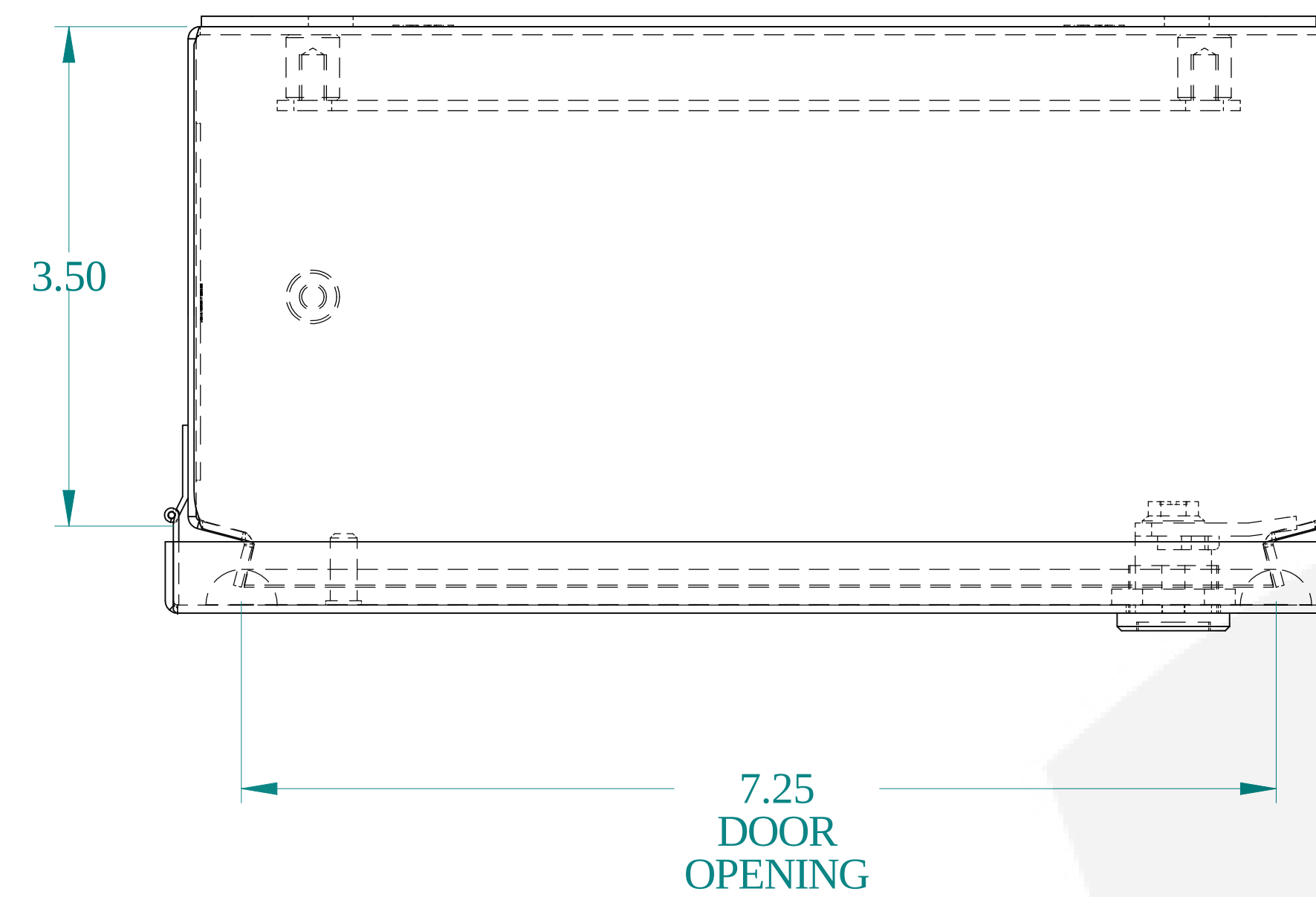
TOP VIEW
