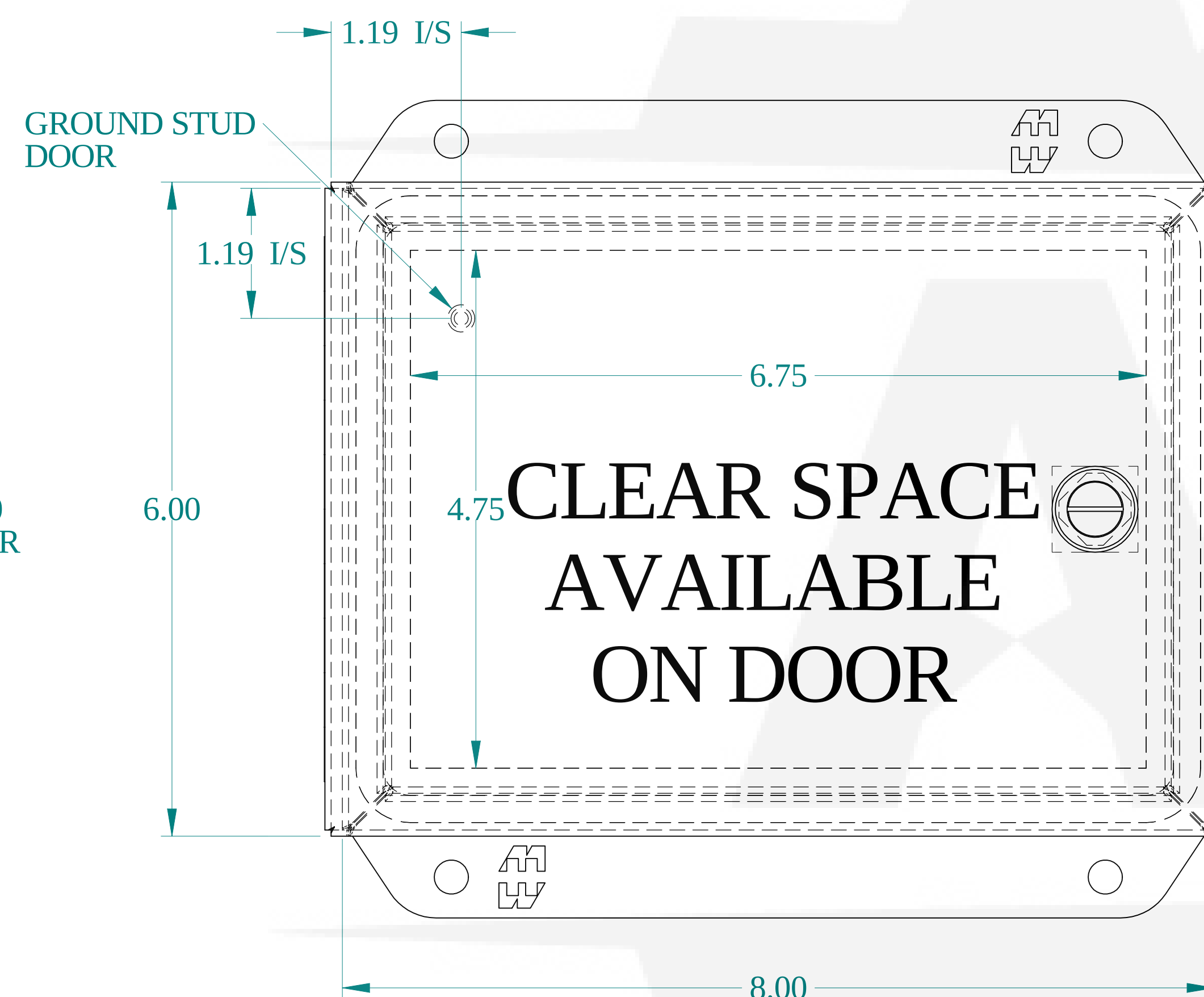
FRONT VIEW
