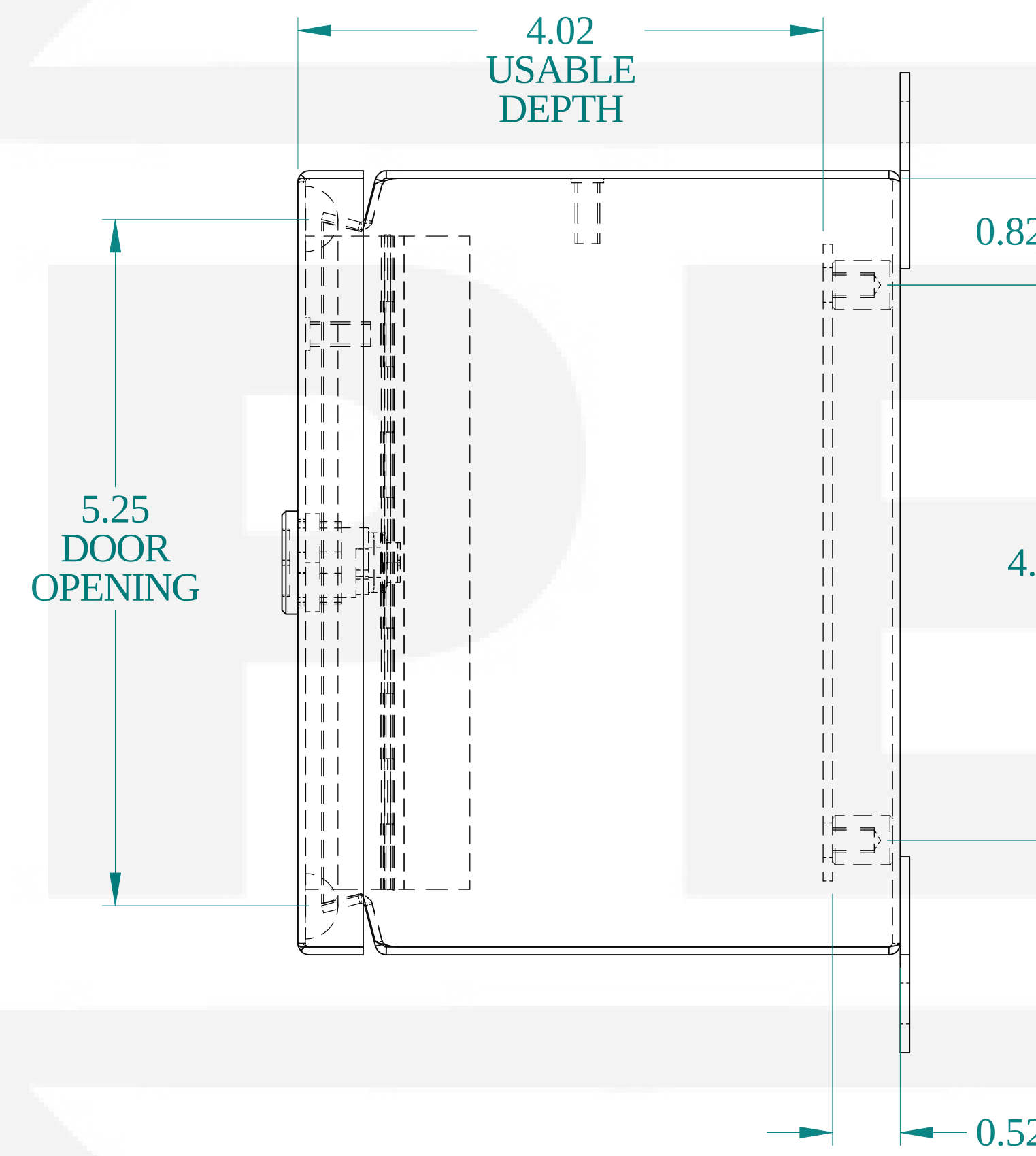
SIDE VIEW
