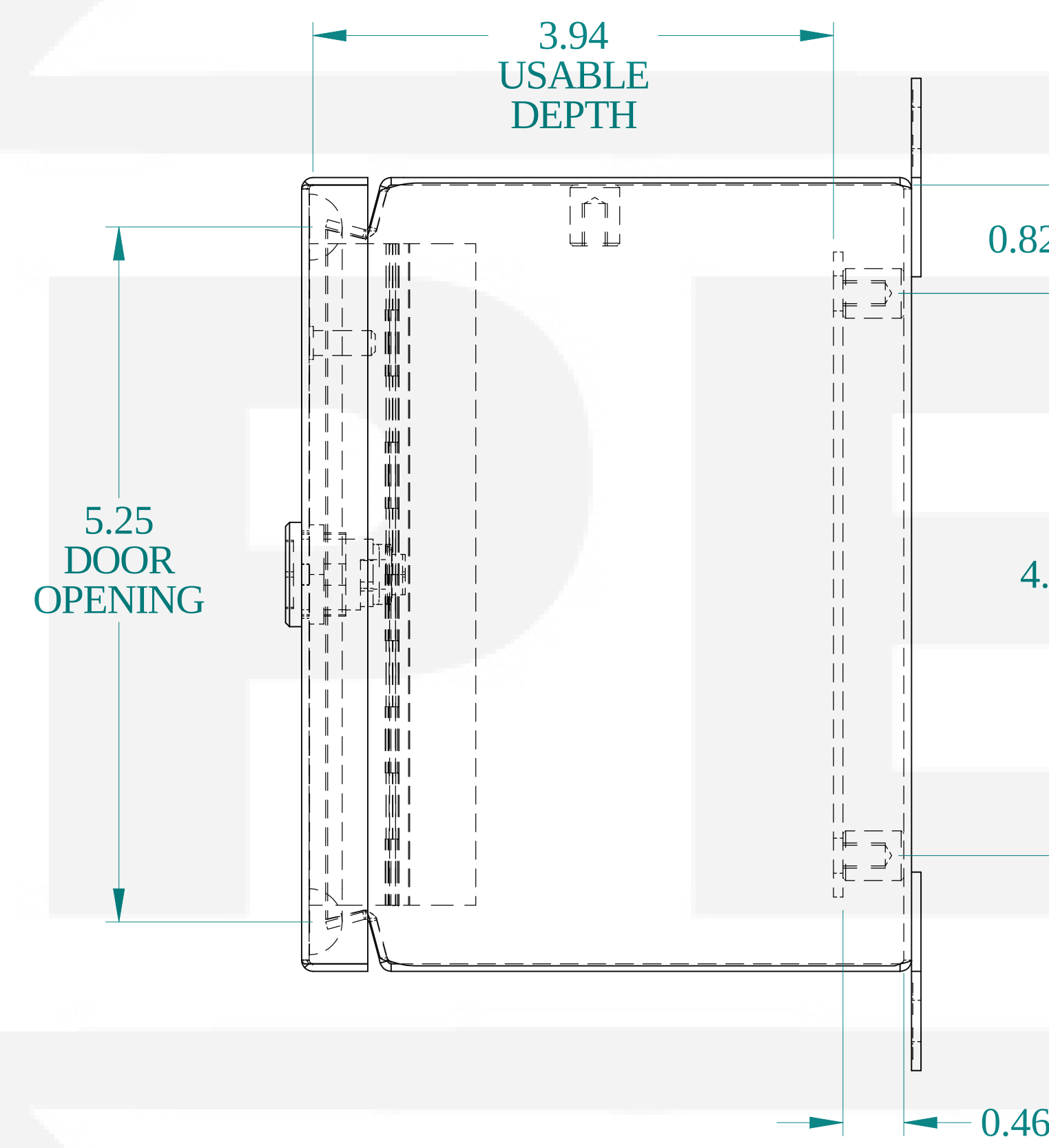
SIDE VIEW
