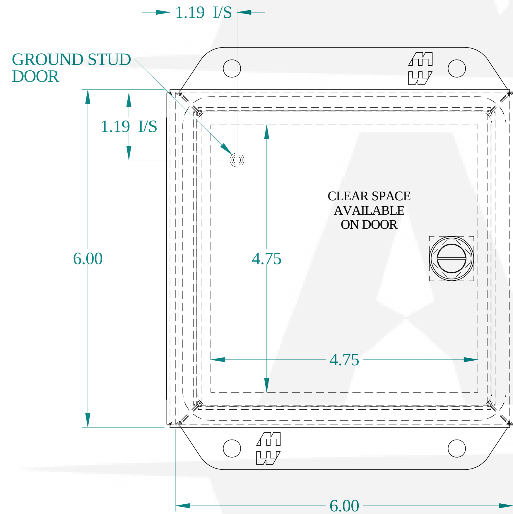
FRONT VIEW
