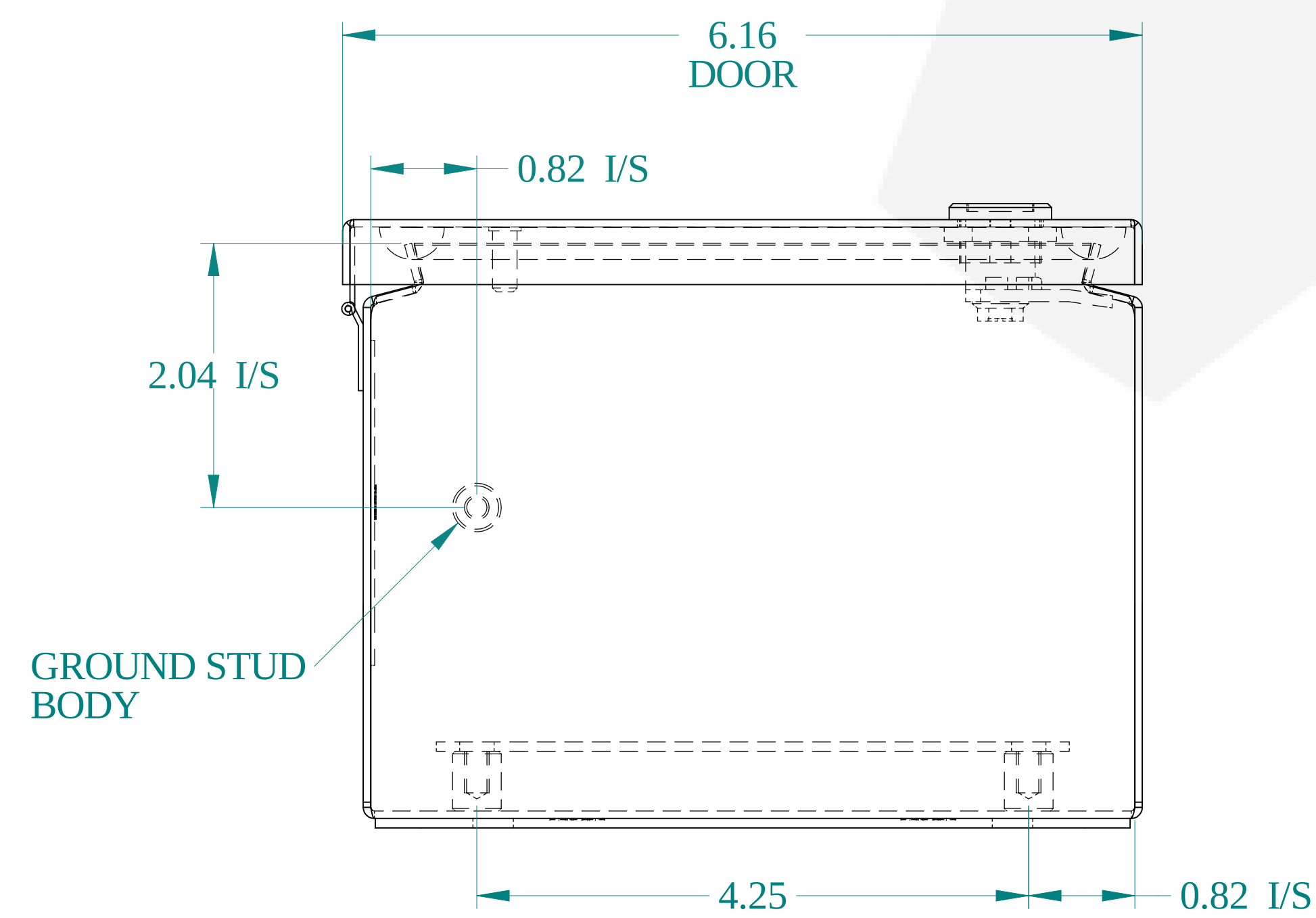
BOTTOM VIEW
