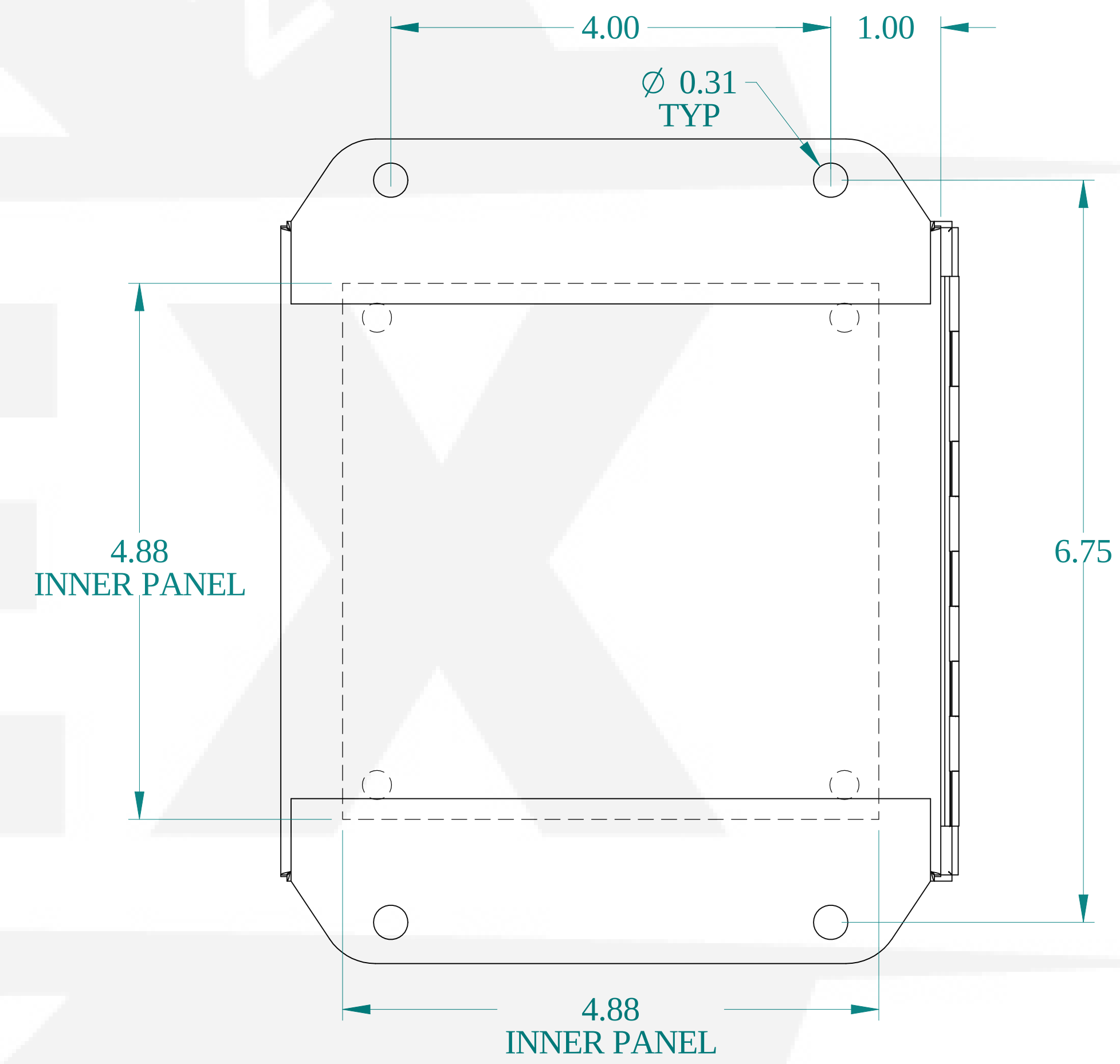
BACK VIEW
