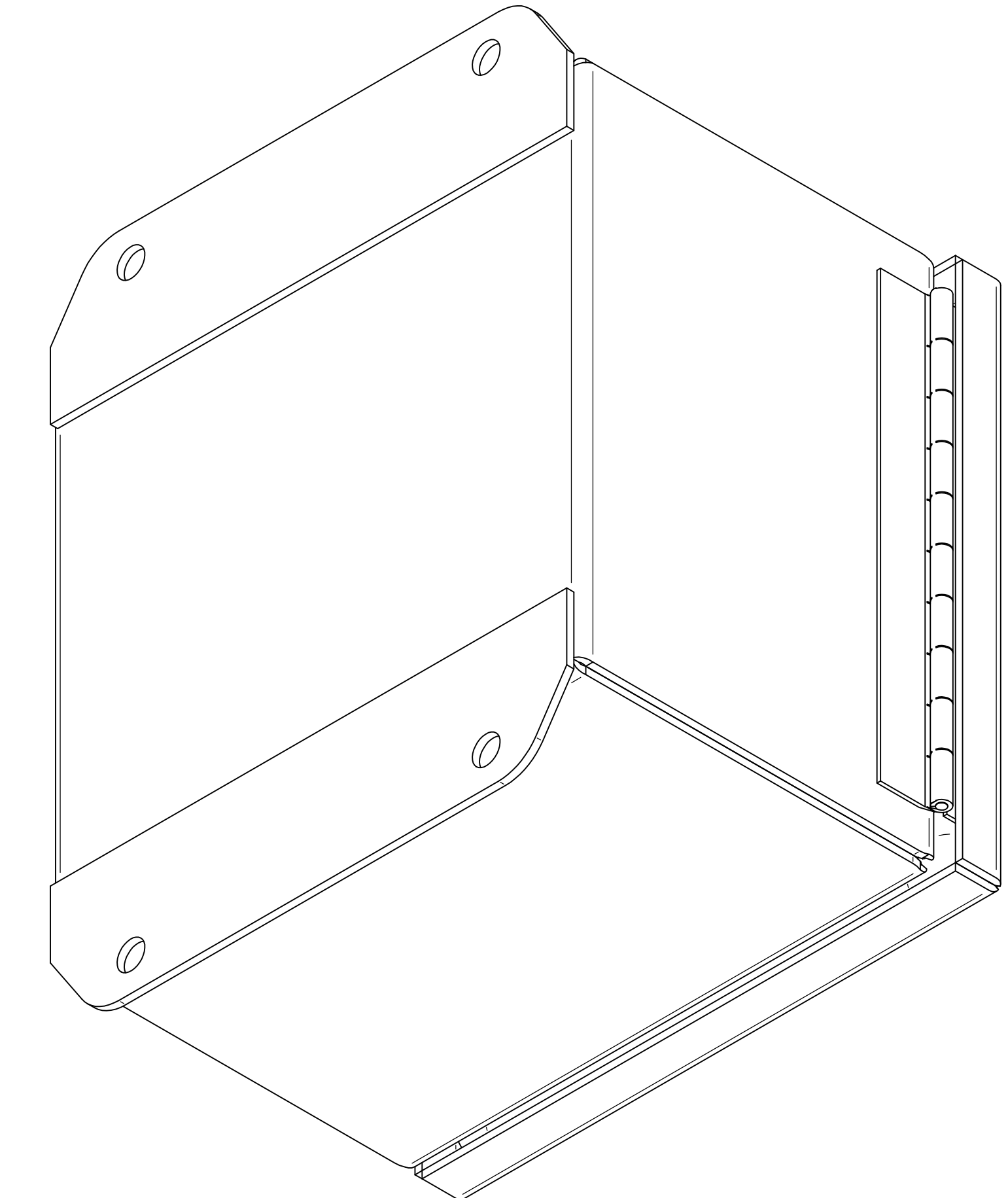
ISOMETRIC VIEWS
