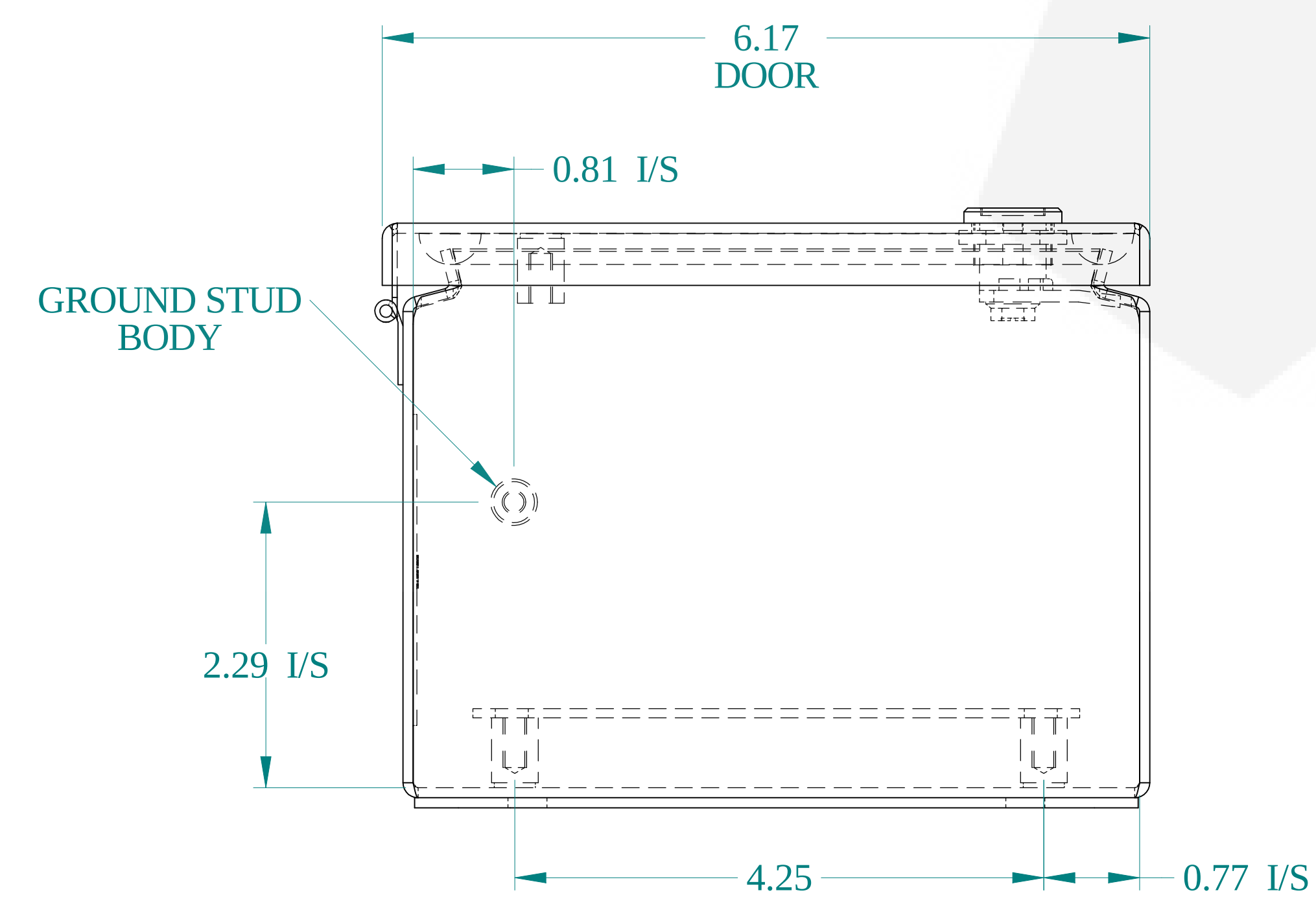
BOTTOM VIEW
