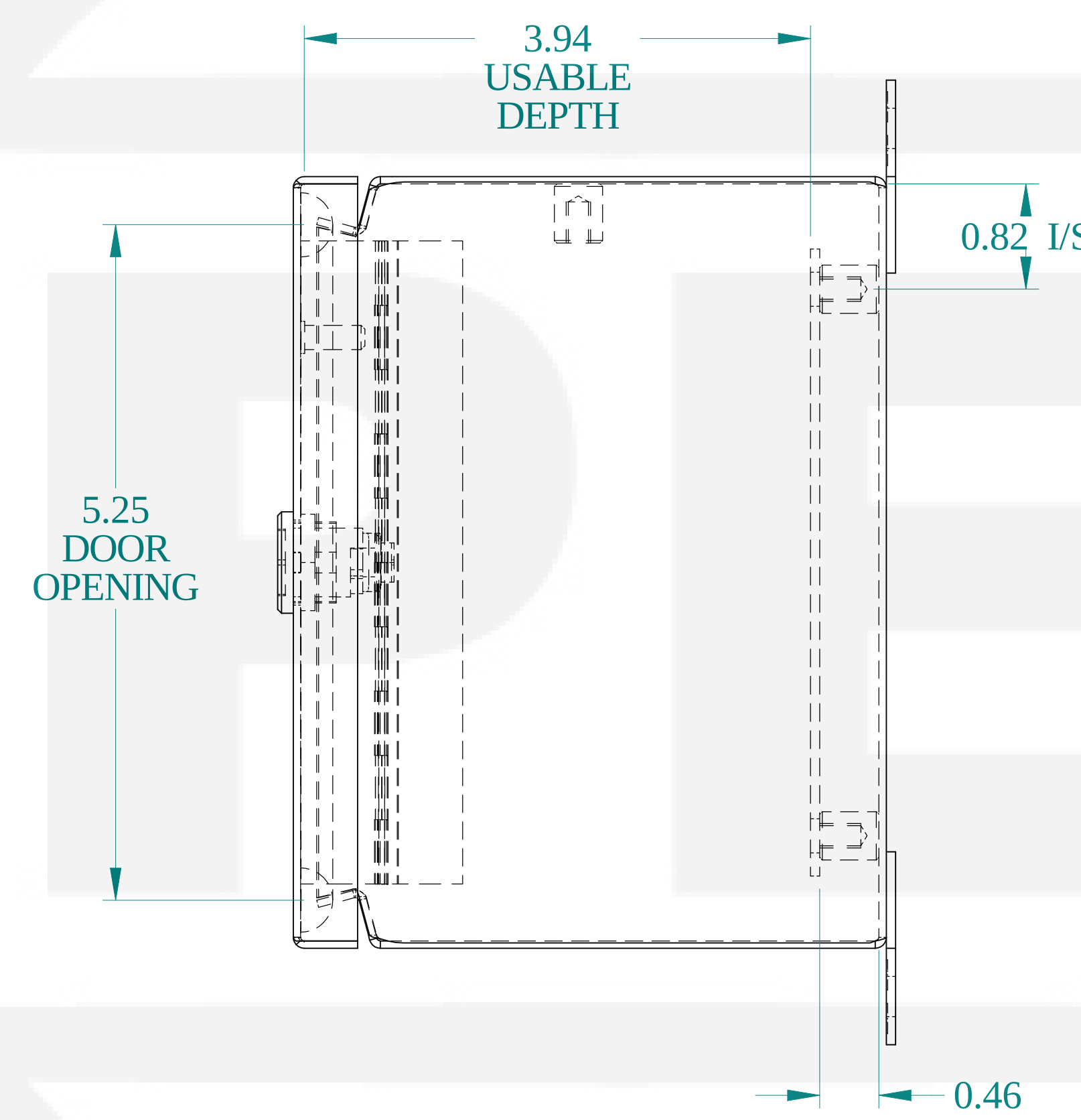
SIDE VIEW
