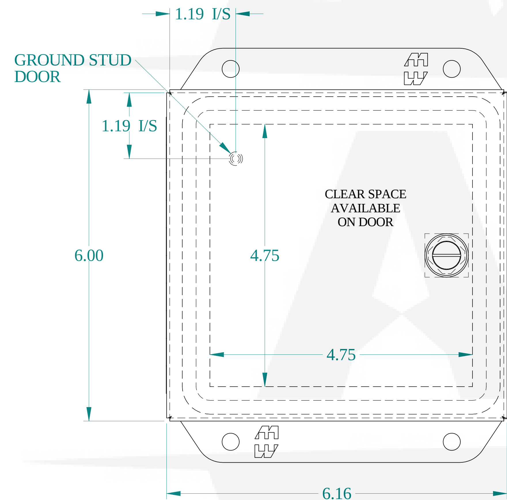
FRONT VIEW
