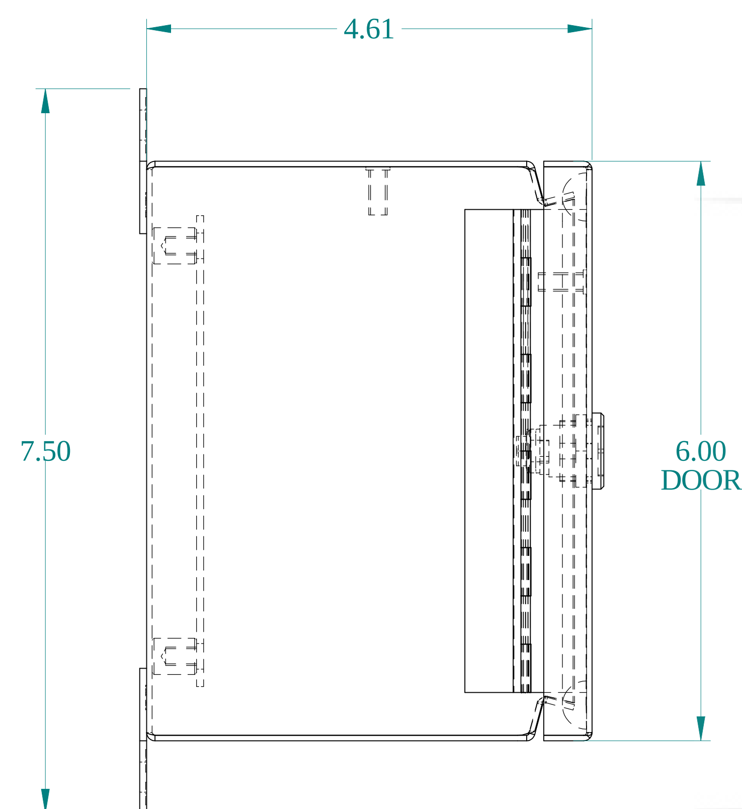
SIDE VIEW
