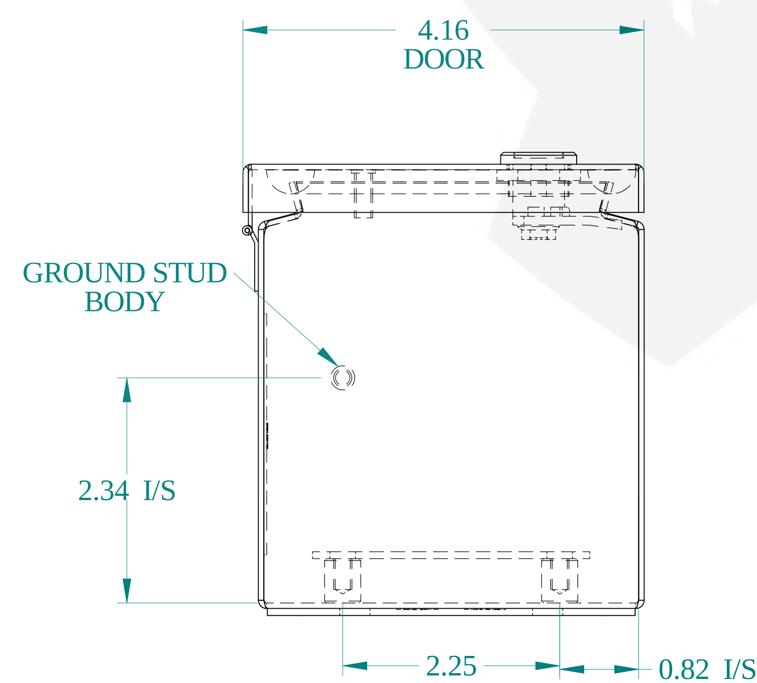
BOTTOM VIEW
