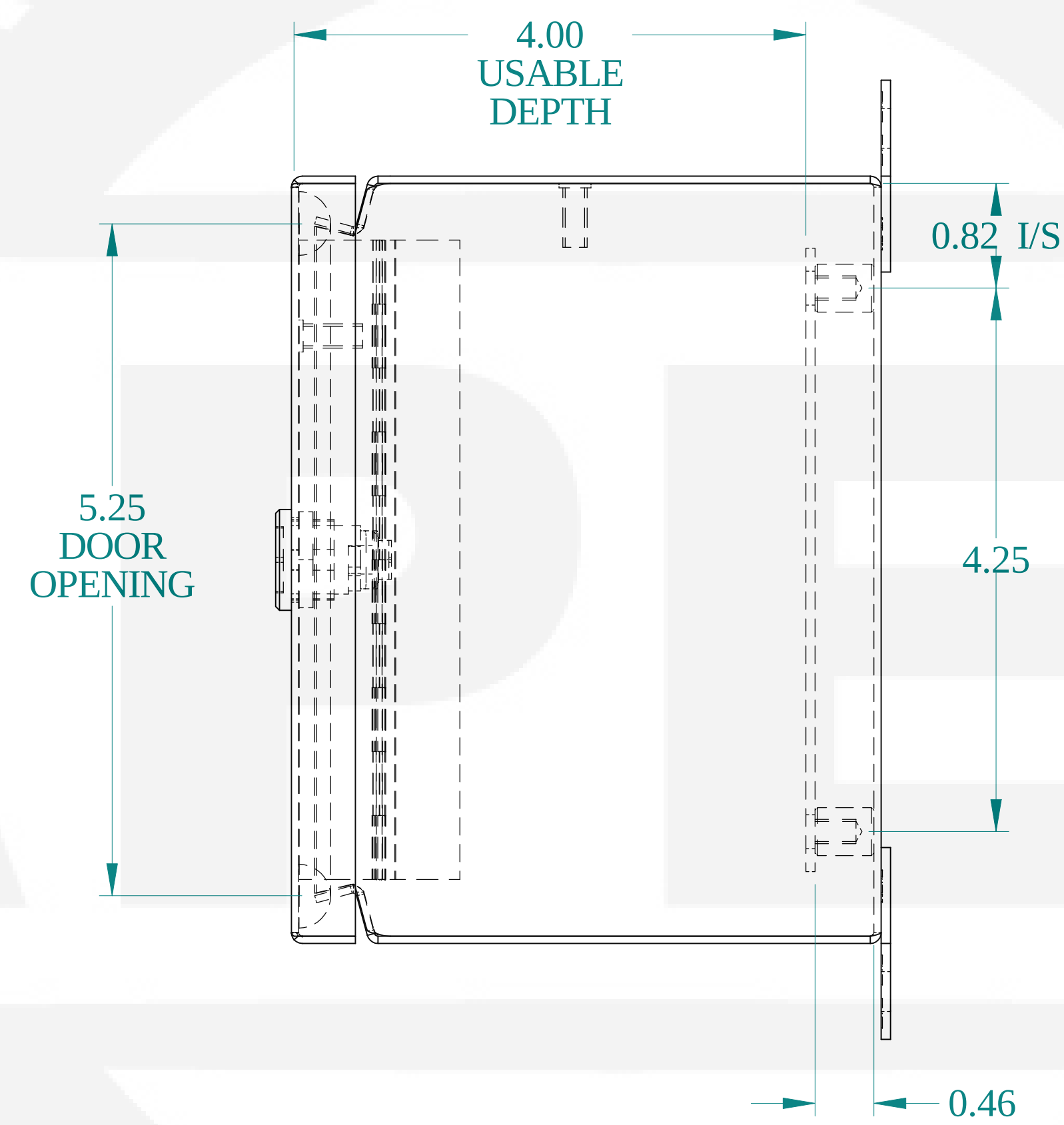
SIDE VIEW
