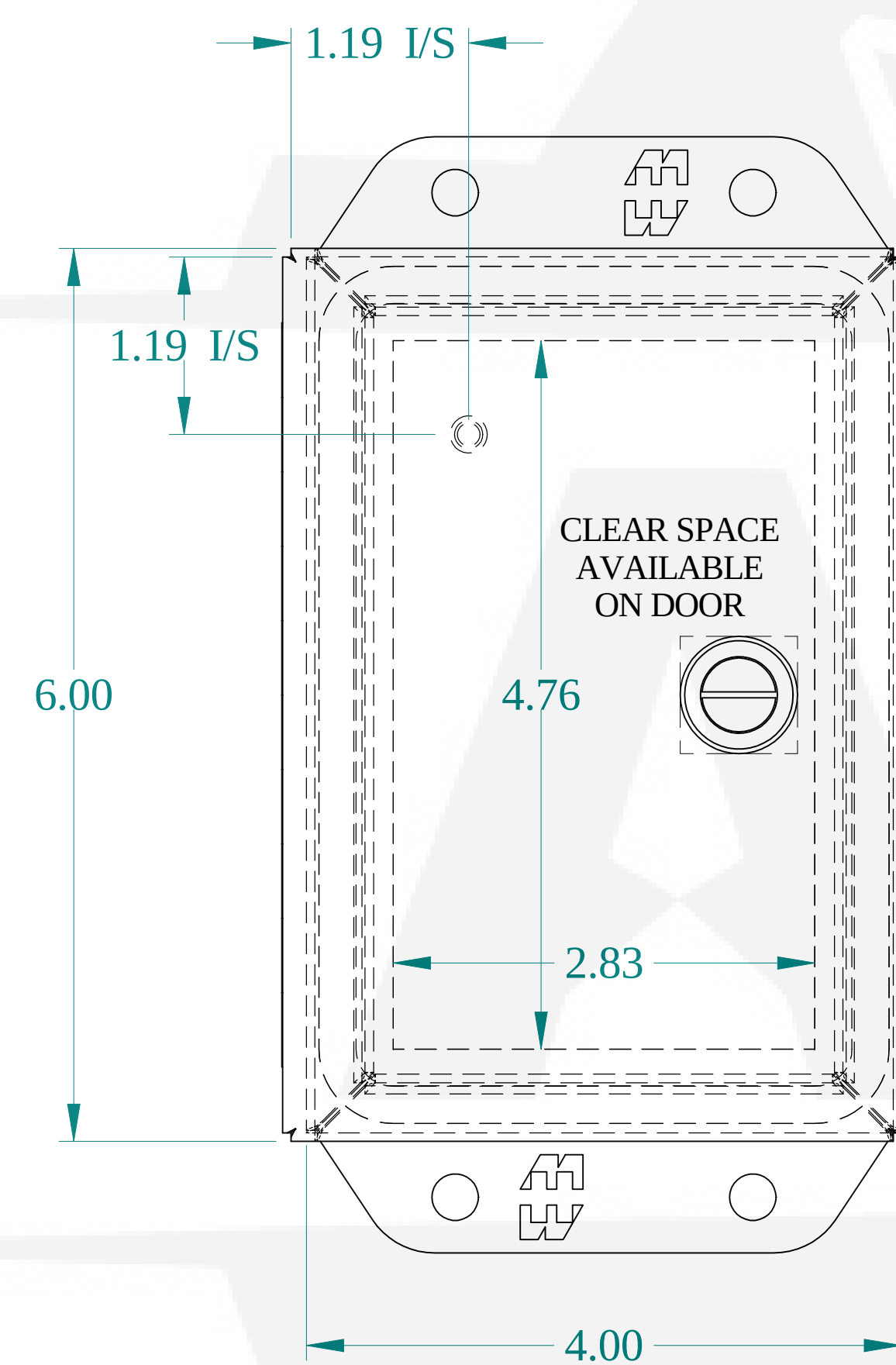
FRONT VIEW
