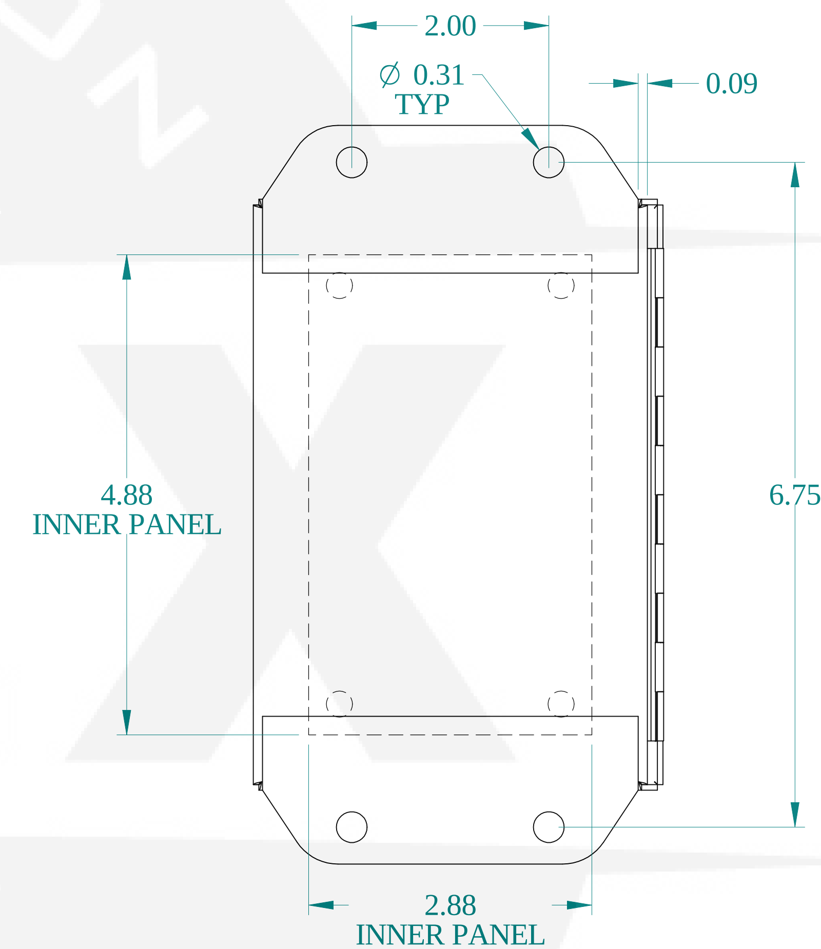
BACK VIEW
