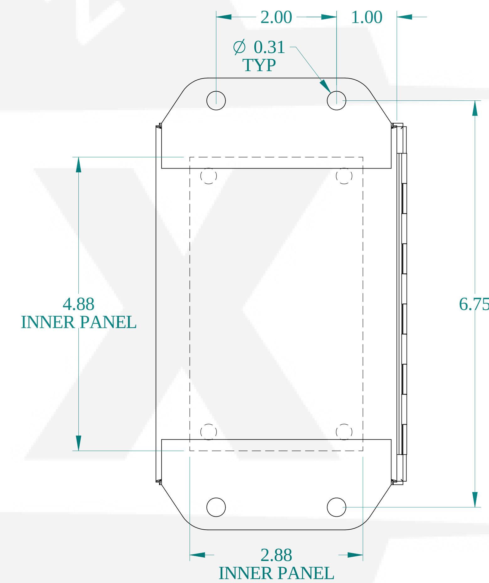
BACK VIEW
