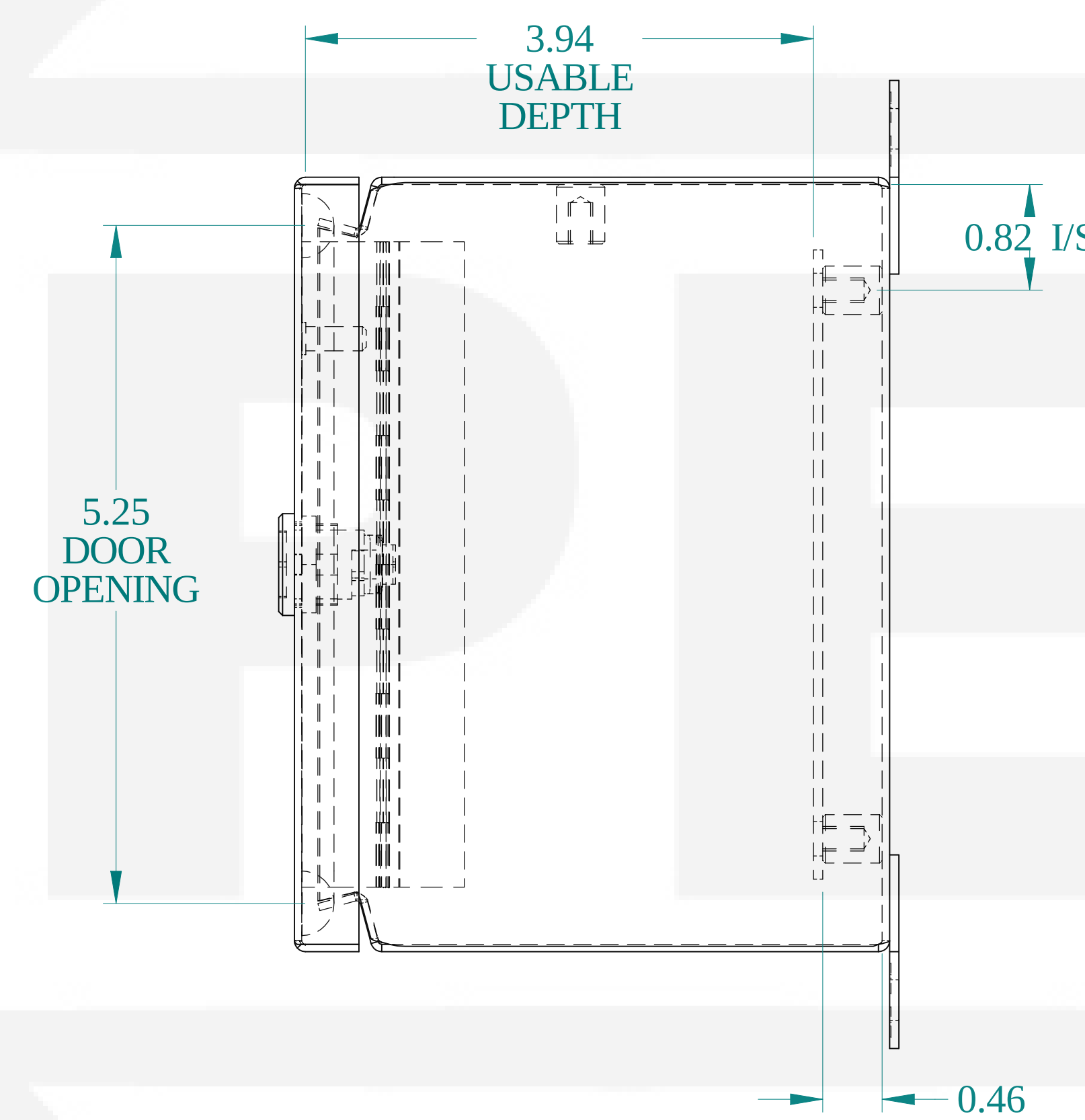
SIDE VIEW
