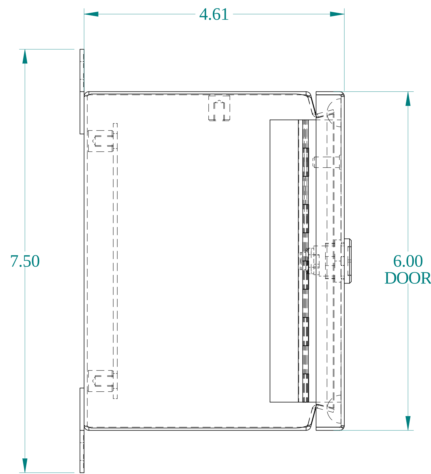
SIDE VIEW
