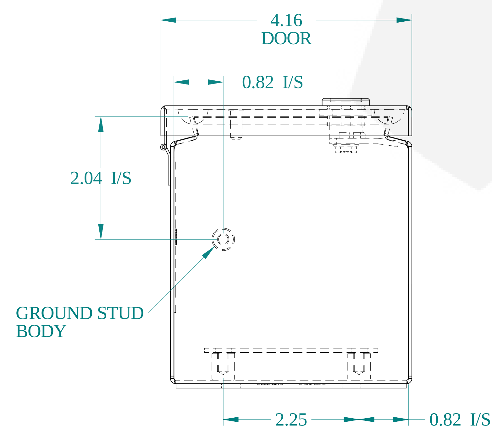
BOTTOM VIEW
