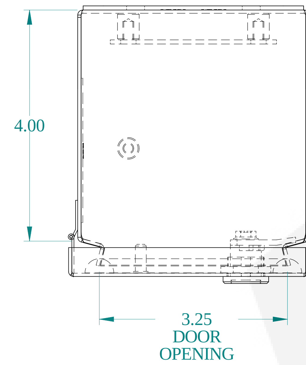
TOP VIEW
