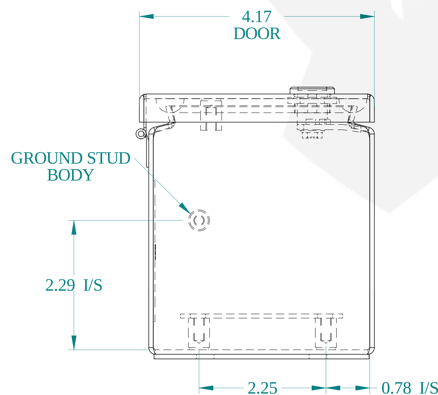
BOTTOM VIEW
