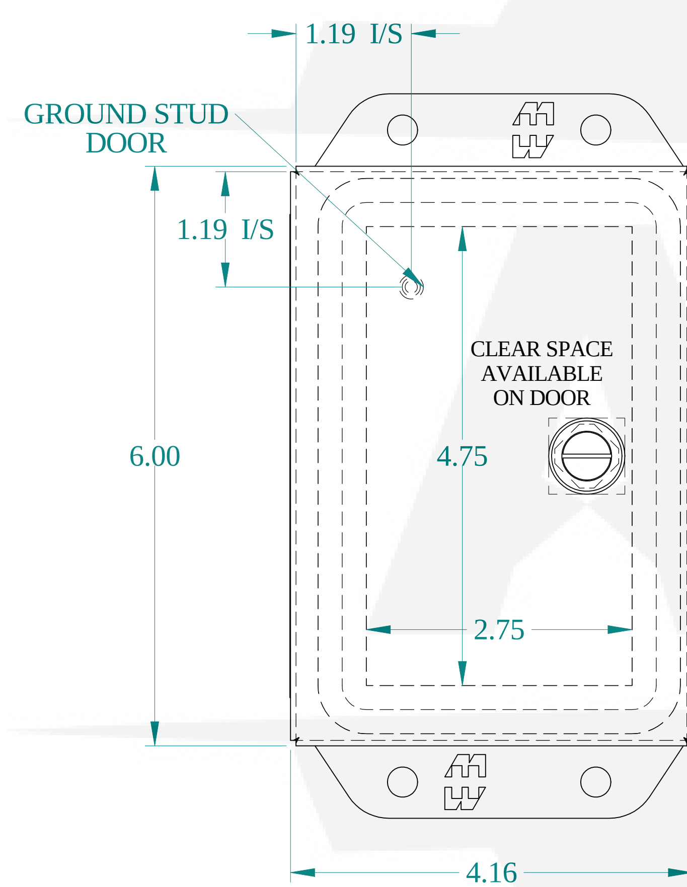
FRONT VIEW
