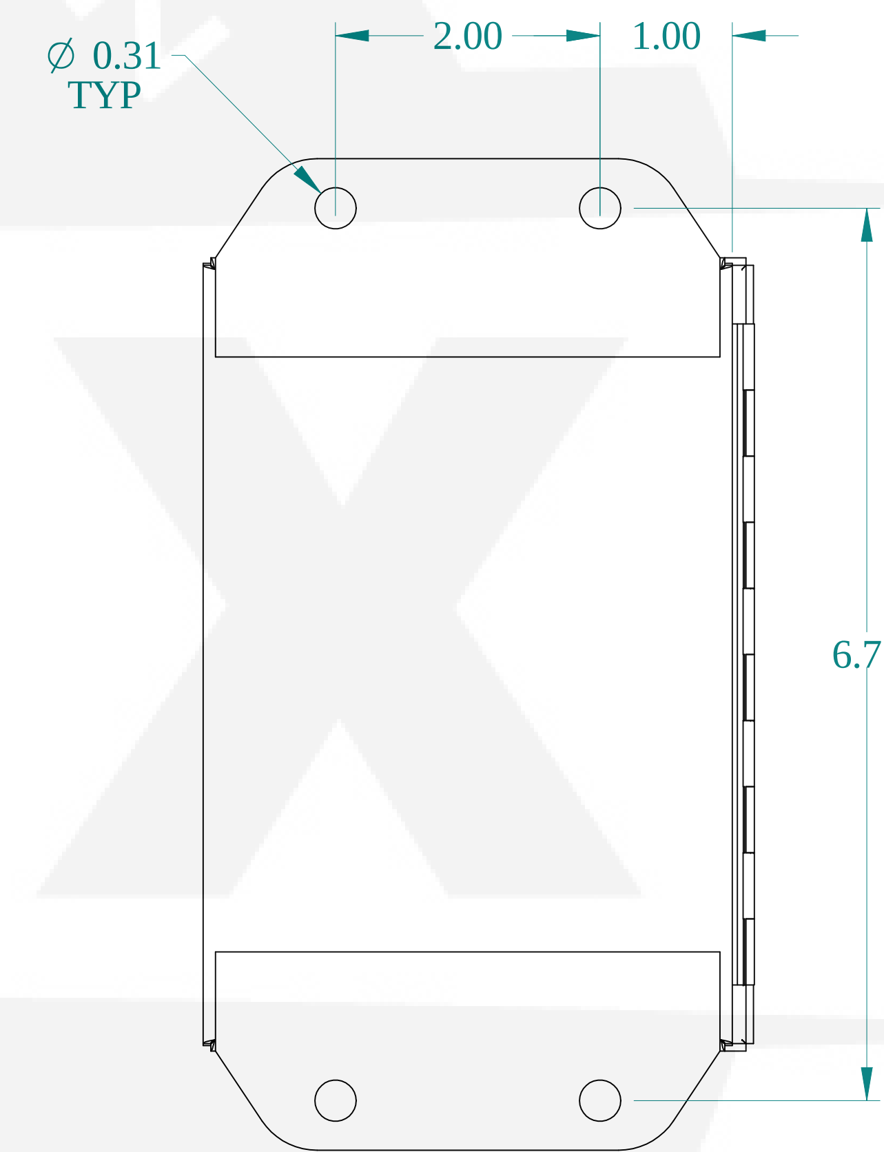
BACK VIEW
