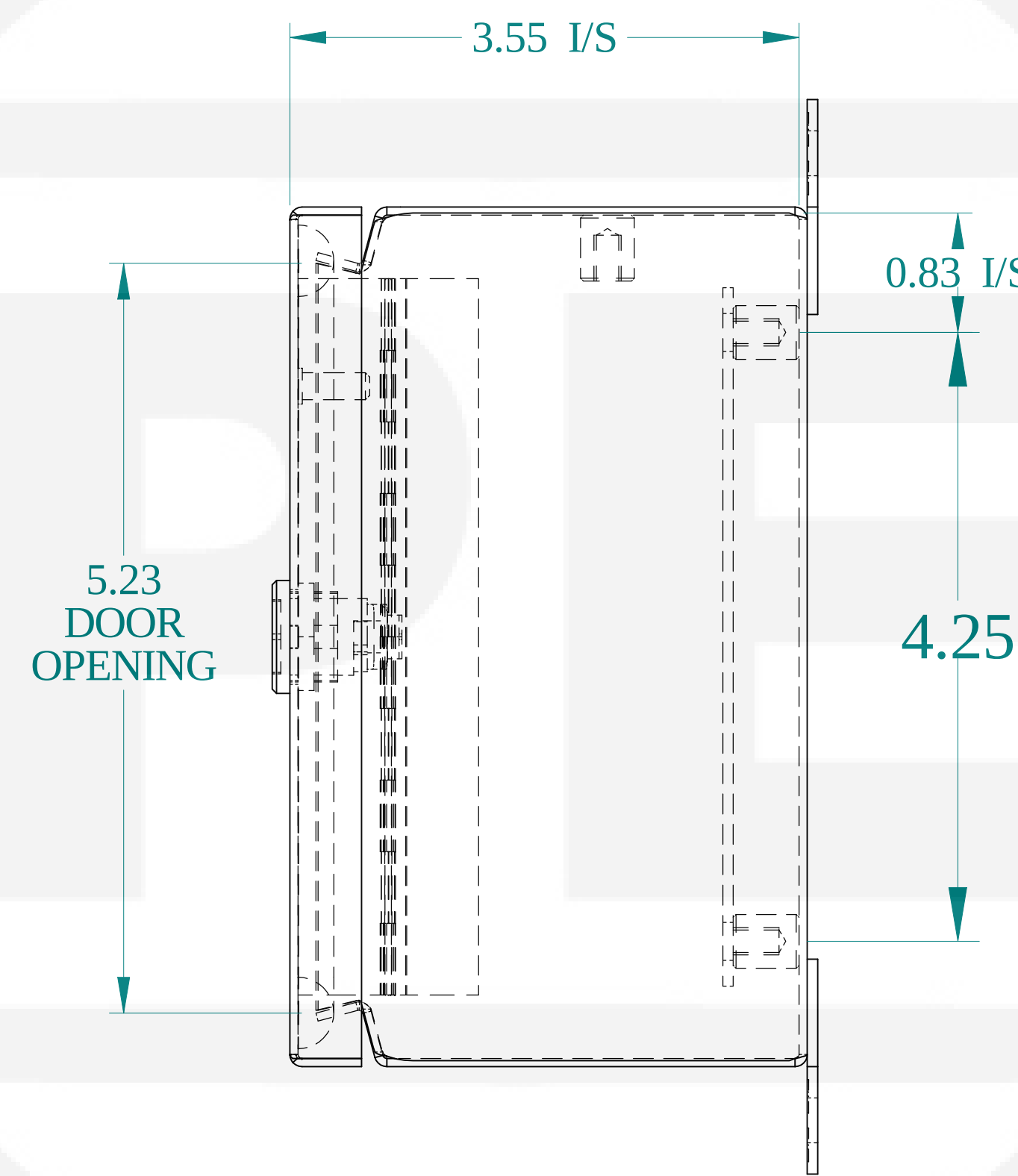
SIDE VIEW
